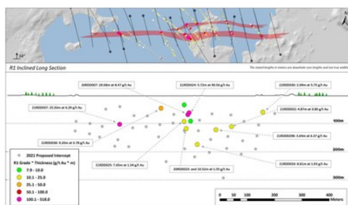
Long Section of Proposed Drilling along R1 Structure (CNW Group/Kenorland Minerals Ltd.)
