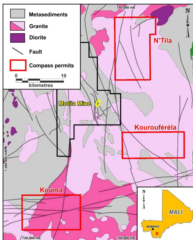
Figure 5 - Location of the Morila block permits with respect to the Morila mine.
