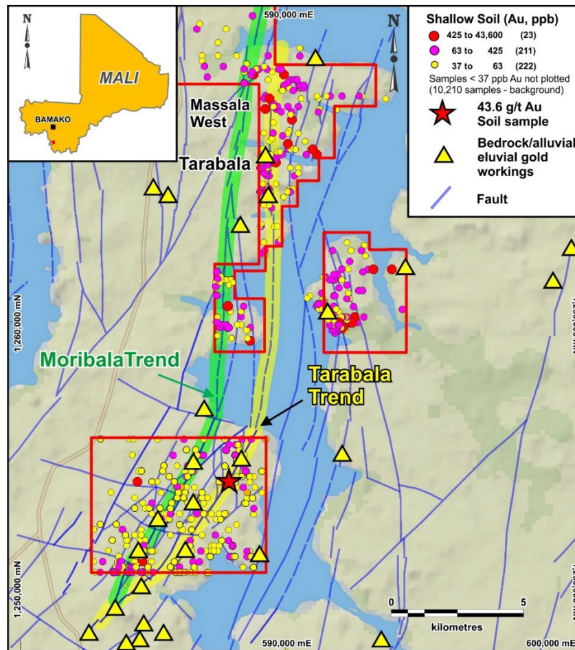
Figure 4 - Location of the Moribala permit with respect to the Tarabala and Moribala Trend.
