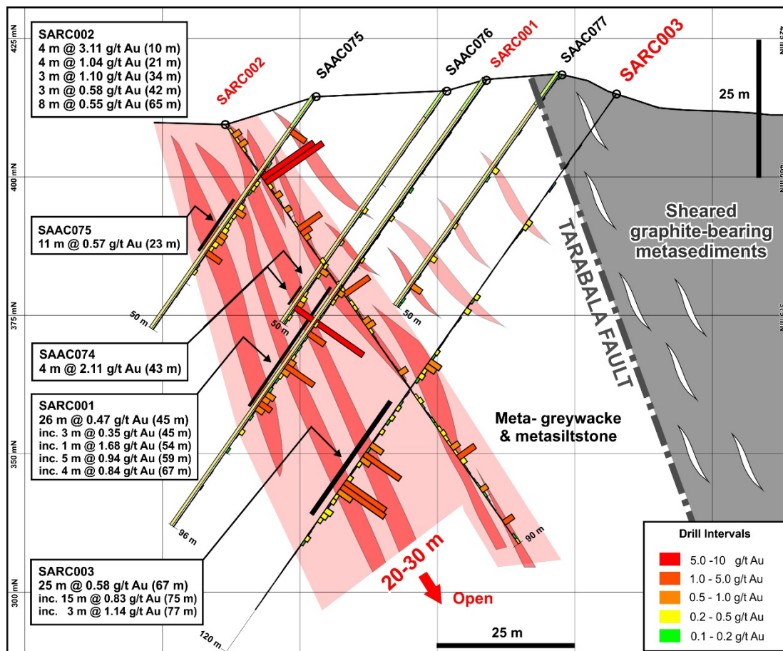
Figure 9: Cross section through the main workings at Tarabala.
