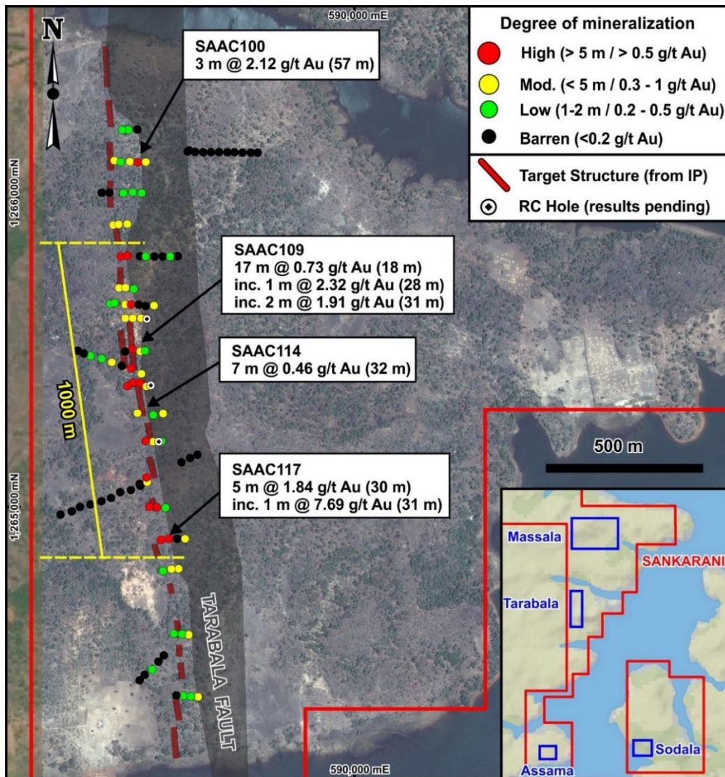
Figure 7: Drilling locations and significant results at Tarabala for the latest drilling.
