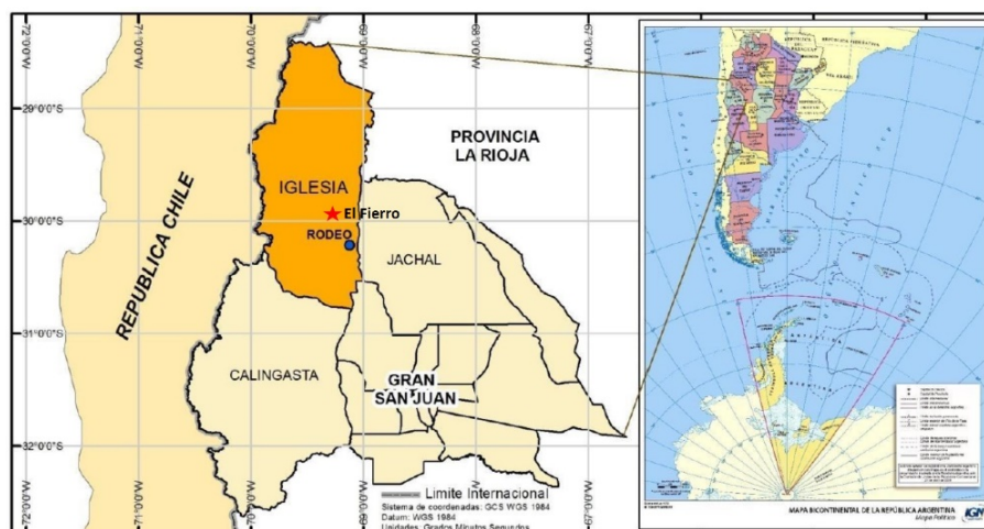
Location of El Fierro Project
