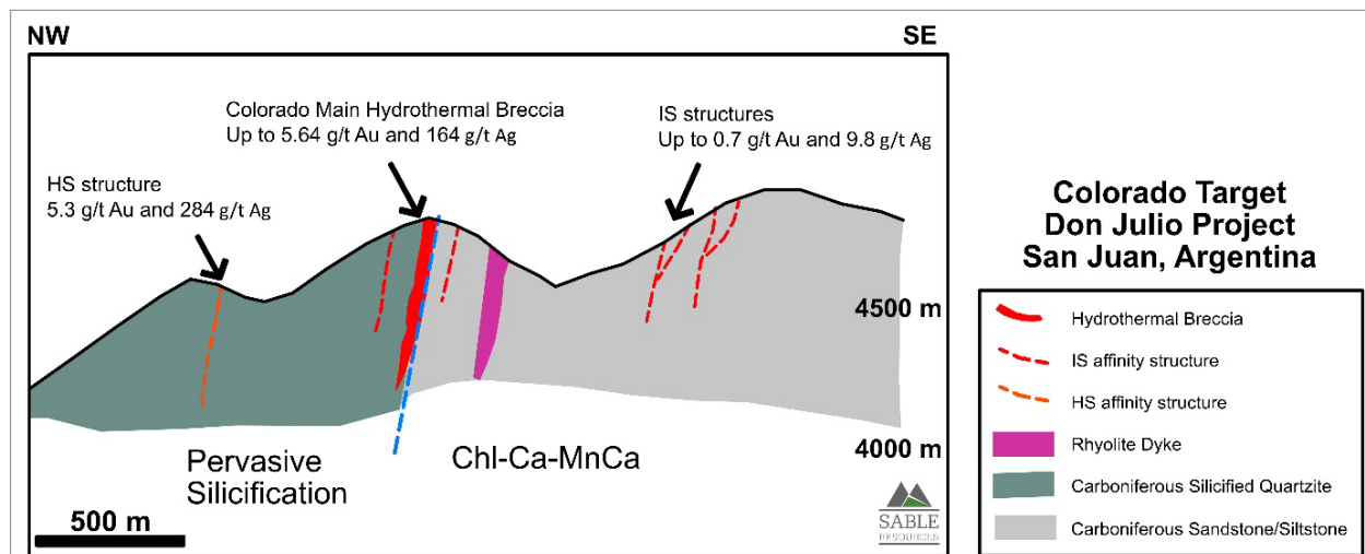
Conceptual section of the Colorado target
