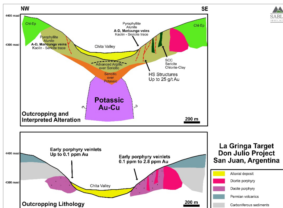
Conceptual section of the La Gringa target
