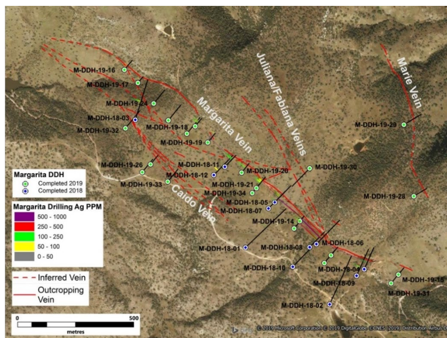
Mineralized Structures and Distribution of 2018-2019 Drill Holes at Margarita Project
