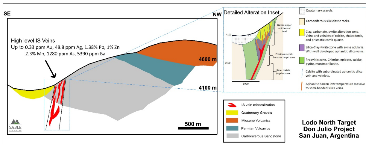
Conceptual section of the Lodo North target
