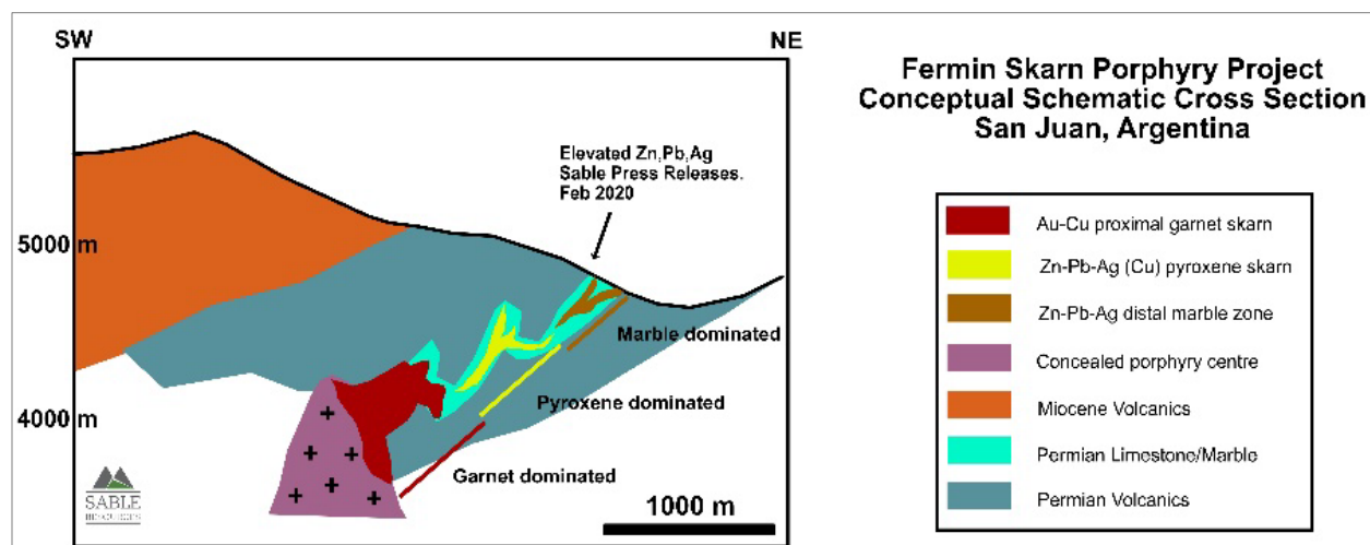
Conceptual Section of the Fermin target
