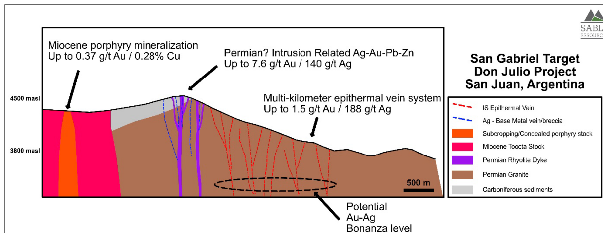
Conceptual section of the San Gabriel target
