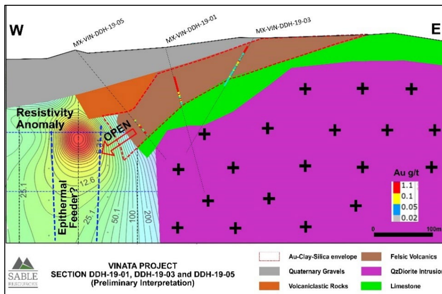
Preliminary Interpretation of geology at Vinata North
