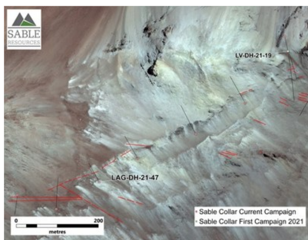
Figure 2. Location of drill hole LAG-DH-21-47 (CNW Group/Sable Resources Ltd.)
