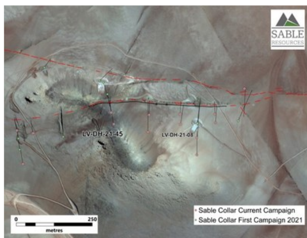
Figure 1. Location of drill hole LV-DH-21-45 (CNW Group/Sable Resources Ltd.)
