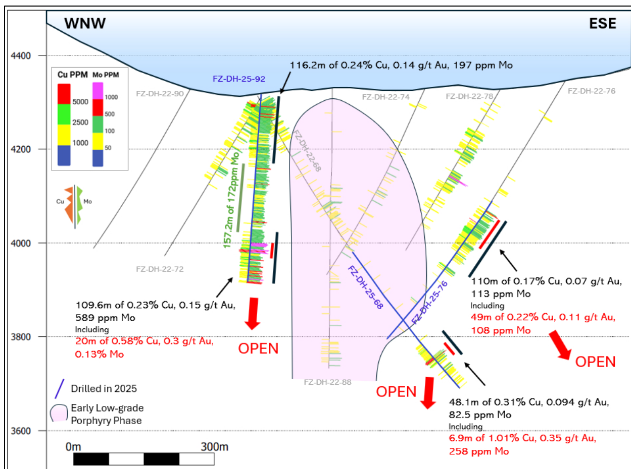
Figure 4. Schematic section of the Pyros porphyry along the main drill fence showing the mineralized intervals in holes FZ-DH-25-92, FZ-DH-25-68, and hole FZ-DH-25-76.
