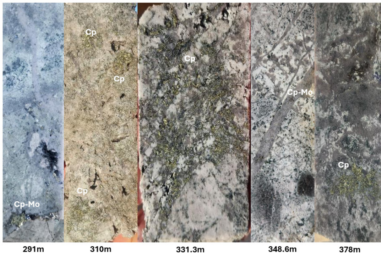
Figure 2. Examples of mineralization observed in hole FZ-DH-25-92. Cp: chalcopyrite; Mo: molybdenite. HQ core (63.5mm)
