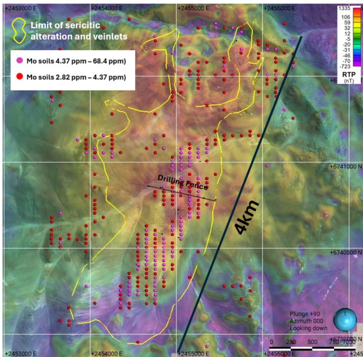
Figure 1. Location of the drill section presented in Figure 4 with respect to the footprint of the Pyros system showing the extension of the sericitic alteration, magnetic anomaly and molybdenum highest anomalies from 2022 soil sampling. The map clearly shows the potential to extend the intercepted Cu-Au-Mo mineralization along strike
