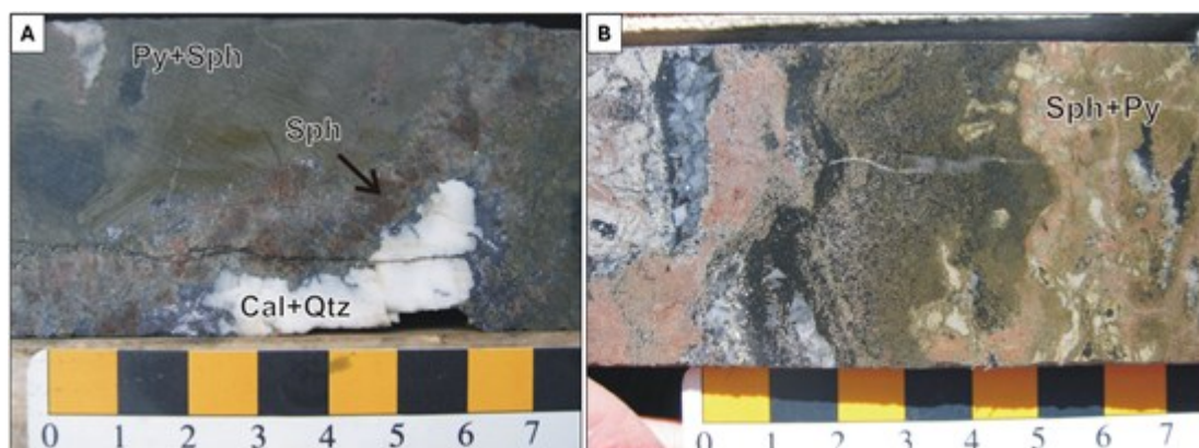
Figure 1. Photographs of Stratabound Massive Sulfide (SMS) mineralization at Prairie Creek, which is now understood to contain high-grade germanium. A) Fine-grained massive aggregate of pyrite (Py) with lesser sphalerite (Sph) crosscut by a vein of coarse-grained red sphalerite. The remaining cavities in the vein are filled first by galena and second by sparry calcite (Cal) and quartz (Qtz). B) Banded sulfides showing broadly defined bands rich in sphalerite and others rich in pyrite. Source: Paradis (2007). (4)
