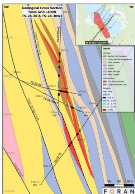
Figure 4 – Geological cross section through the Tesla Zone, highlighting the relationship of drill holes TS-24-30 and TS-24-30w1 relative to the previous drilling in the area. (CNW Group/Foran Mining Corporation)
