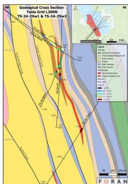
Figure 5 – Geological cross section through the Tesla Zone, highlighting the copper-dominant mineralization intersected in TS-24-29. (CNW Group/Foran Mining Corporation)
