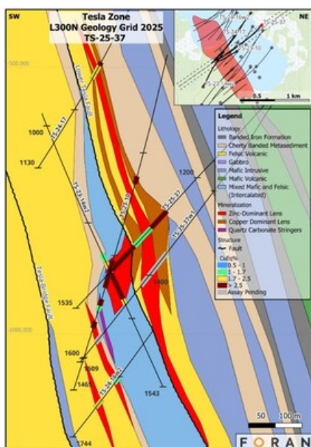
Figure 4 – Cross section along Line 300N through the Tesla Zone, showing the relationship between drill holes TS-25-37, TS-25-37w1, TS-23-10 and TS-2314w2 (CNW Group/Foran Mining Corporation)
