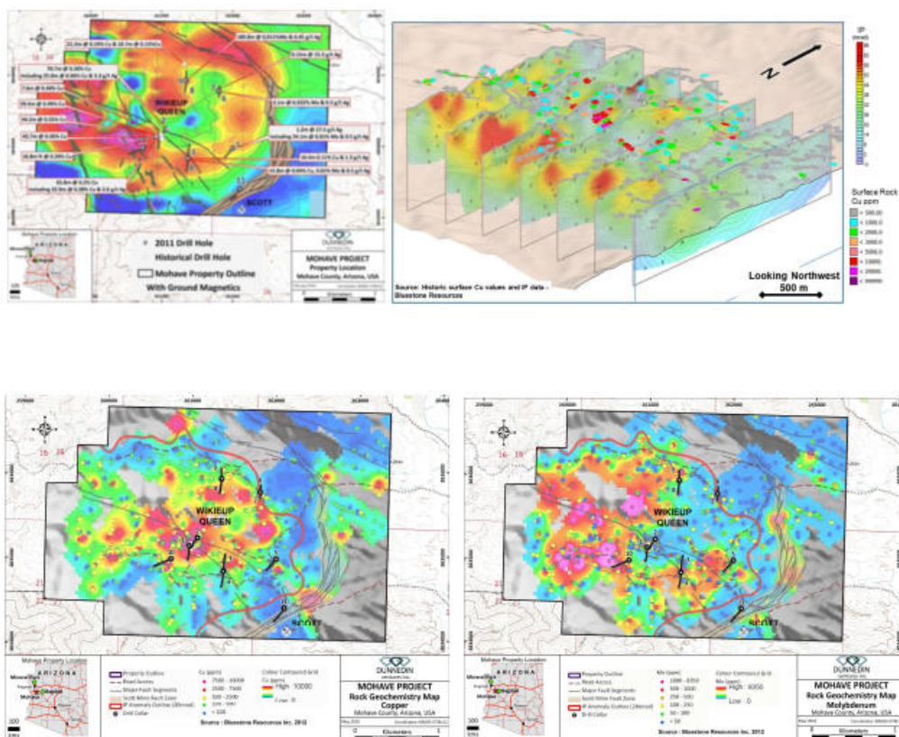
Figures 2 - Ground magnetics, IP sections, copper geochemistry and molybdenum geochemistry
