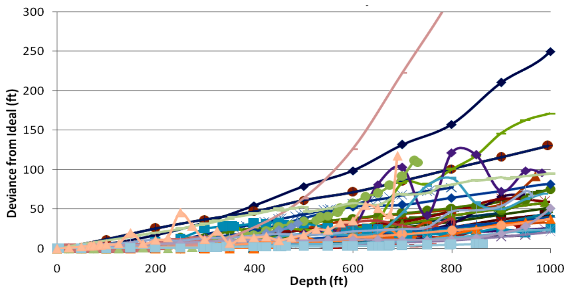
Figure 12.8. Drift deviation per core drill hole versus depth
