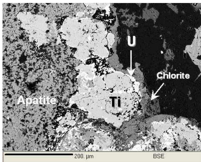
Figure 7.2. Microprobe, backscatter electrons: Titanium oxides are rimmed and impregnated by Uranium and associated with apatite and chlorite (S-603, 282.3 to 283.0 feet).
