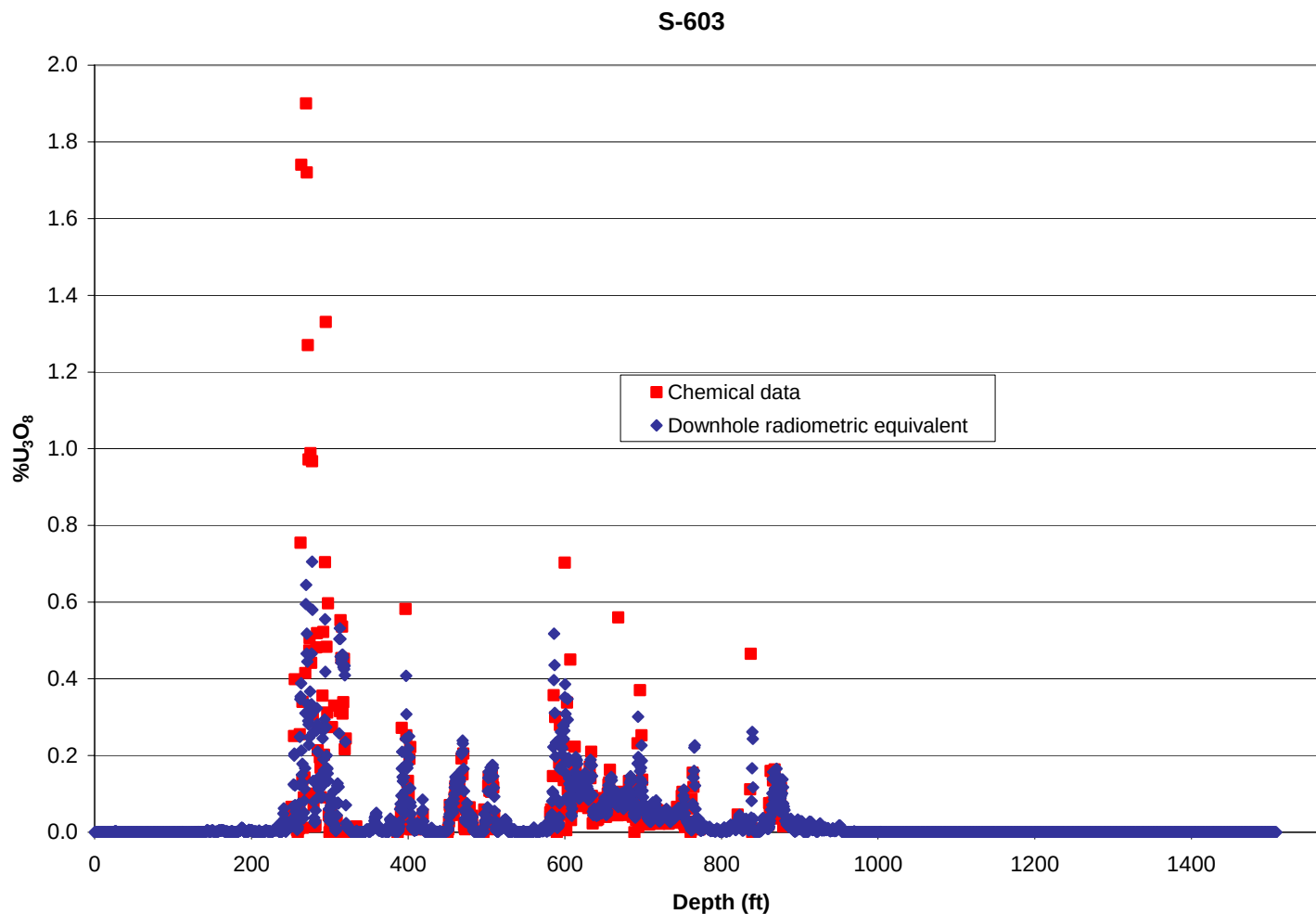
Figure 12.3. Chemical assays for drill hole S-603 from Energy Labs and radiometric equivalent from MM&A
