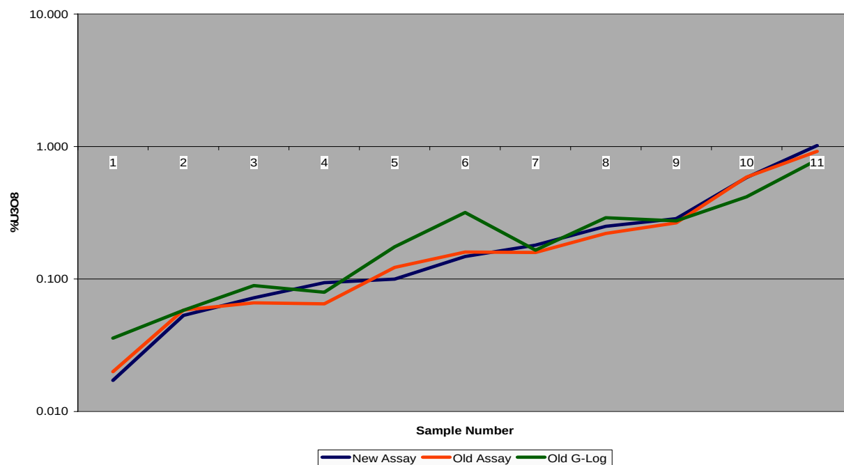
Figure 12.6. Assay and gamma log comparison for selected Marline drill holes
