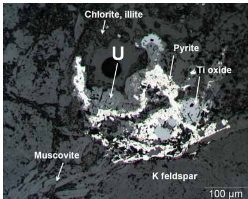
Figure 7.1. Reflected light : Uranium minerals are developed on pyrite and titanium oxide, and associated with chlorite.(S-602, 505 to 508 feet).
