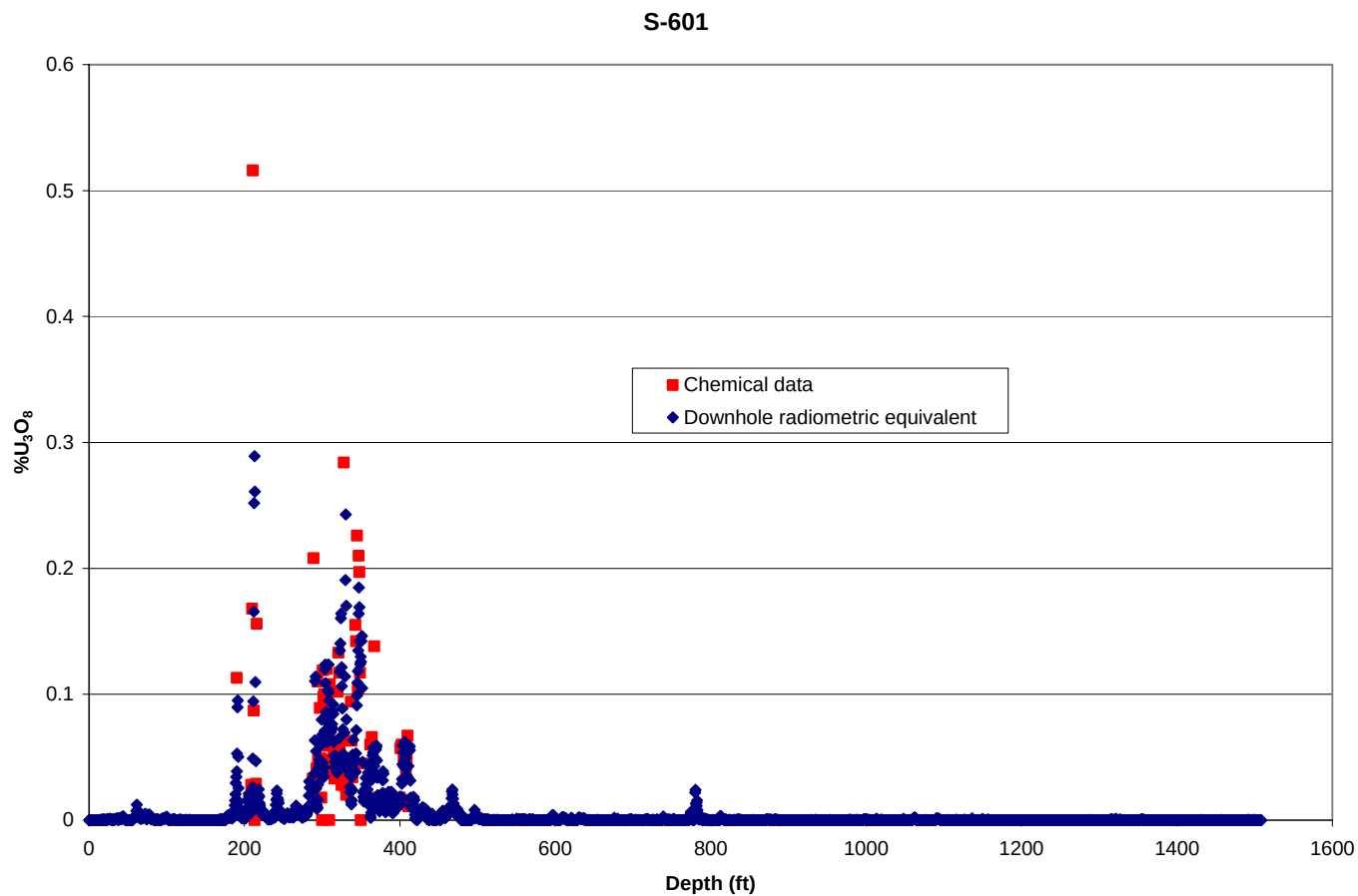
Figure 12.1. Chemical assays for drill hole S-601 from Energy Labs and radiometric equivalent from MM&A
