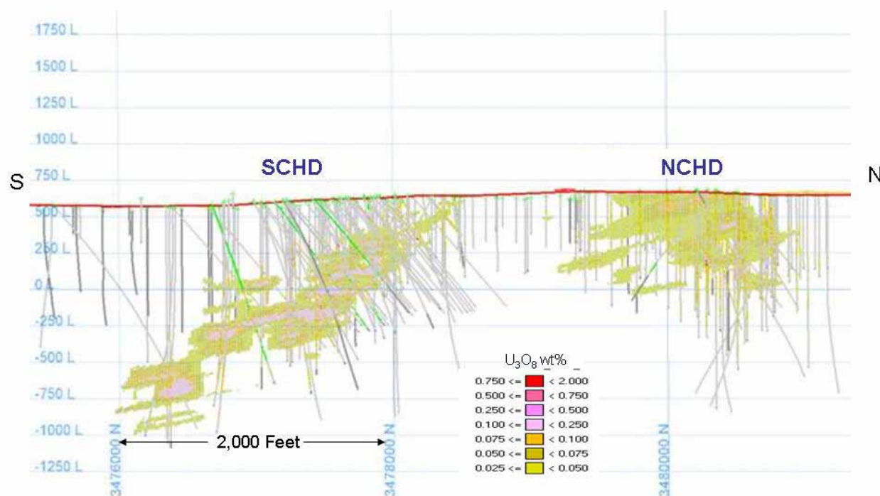
Figure 15.3. Vertical cross-section with 2-D view of block grade estimations, looking west. Grade intervals are wt % U_3O_8 . Line of cross-section shown in Figure 15.1
