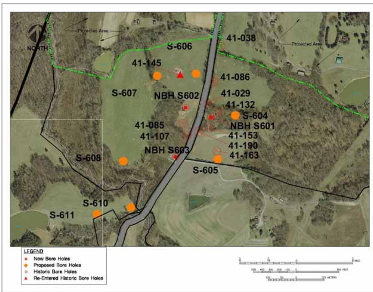
Figure 9.1. Drill hole locations, South Coles Hill Deposit (SCHD)
