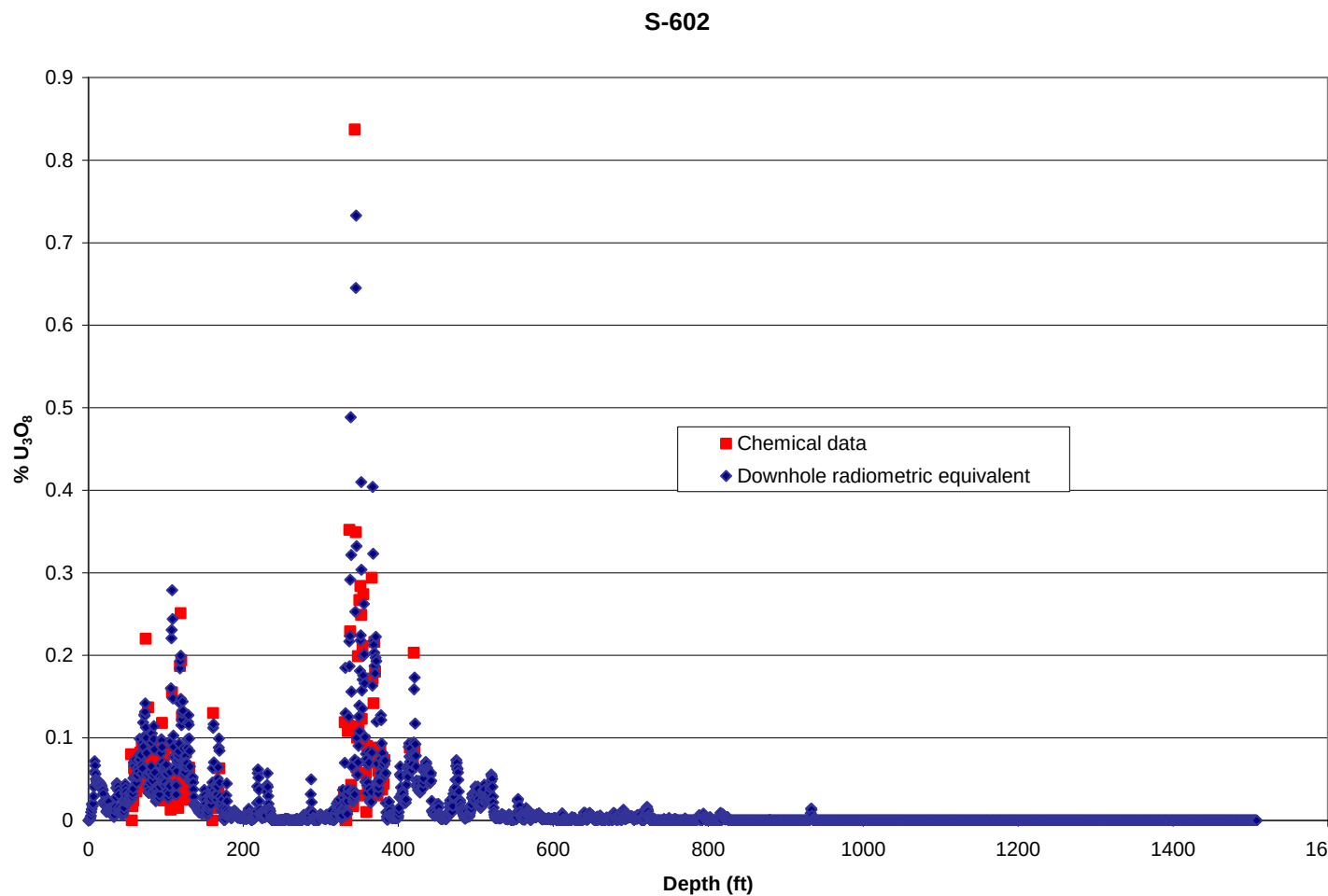
Figure 12.2. Chemical assays for drill hole S-602 from Energy Labs and radiometric equivalent from MM&A
