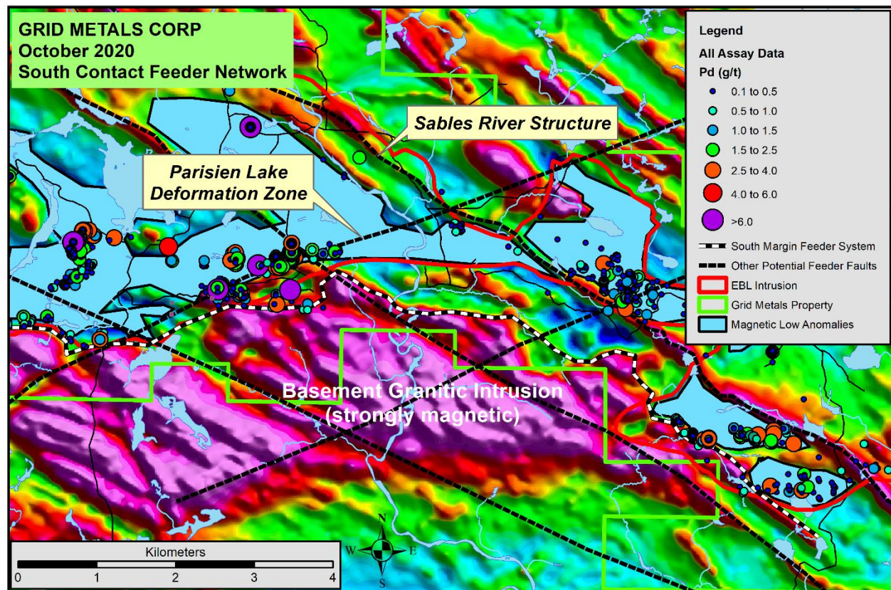
Figure 2. Interpreted feeder structures and corresponding magnetic low anomalies on a background total magnetic intensity image. Also shown are historical and recent core and surface sample locations with symbols coded to palladium grade.
