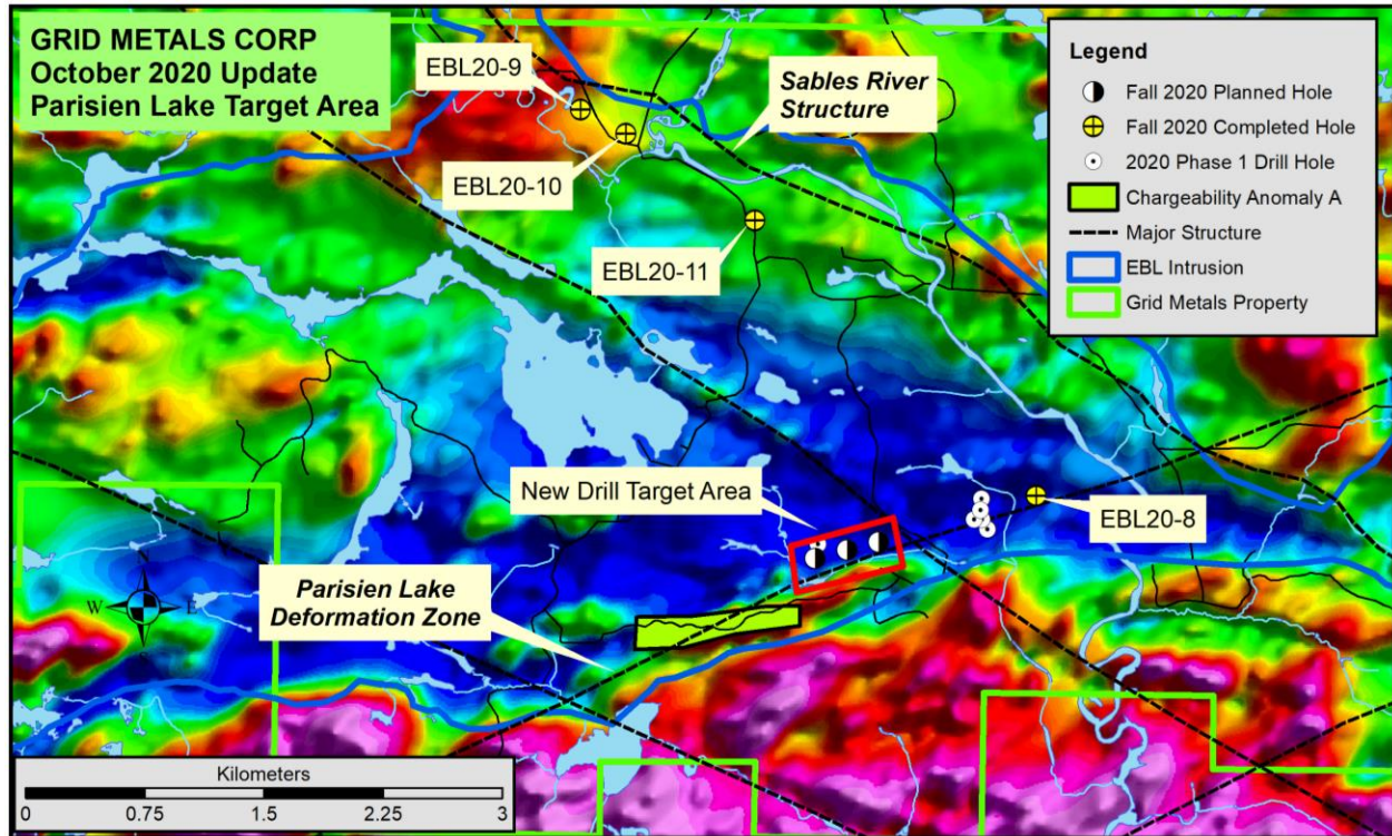
Figure 1. Completed 2020 Grid Metals drill holes in the west lobe of the East Bull Lake intrusion on total magnetic intensity background image. Also shown are the preliminary locations of three proposed holes in the Parisien Lake area targeting a coincident magnetic low anomaly and Pd- and base metal-rich surface mineralization.
