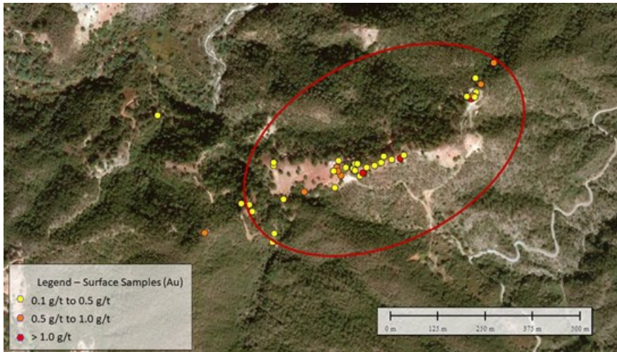
Figure 2 - Gold Results from Surface Rock Sampling at Gold Ridge
