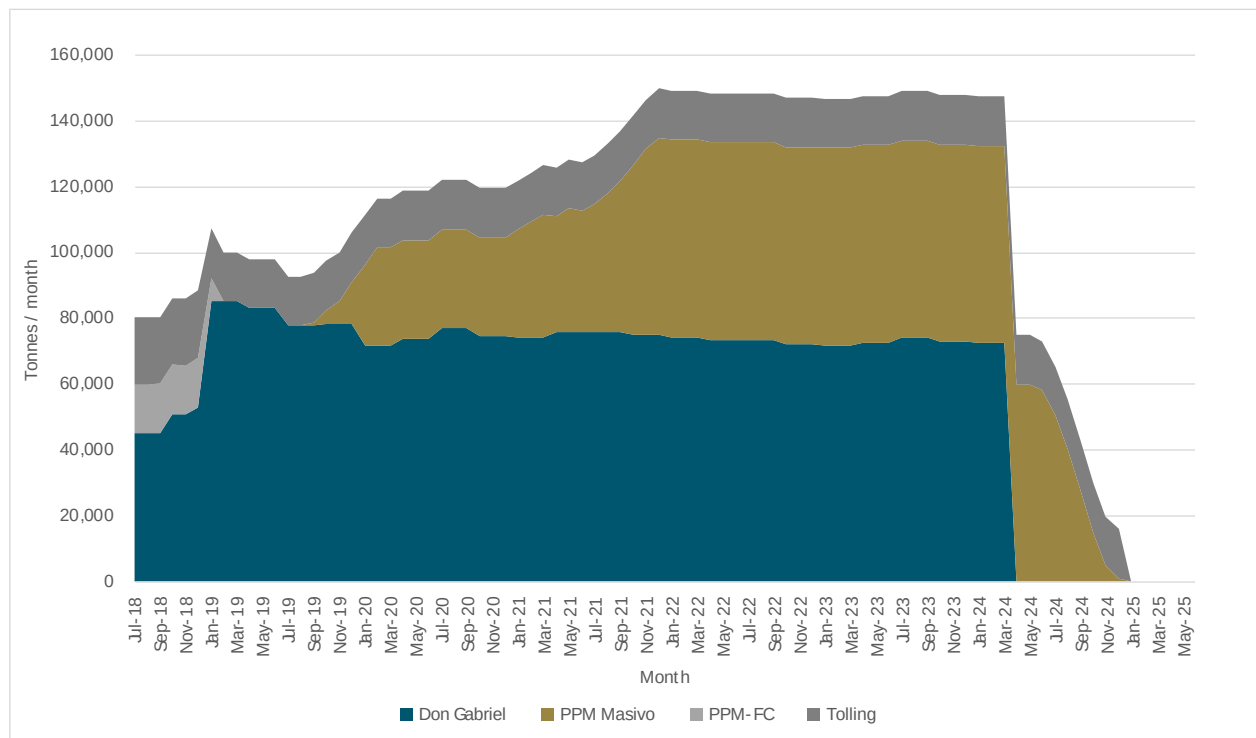
Figure 1. Base Case Forecast Mine and Process Plan
