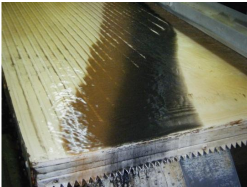
Wet table separation of HM from Thunderbird bulk sample
