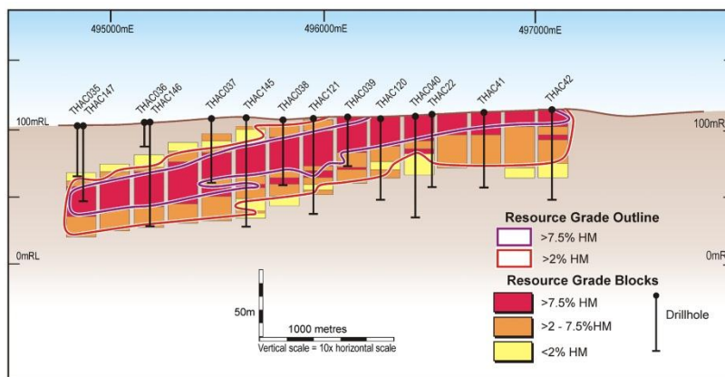
Cross section through Thunderbird HMS deposit
