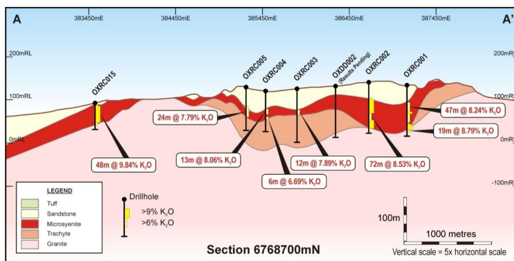
Drill Section through Oxley potash project
