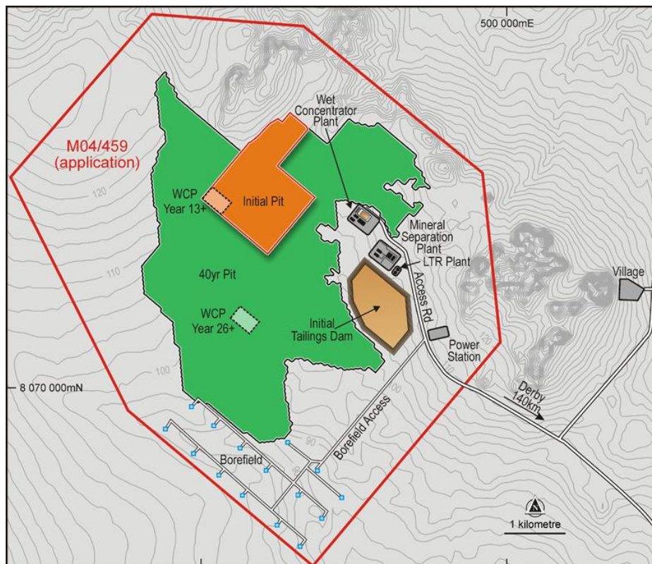
Figure 3: Thunderbird Site Layout Plan
