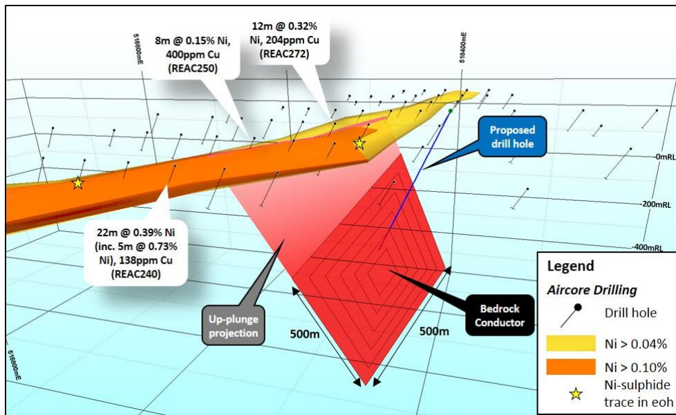
Figure 9: Stud prospect showing modelled bedrock conductor beneath extensive nickel geochemical anomalism in shallow aircore drill holes
