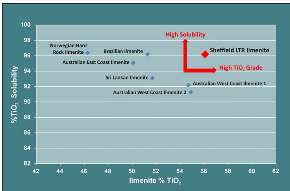
Figure 5: %TiO 2 Solubility vs Grade, Sheffield LTR Ilmenite benchmarked against known sulphate Ilmenites (blue)
