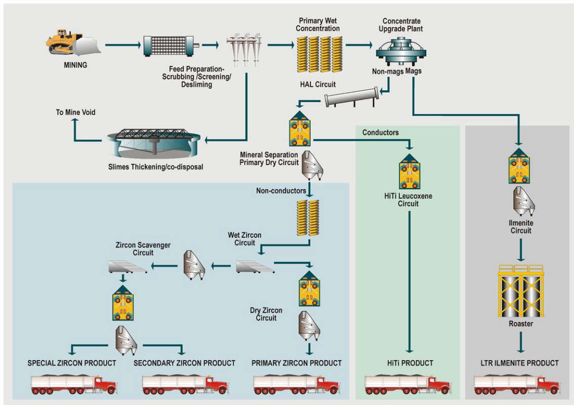
Figure 4: Thunderbird Schematic Process Flow Sheet
