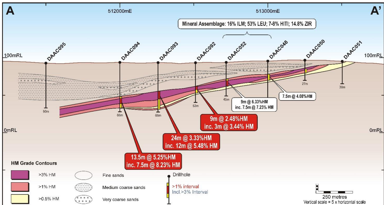
Figure 7: Night Train prospect cross-section
