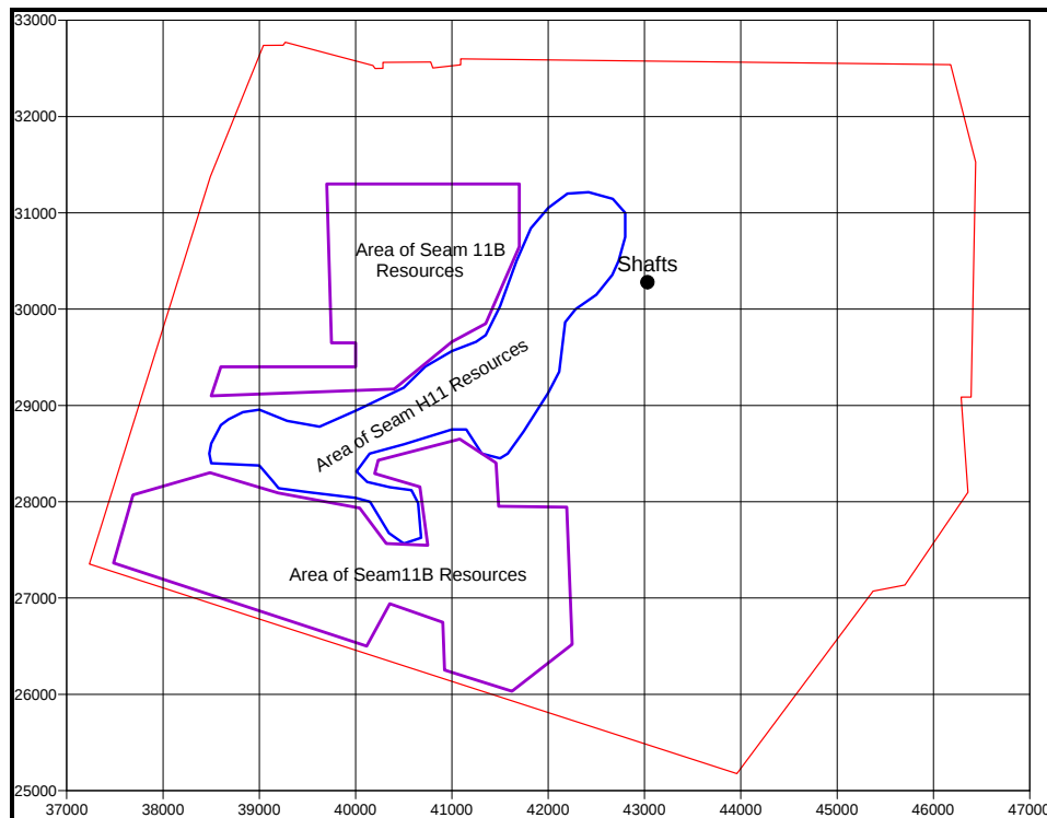
Figure 19-1 Resource Areas, Seams H 11 and H 11 B , Verticalnaya Mine
