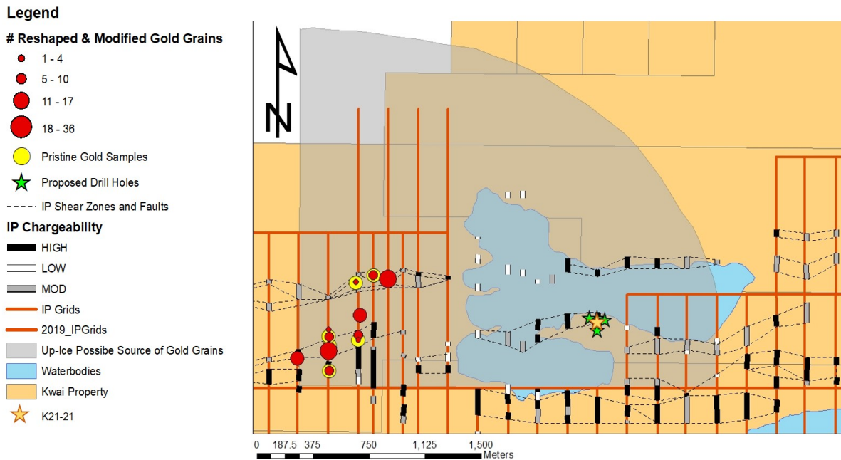
Figure 3 Gold Grains Probable Source Area Plot For the West Grid
