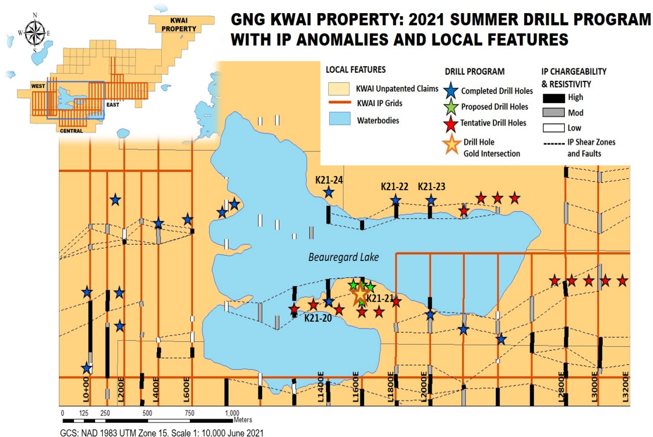
Figure 2 IP anomalies and drill holes at Beauregard Lake
