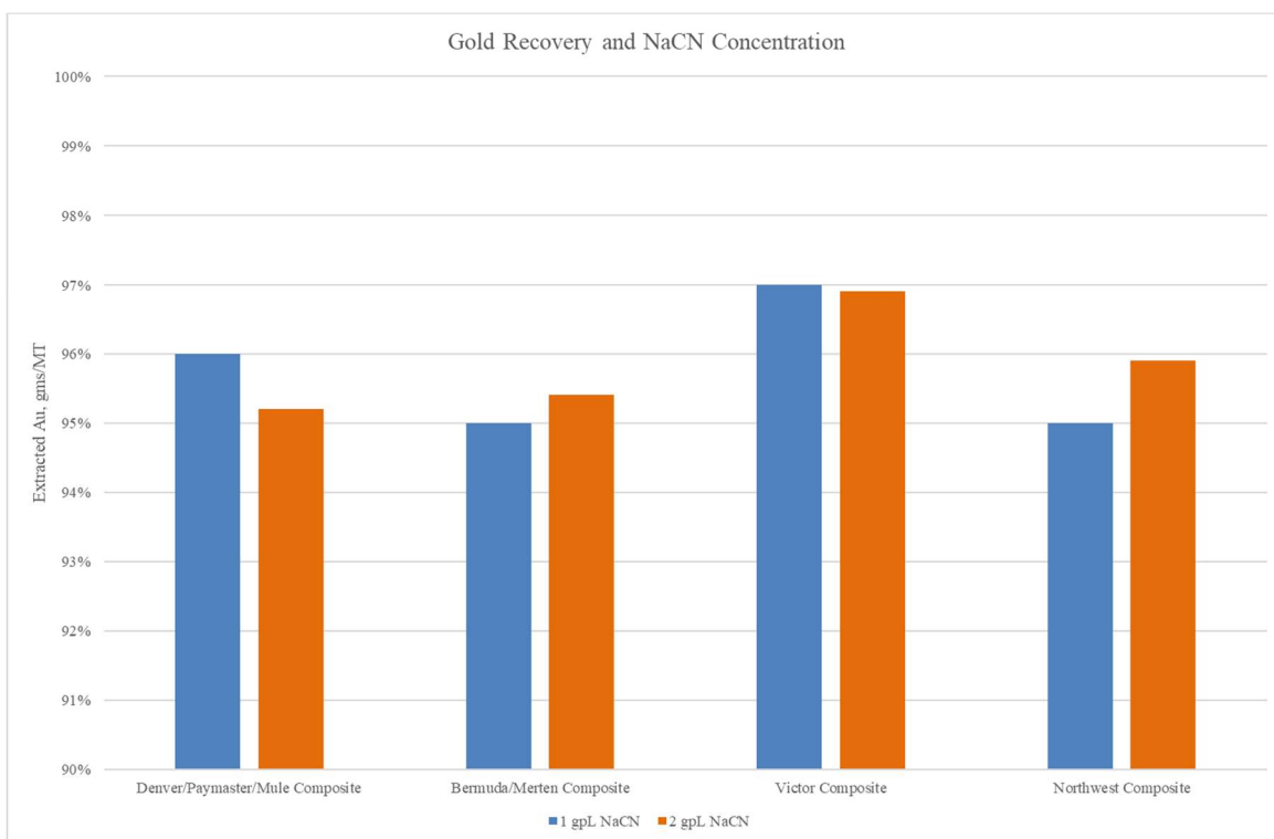
Figure 13-5 Gold Recovery vs. NaCN Concentration
