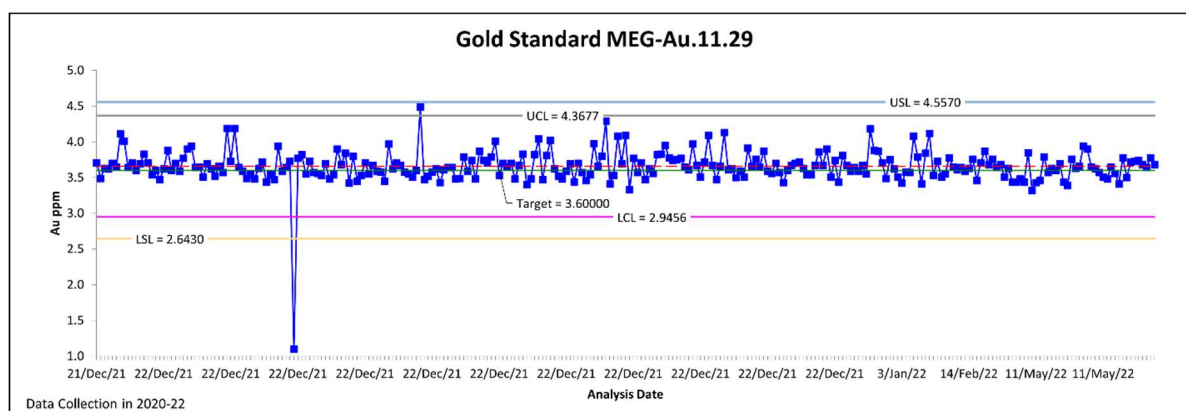
Figure 11-5 Control Chart for Gold CRM MEG-Au.11.29
