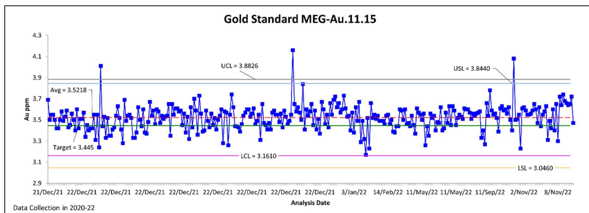
Figure 11-4 Control Chart for CRM MEG-Au.11.15
