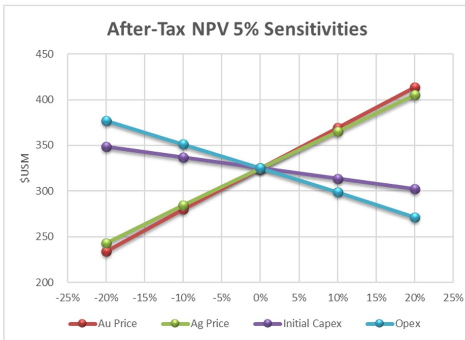
Figure 22-2 After-Tax NPV @ 5%
