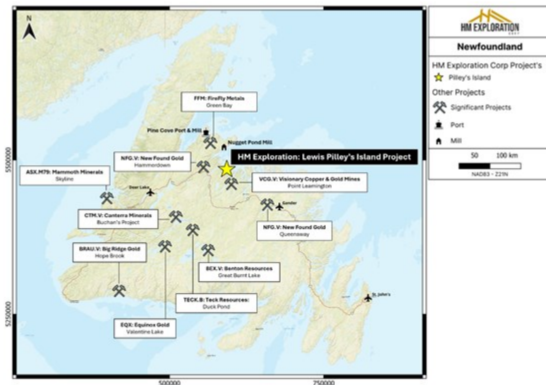
Figure 3: Regional map of Newfoundland displaying the location of the Project and other significant mineral exploration and mining projects in Newfoundland - Canada.
