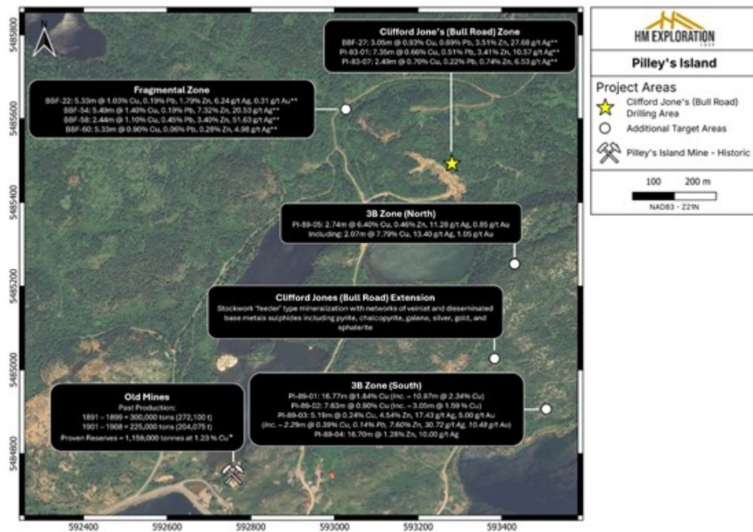
Figure 2: Location map of the Project displaying historical showings/zones located on the Project. 2026 diamond drilling has commenced at the Zone.
