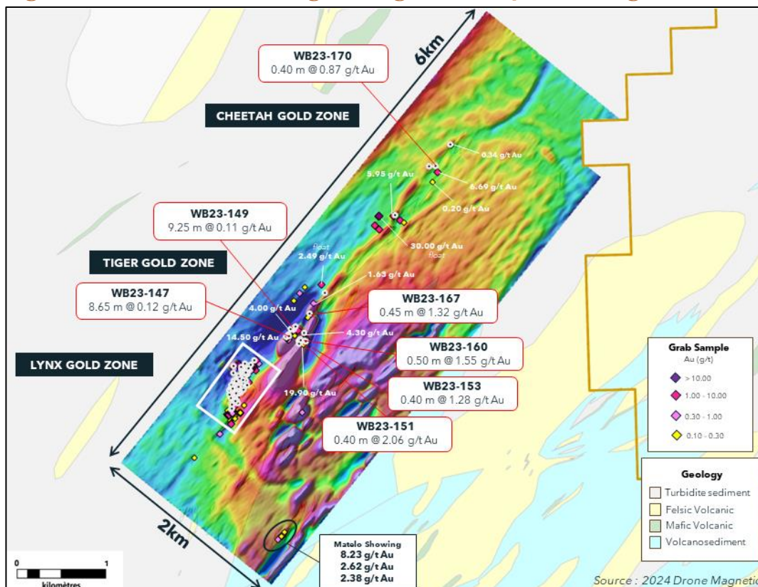
Figure 1. Location of scouting drilling over 2024 drone magnetic survey map
