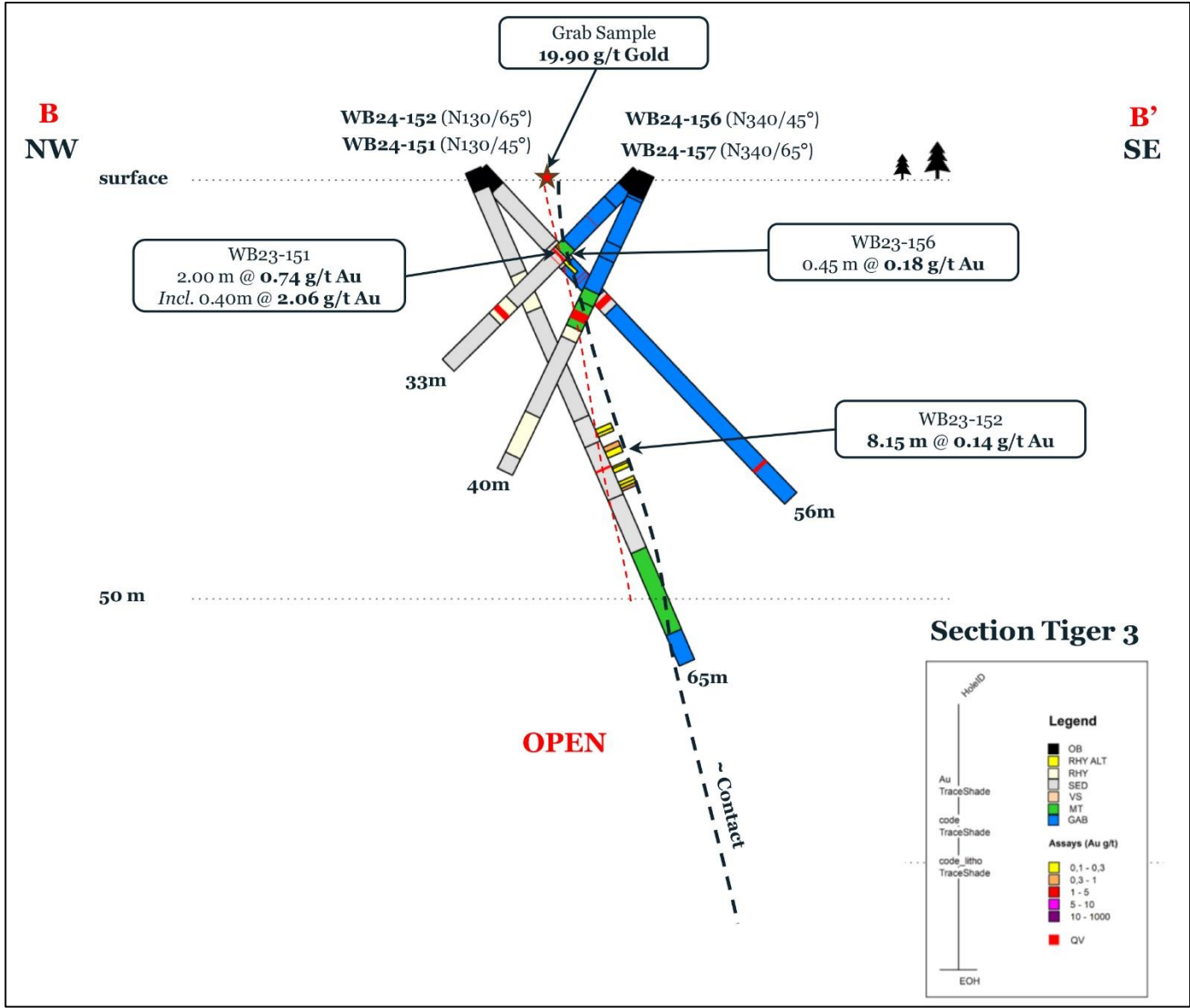
Figure 5. Drill section at Tiger 3
