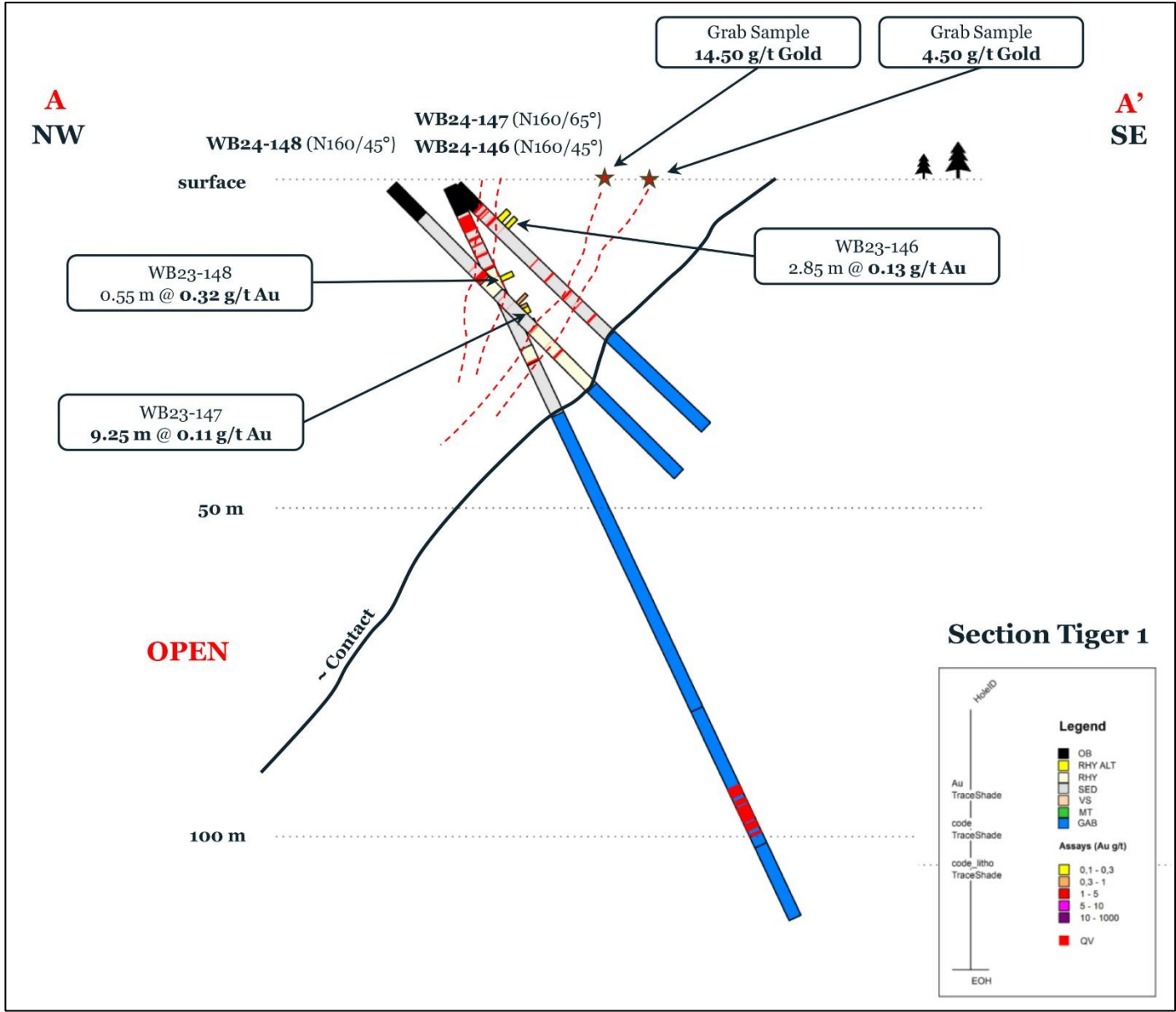
Figure 4. Drill section at Tiger 1
