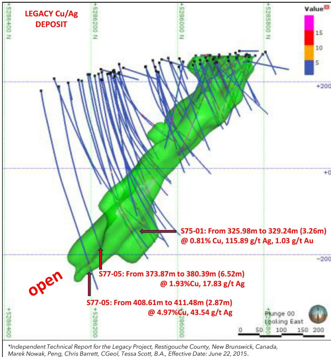
Figure 2. 3D model of the Legacy Deposit from historic resource estimate*
