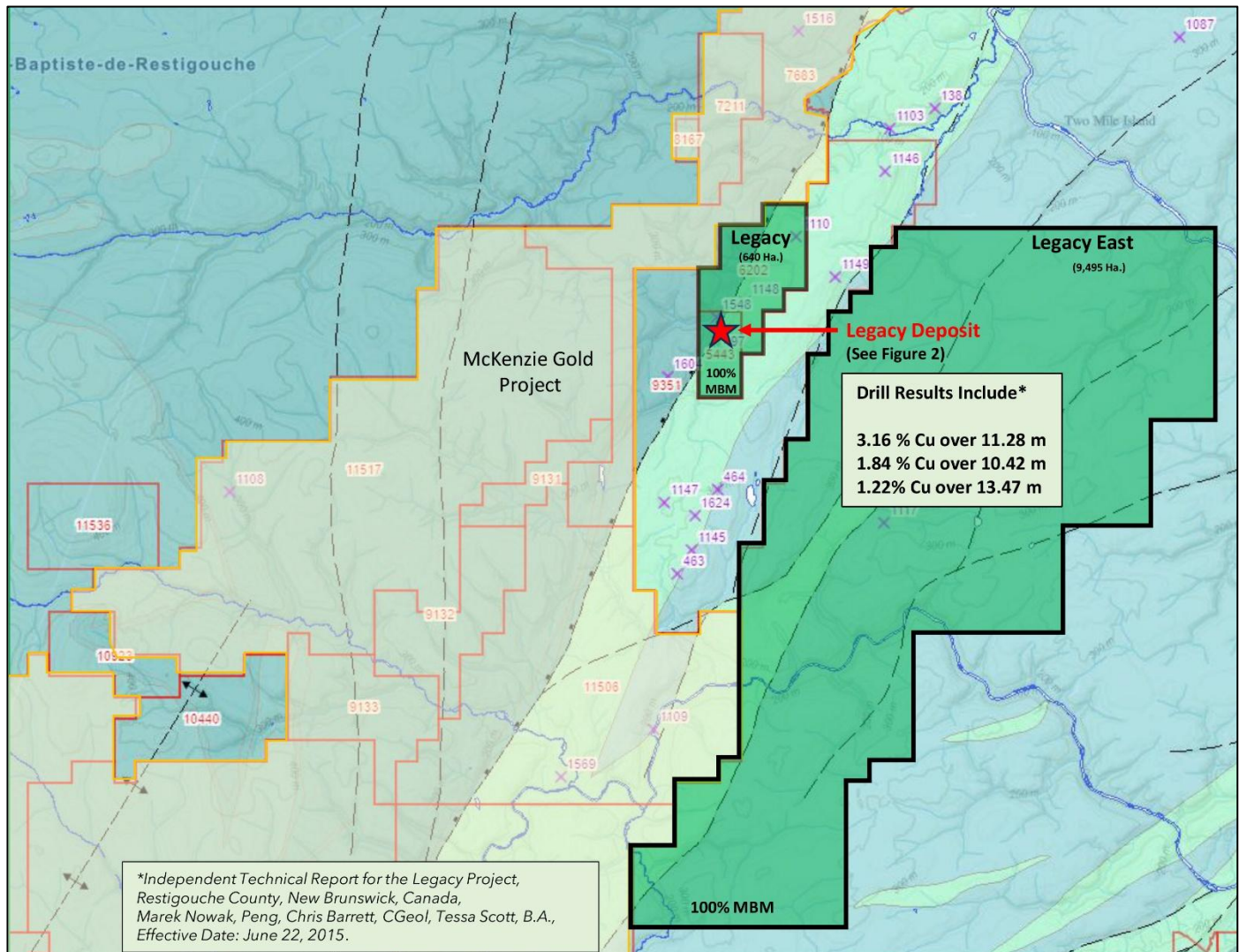
Figure 1. Location of the Legacy Project
