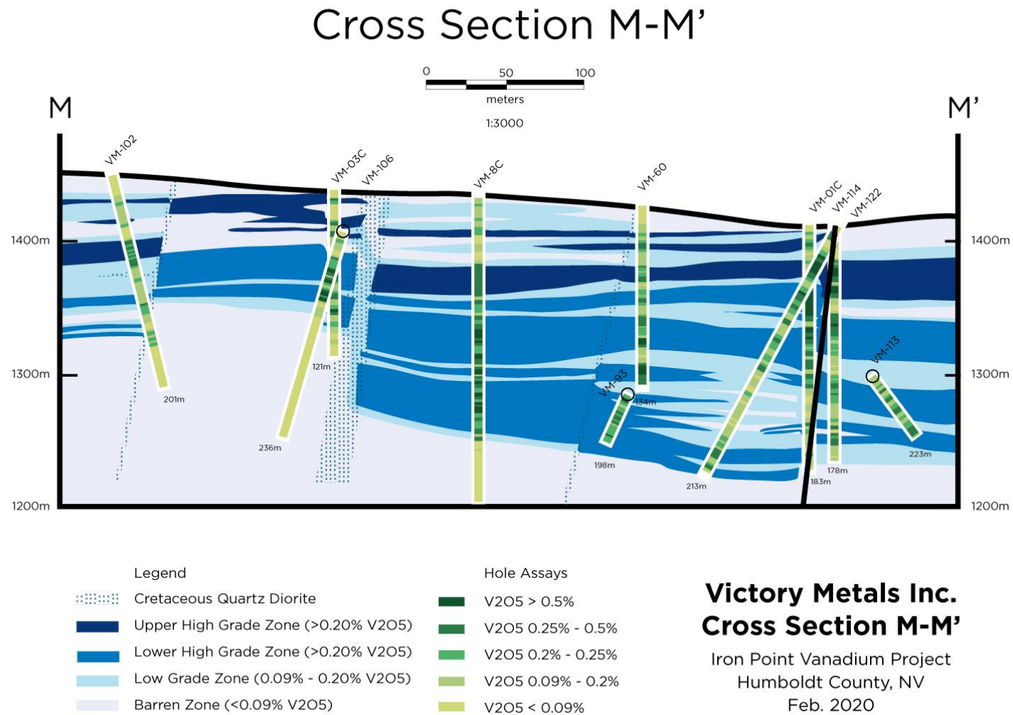
Figure 3. Cross section M-M' showing distribution of vanadium mineralization in relation to the current geologic interpretation.
