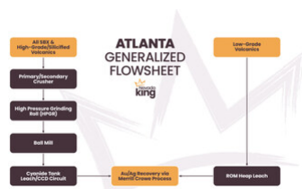
Figure 1. Revised Atlanta generalized flowsheet after Phase 2 metallurgical testing (CNW Group/Nevada King Gold Corp.)
