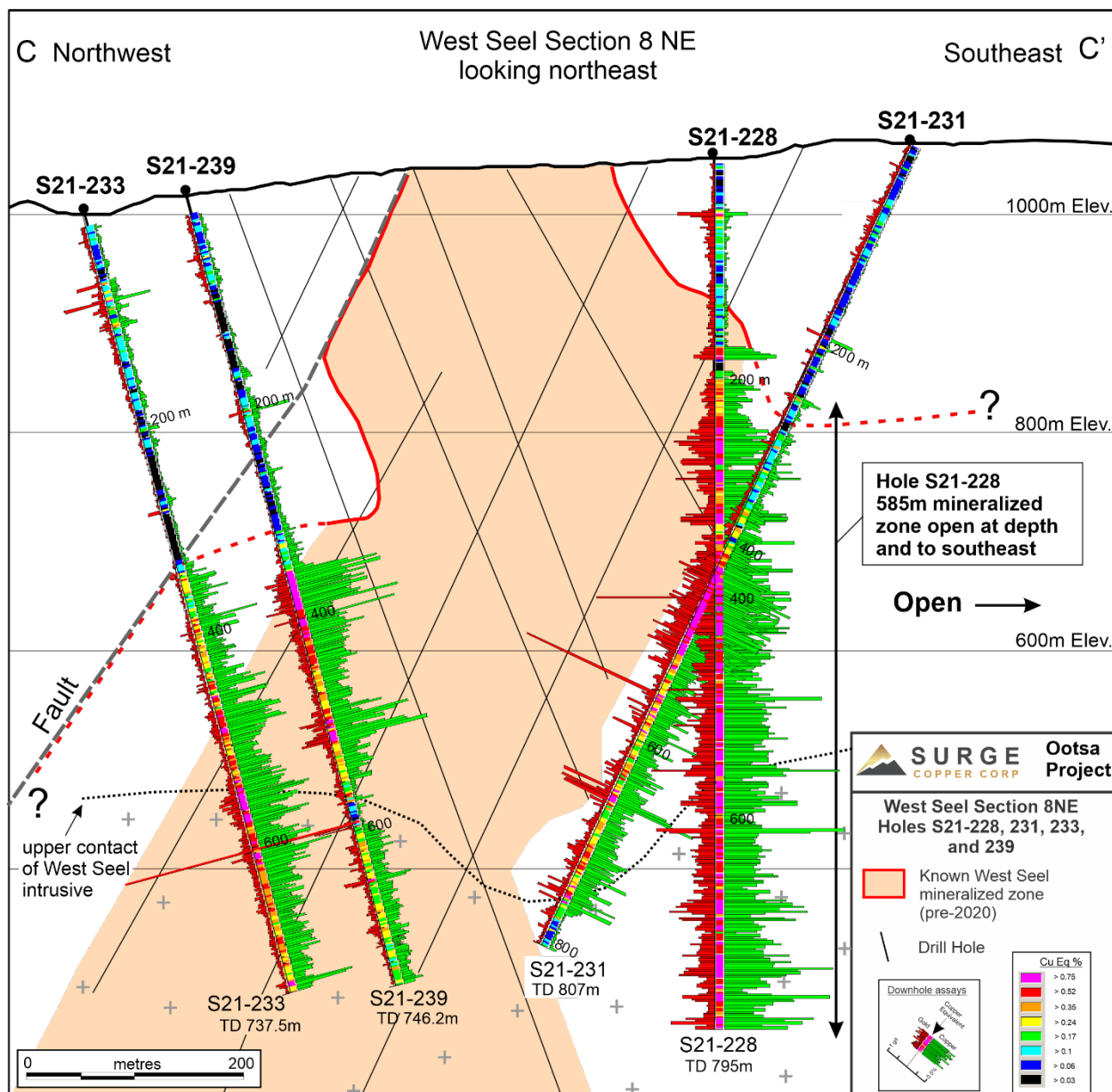
Figure 2. West Seel Cross Section C-C' showing results for holes S21-228, 231, 233, and 239. See Figure 1 for section location.
