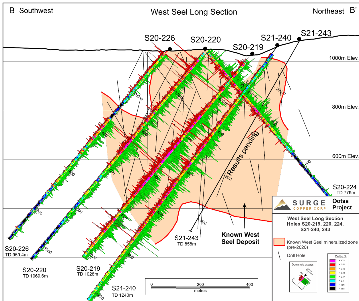
Figure 4. West Seel long section B-B' showing results for holes S20-219, 220, 224, and 226, and S21-240. See Figure 1 for section location.
