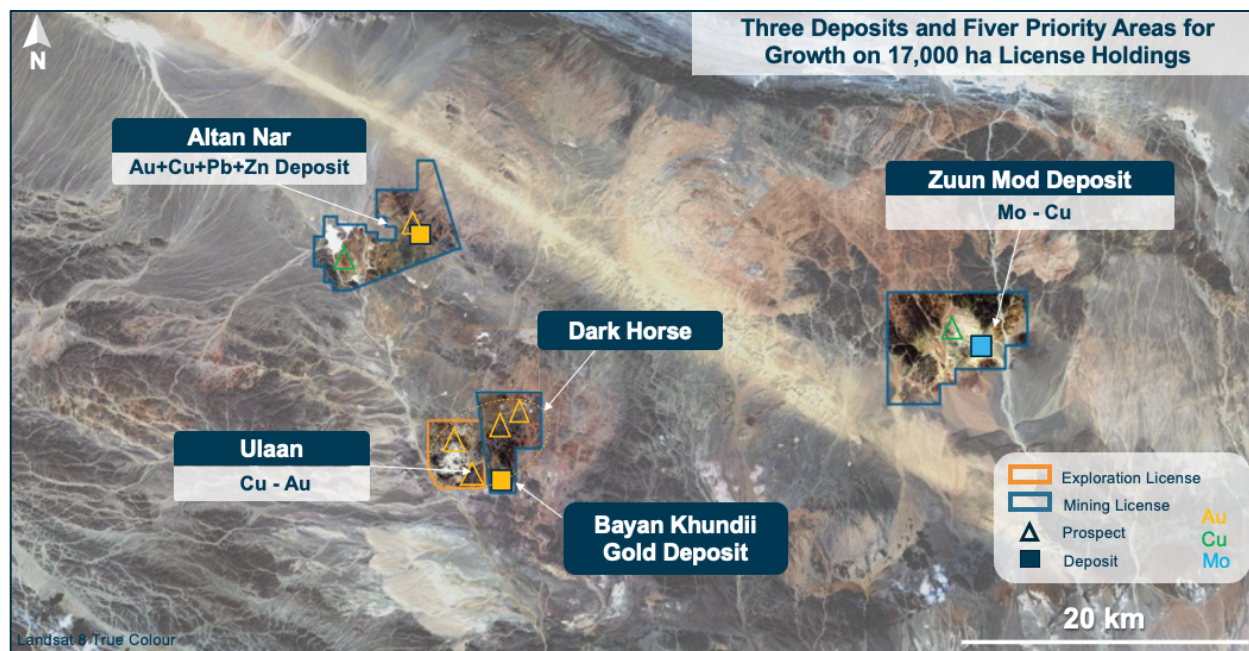
Figure 2: Gold, Copper & Molybdenum Deposits and Prospects – Khundii Minerals District
