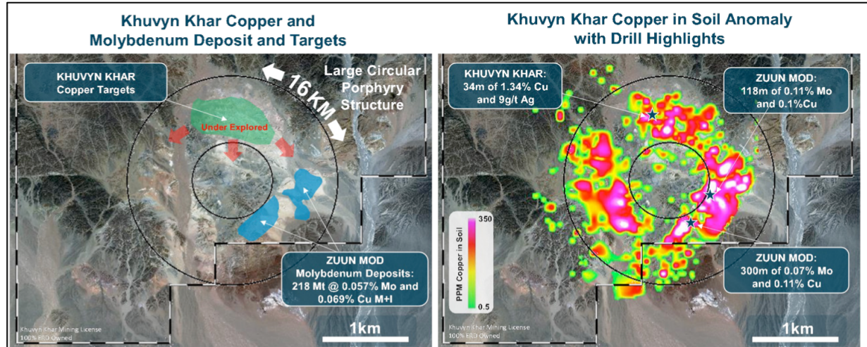
Figure 3: Khuvyn Khar Porphyry Complex – Zuun Mod Deposit
