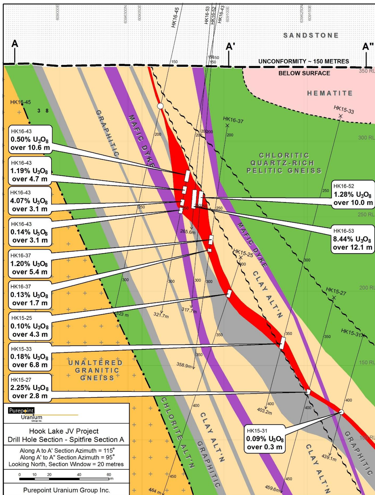
Figure 9: Geologic Section of the Spitfire Uranium Deposit
