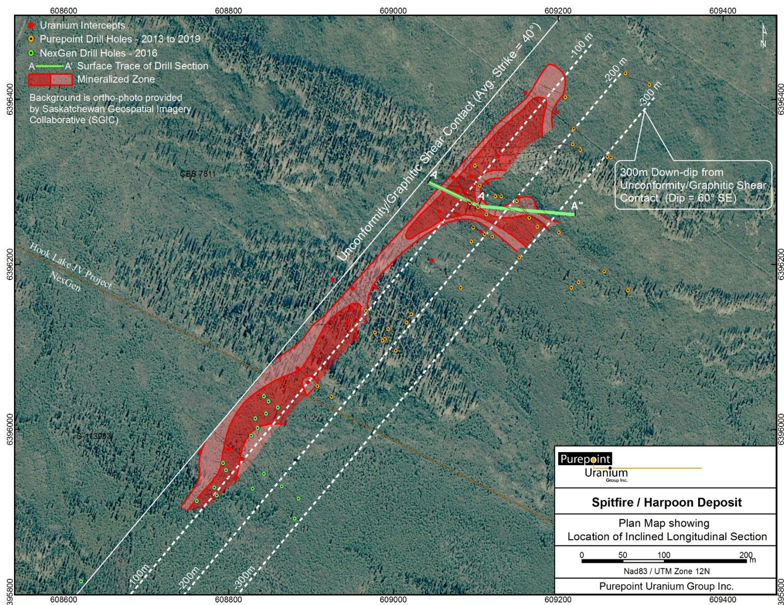
Figure 8: Location Map of the Spitfire / Harpoon Uranium Deposit
