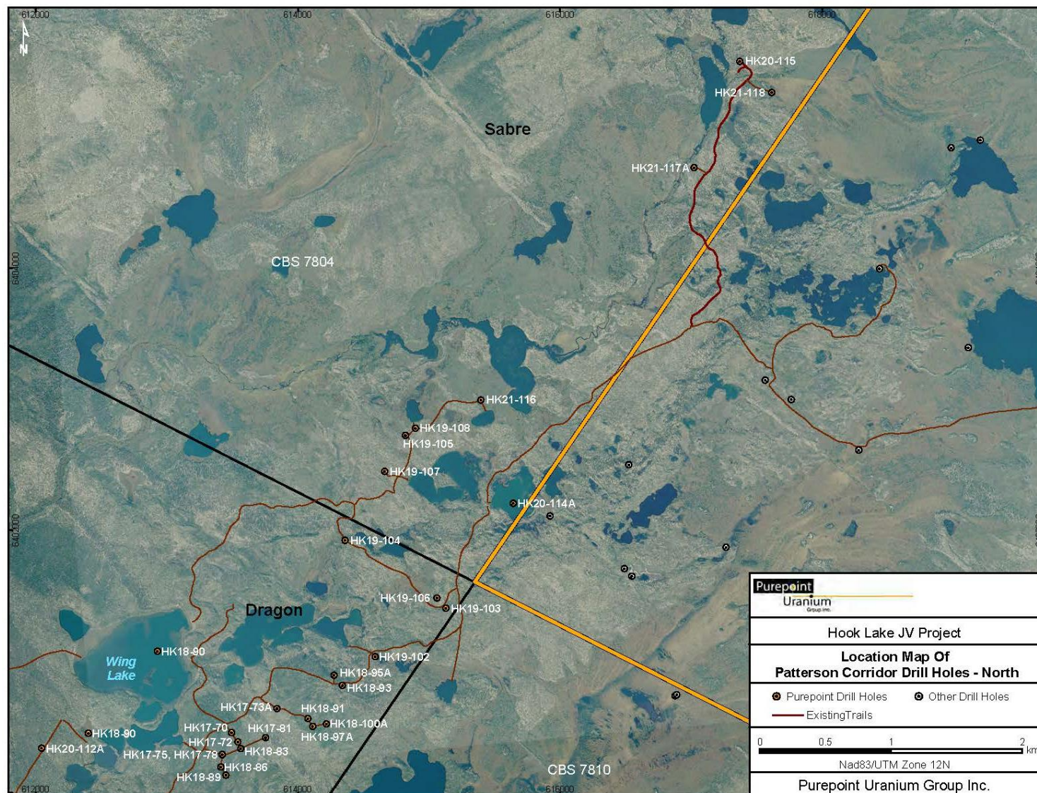
Figure 27: Location Map of Patterson Corridor Drill Holes – North Area
