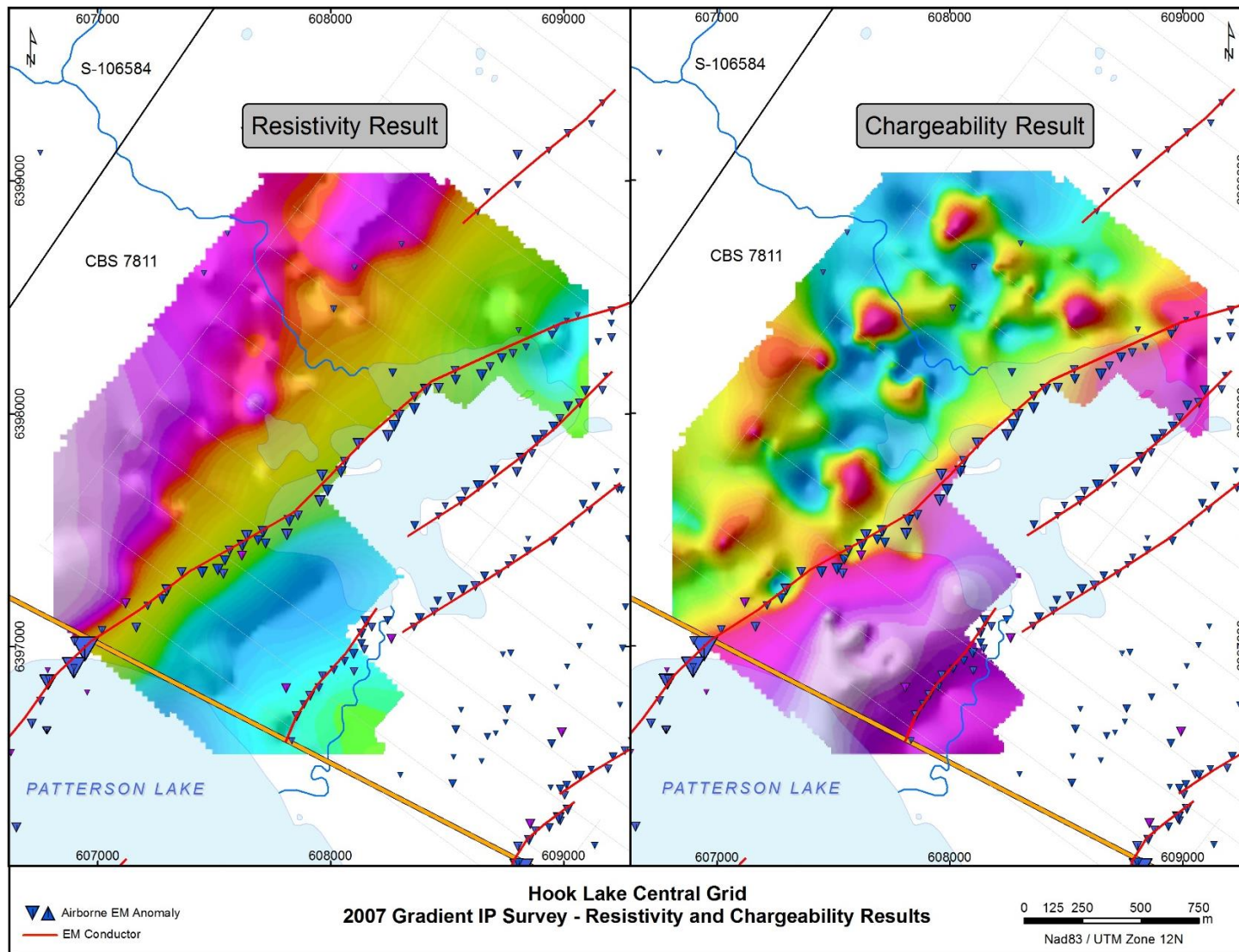
Figure 22: Gradient Induced Polarization Results - Central Grid
