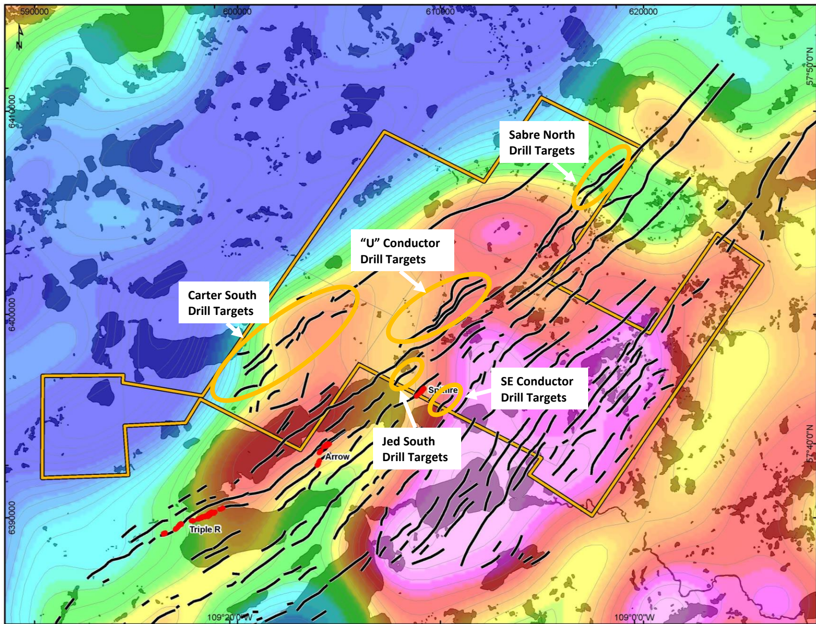
Figure 42: Proposed Priority Drill Targets - 1 st Derivative Gravity Background
