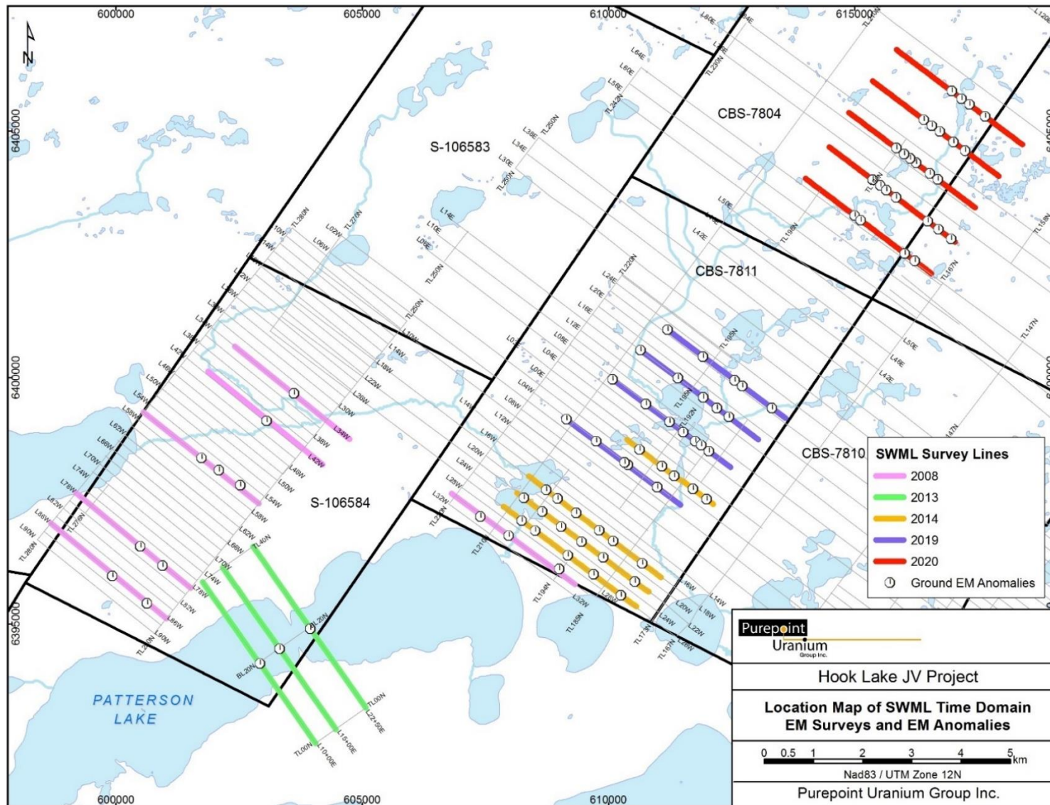
Figure 24: Location Map of Step-Wise Moving Loop TEM Surveys
