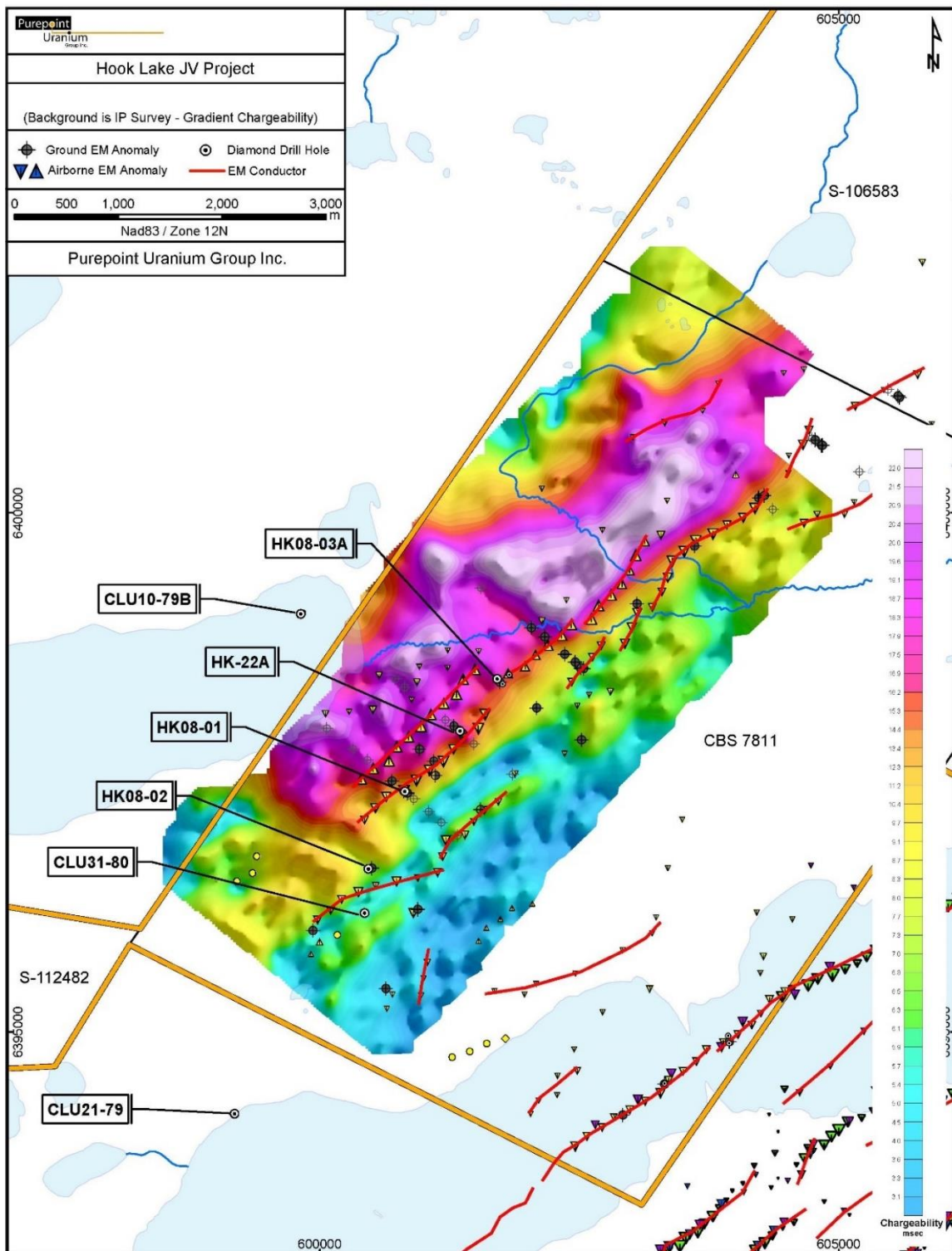
Figure 21: Gradient Chargeability Results – Carter Corridor
