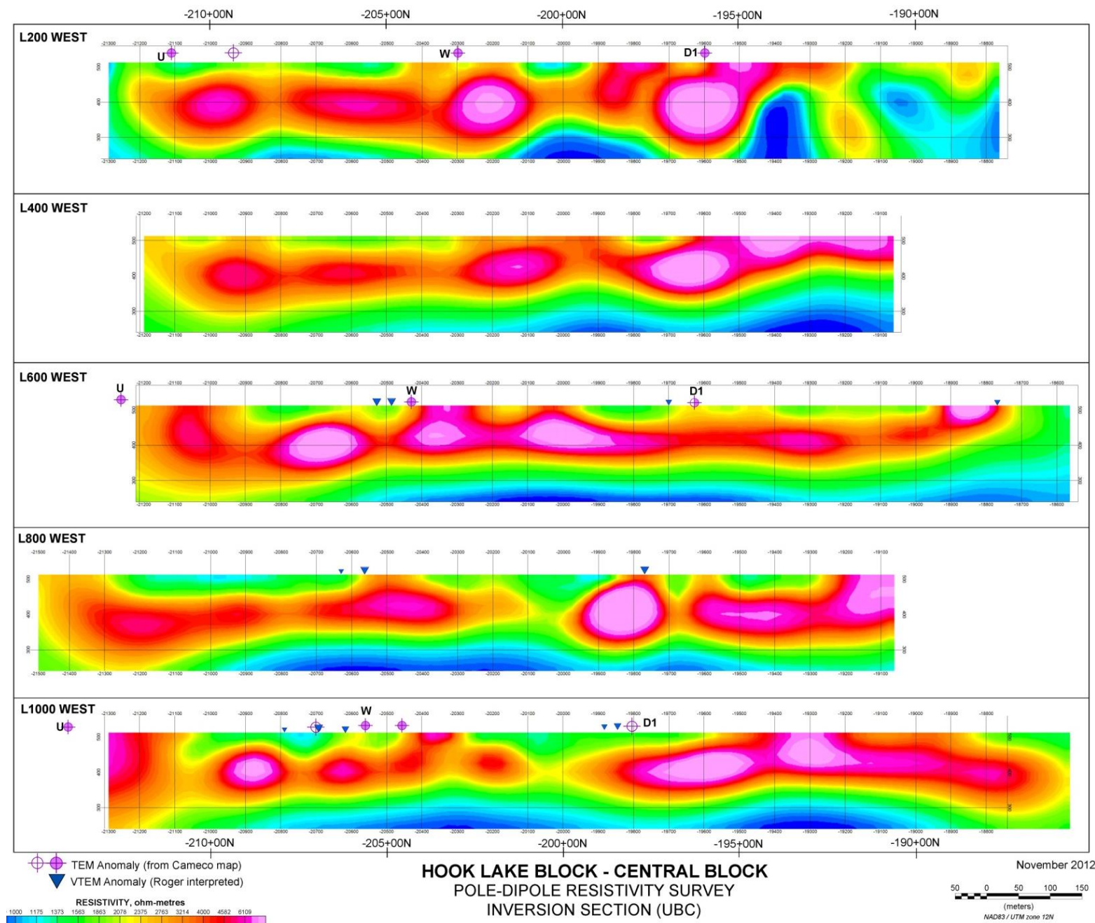
Figure 23: Stacked Pole-dipole Induced Polarization Sections - Central Grid
