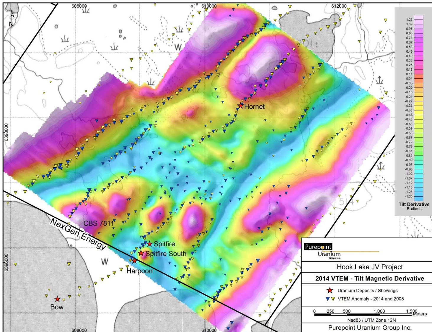
Figure 17: Tilt Magnetic Derivative – 2014 VTEM Survey
