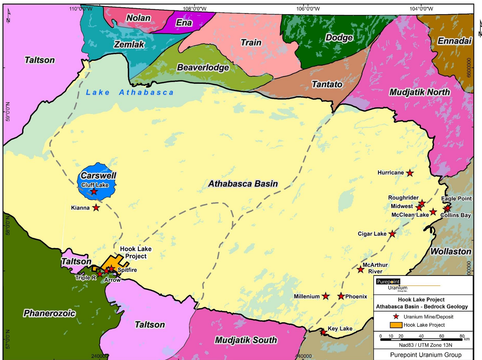
Figure 5: Bedrock Geology of Northern Saskatchewan
