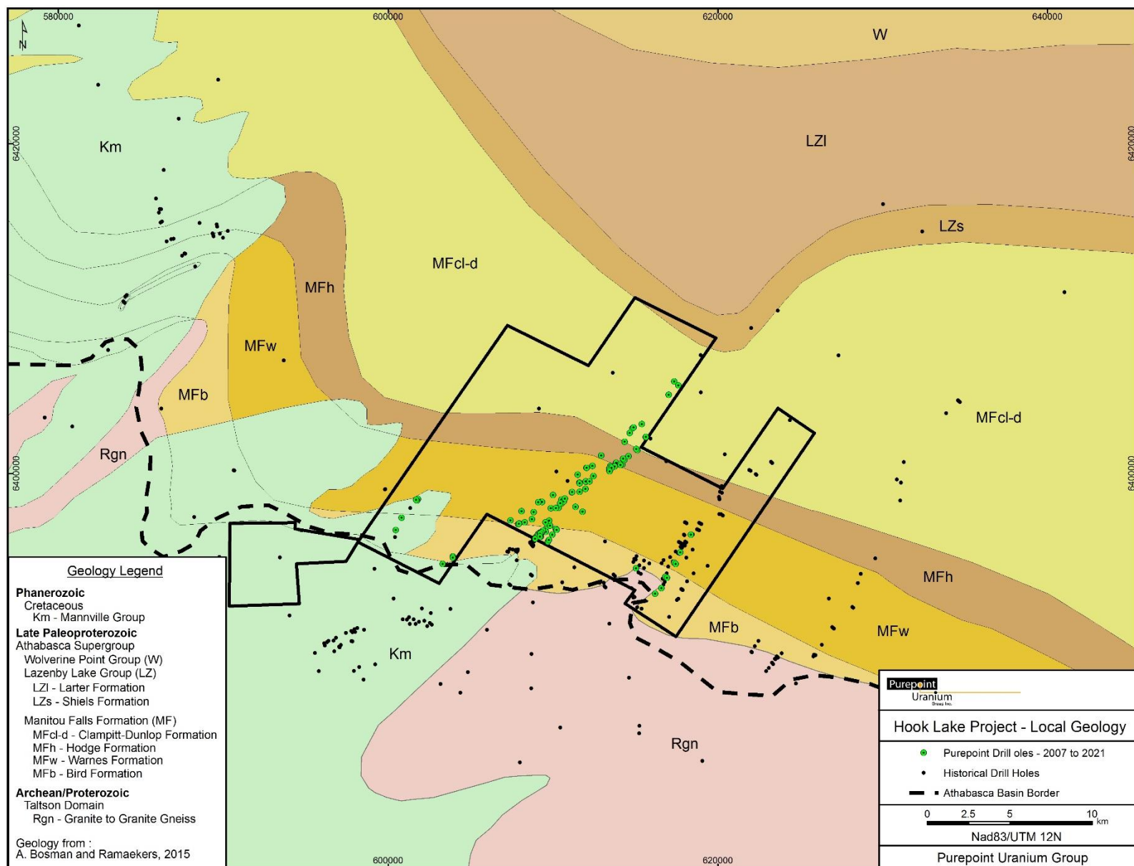
Figure 6: Local Geology of the Hook Lake Project Area
