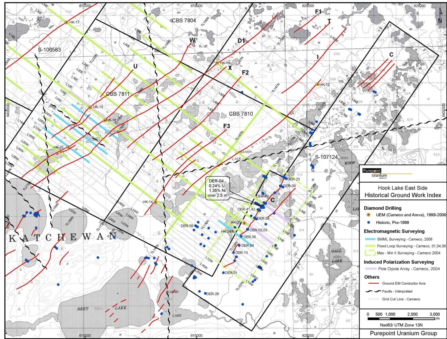
Figure 3: Historical Ground Work on the Hook Lake Project – East Side
