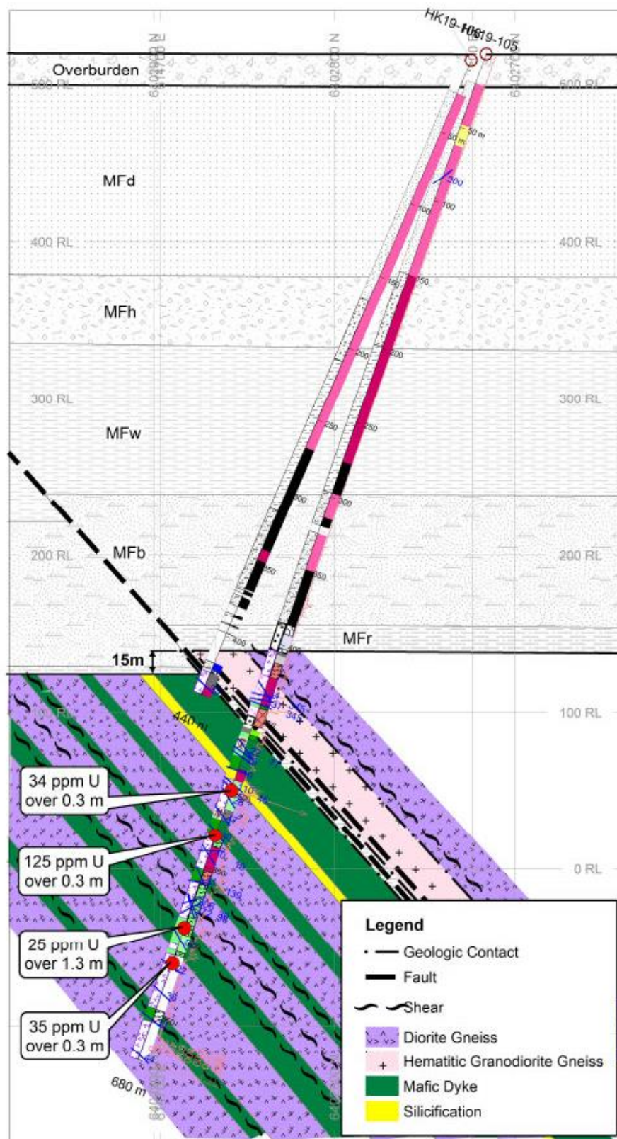
Figure 35: Drill Section of HK19-105 and HK19-108 – Sabre Area
