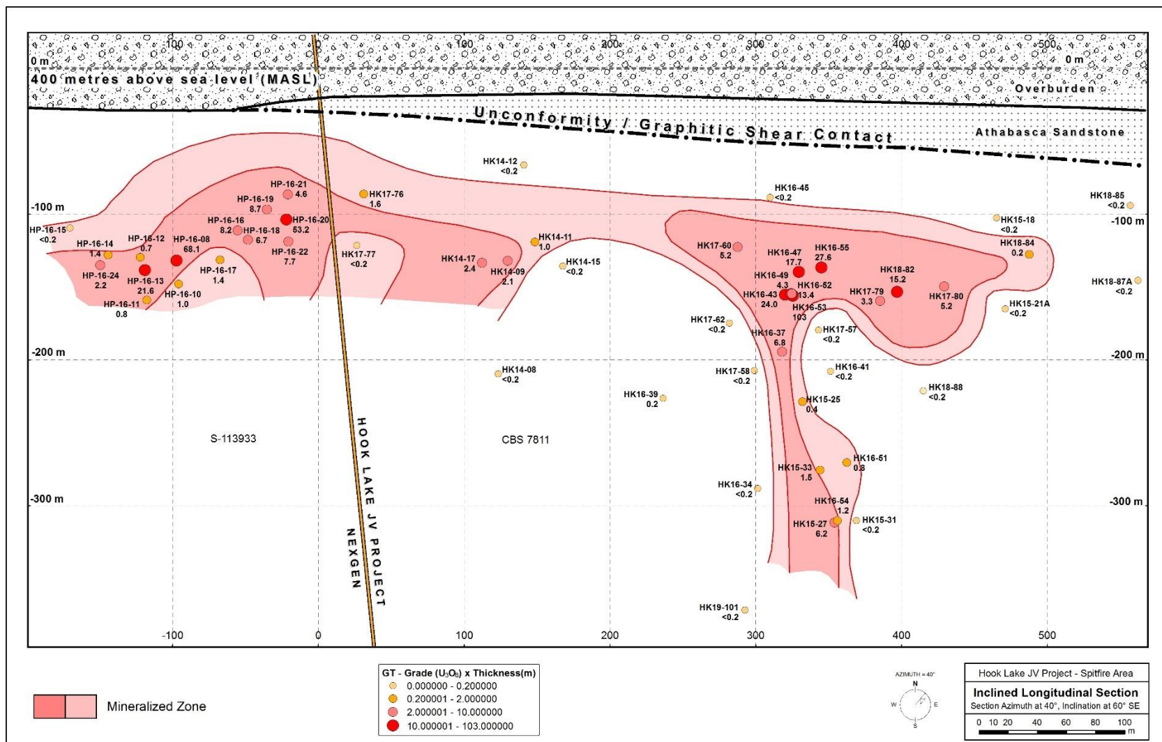
Figure 31: Inclined Longitudinal Section of Spitfire Zone
