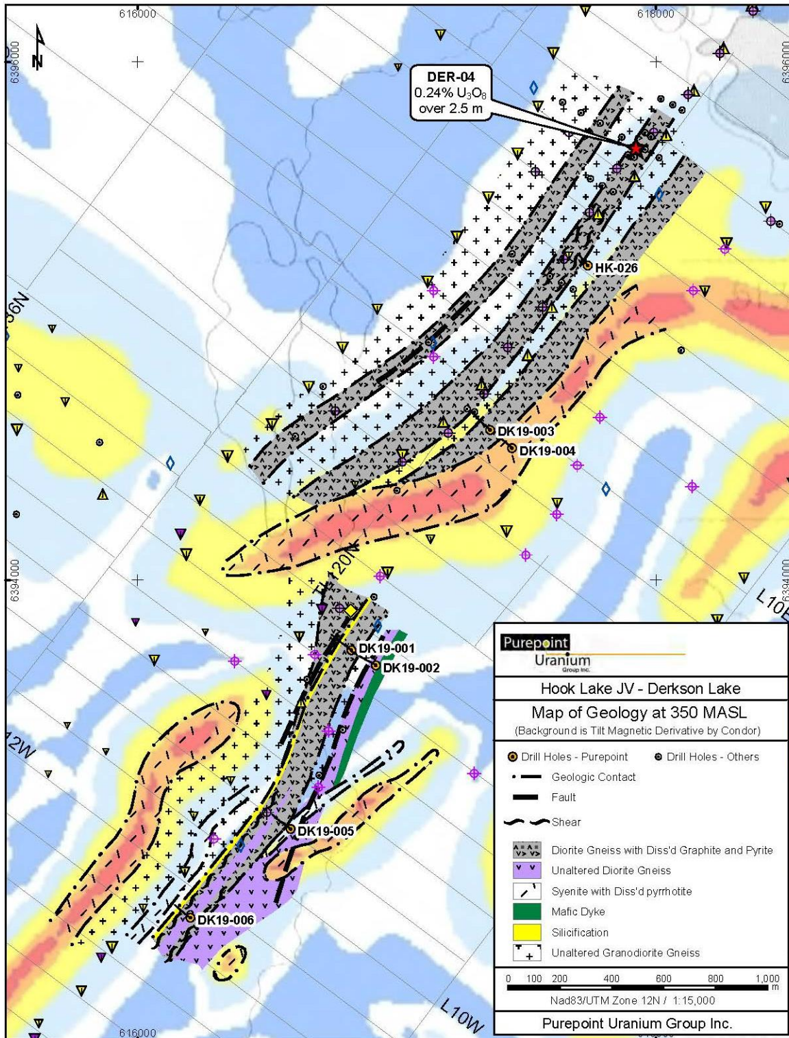
Figure 37: Interpreted Derkson Area Geology – Magnetic Tilt Background
