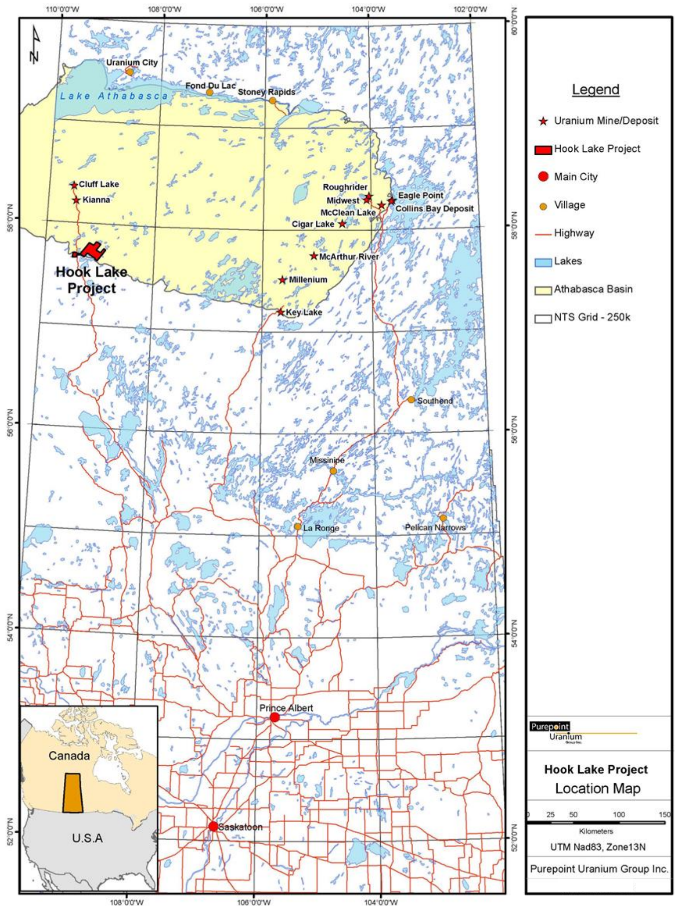
Figure 1: Location Map of the Hook Lake Project
