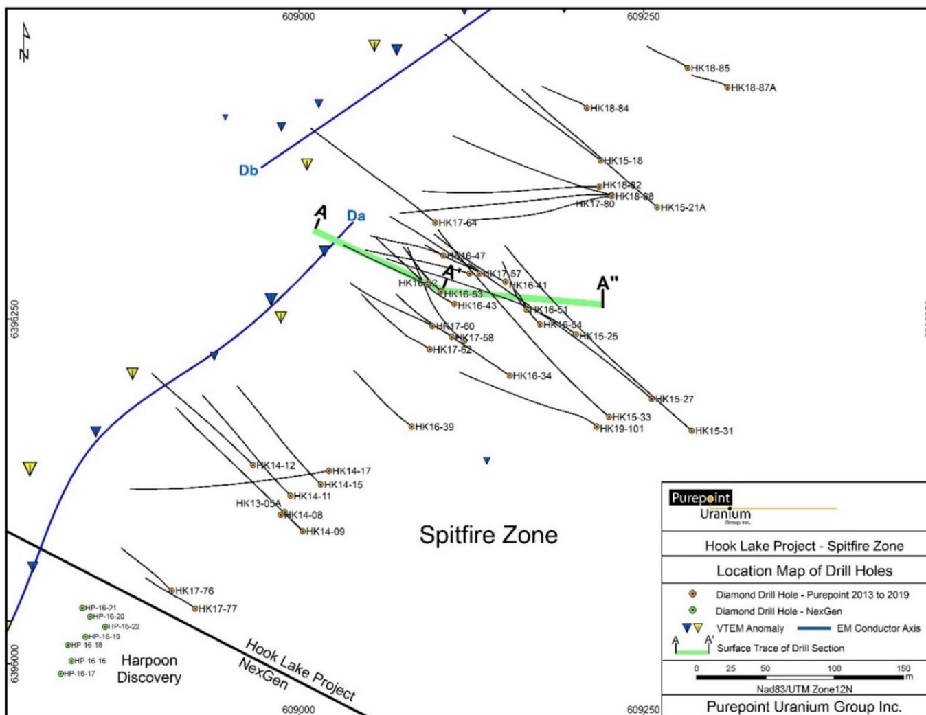
Figure 30: Location Map of Spitfire Zone Drill Holes
