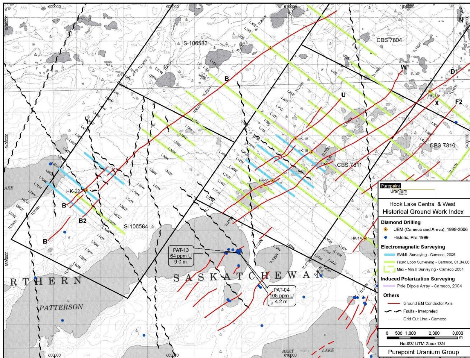
Figure 4: Historical Ground Work on the Hook Lake Project – West Side
