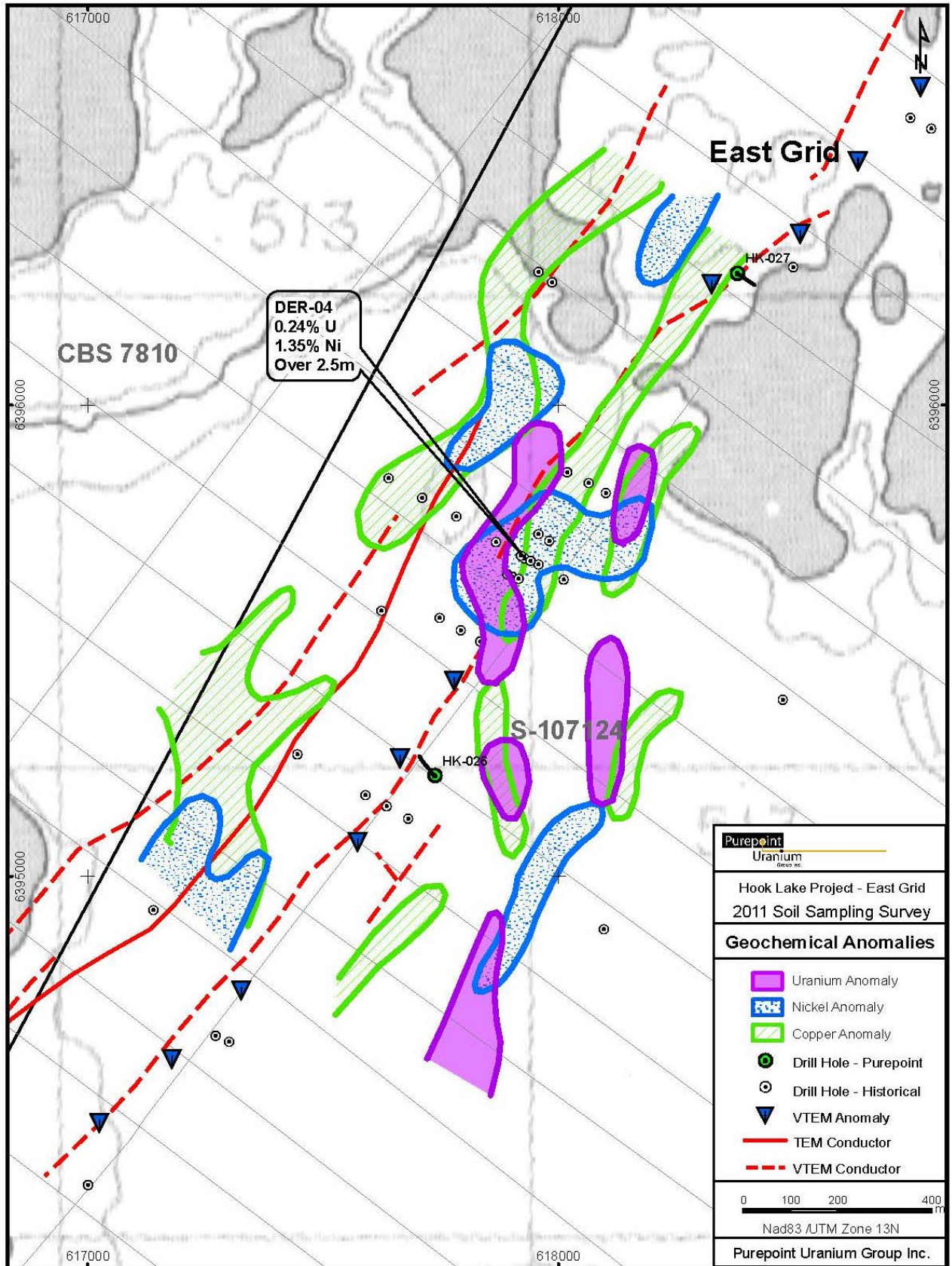
Figure 12: Compilation Map of U, Ni and Cu Soil Anomalies
