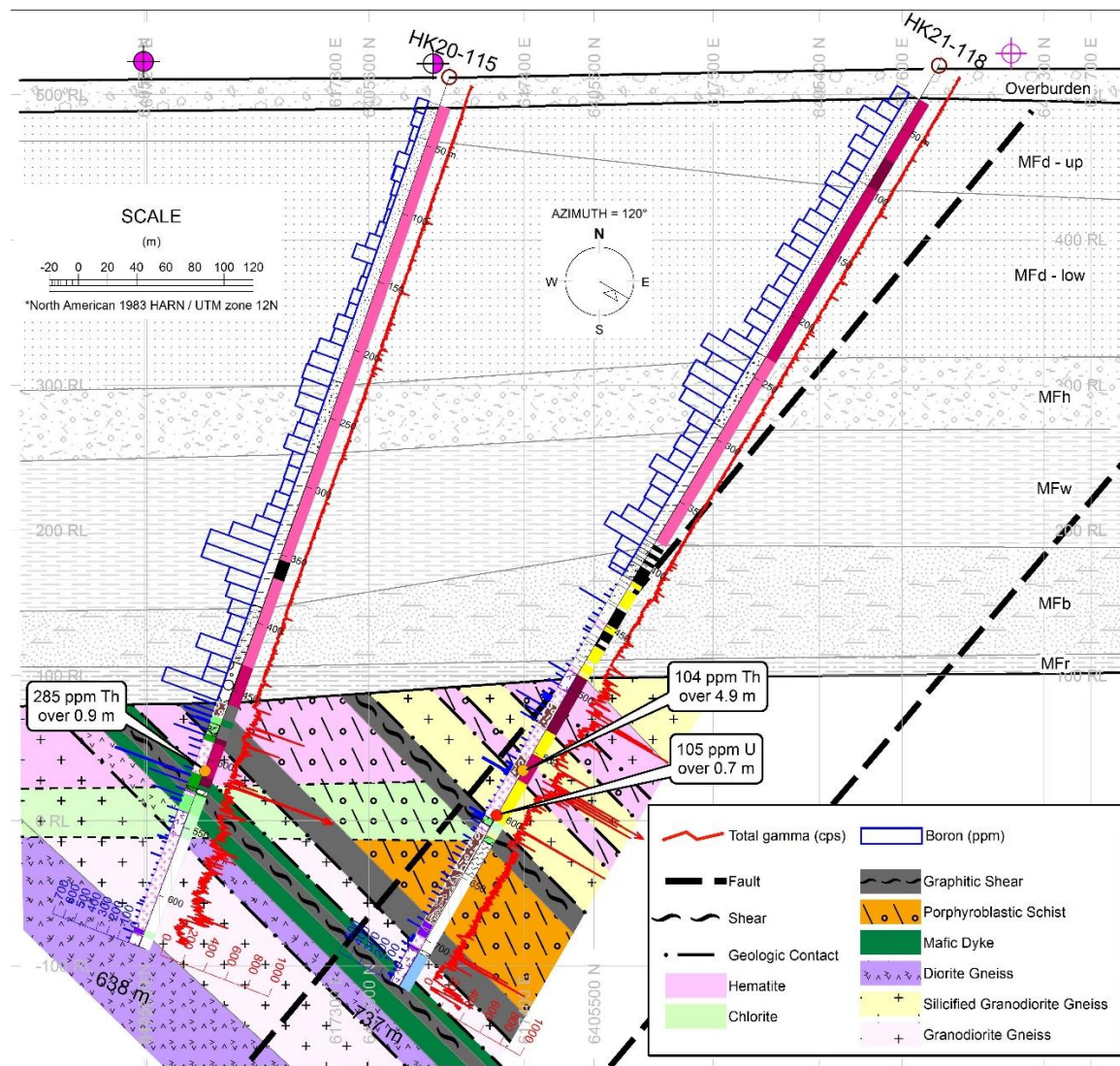
Figure 36: Drill Section of HK20-115 and HK21-118 – Sabre Area
