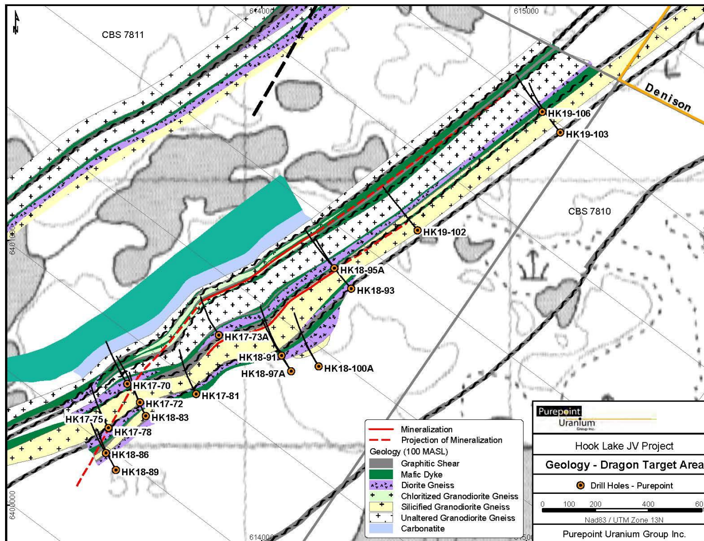
Figure 33: Interpreted Geology – Dragon Area
