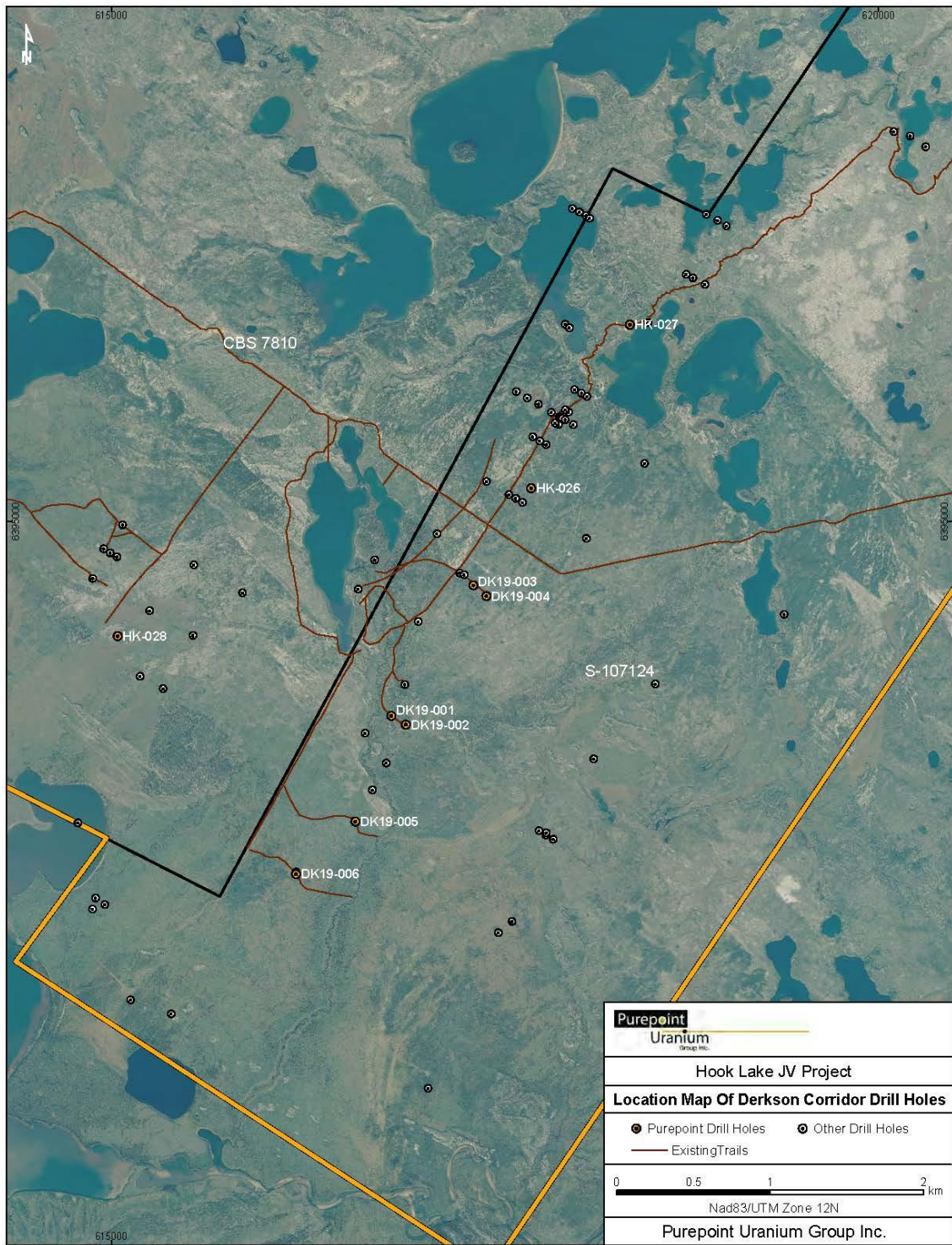
Figure 29: Location Map of Derkson Corridor Drill Holes
