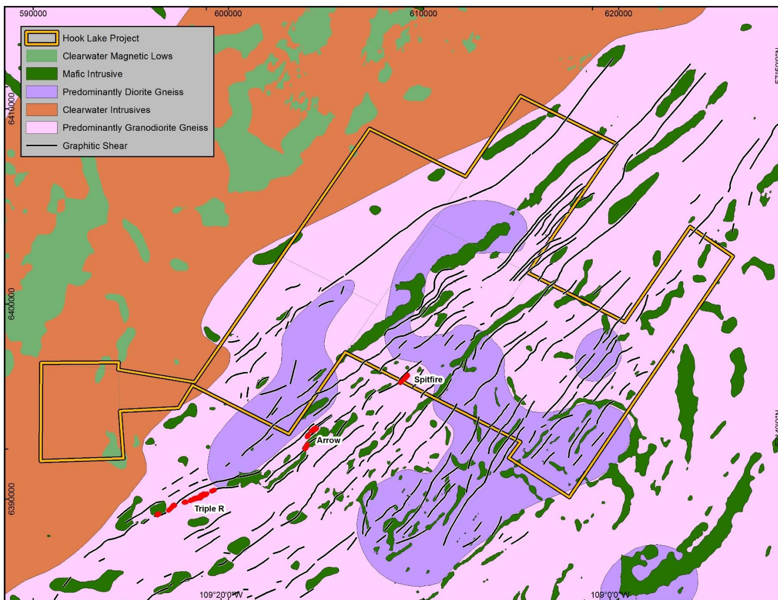
Figure 7: Interpreted Basement Geology of the Hook Lake Project Area
