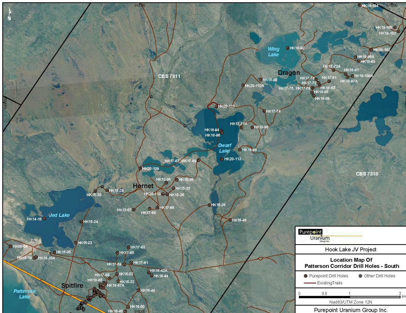
Figure 26: Location Map of Patterson Corridor Drill Holes – South Area
