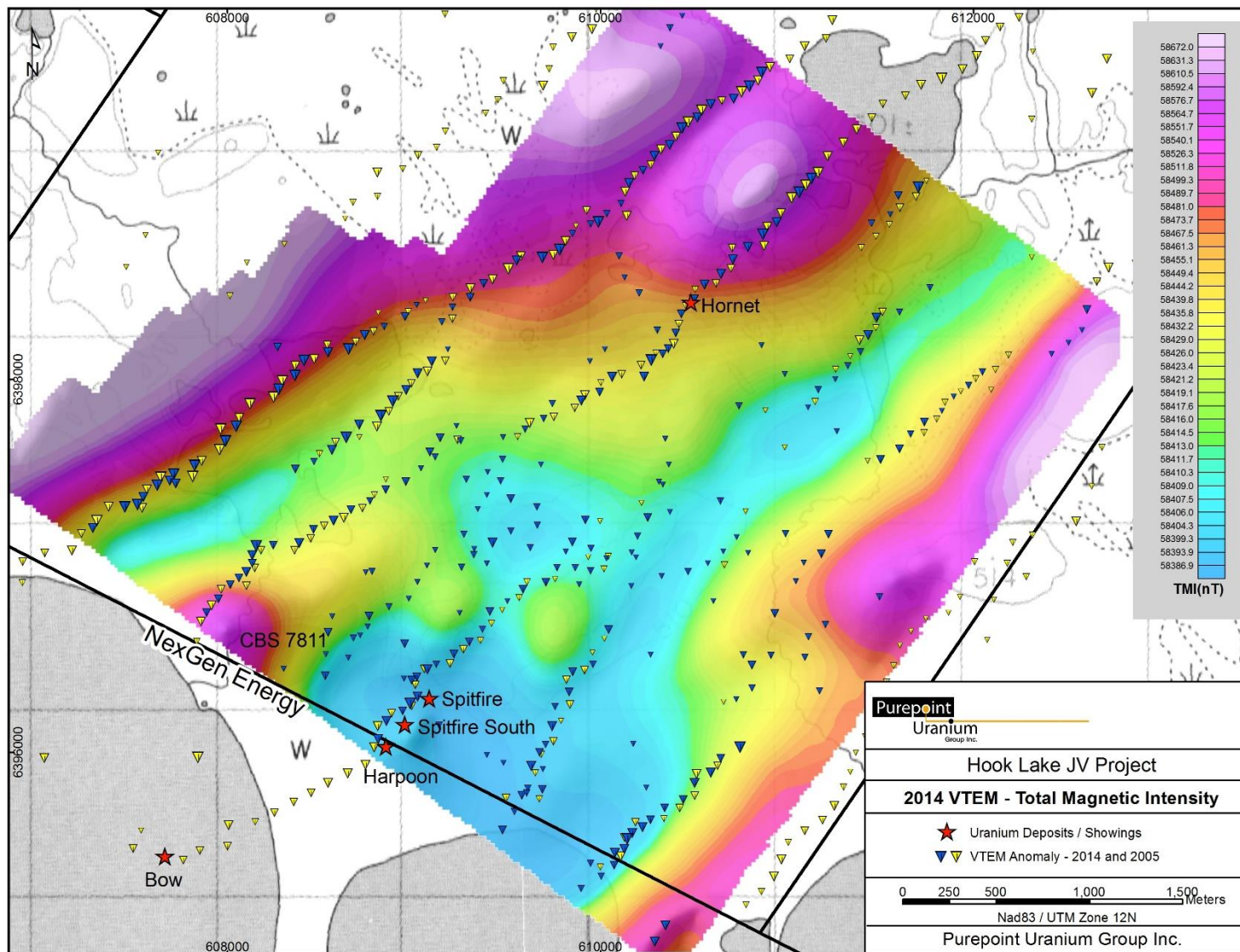
Figure 16: Total Magnetic Intensity – 2014 VTEM Survey
