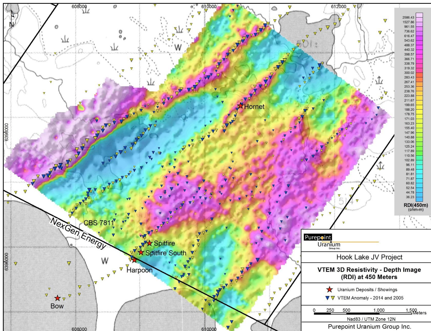
Figure 18: Resistivity Depth Image (RDI) at 450 Metre Depth
