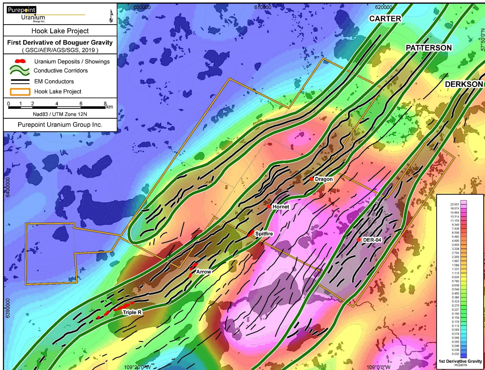
Figure 11: Structural / Conductive Corridors with 1 st Derivative Gravity Background
