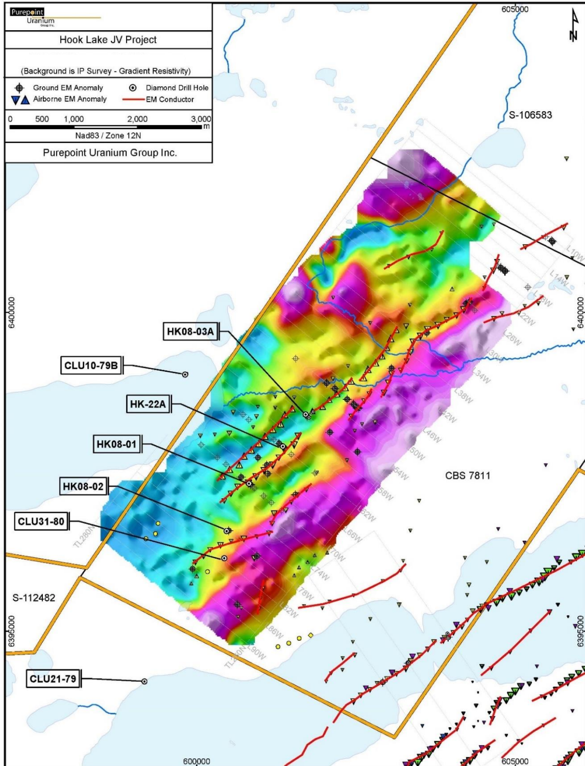
Figure 20: Gradient Resistivity Results – Carter Corridor
