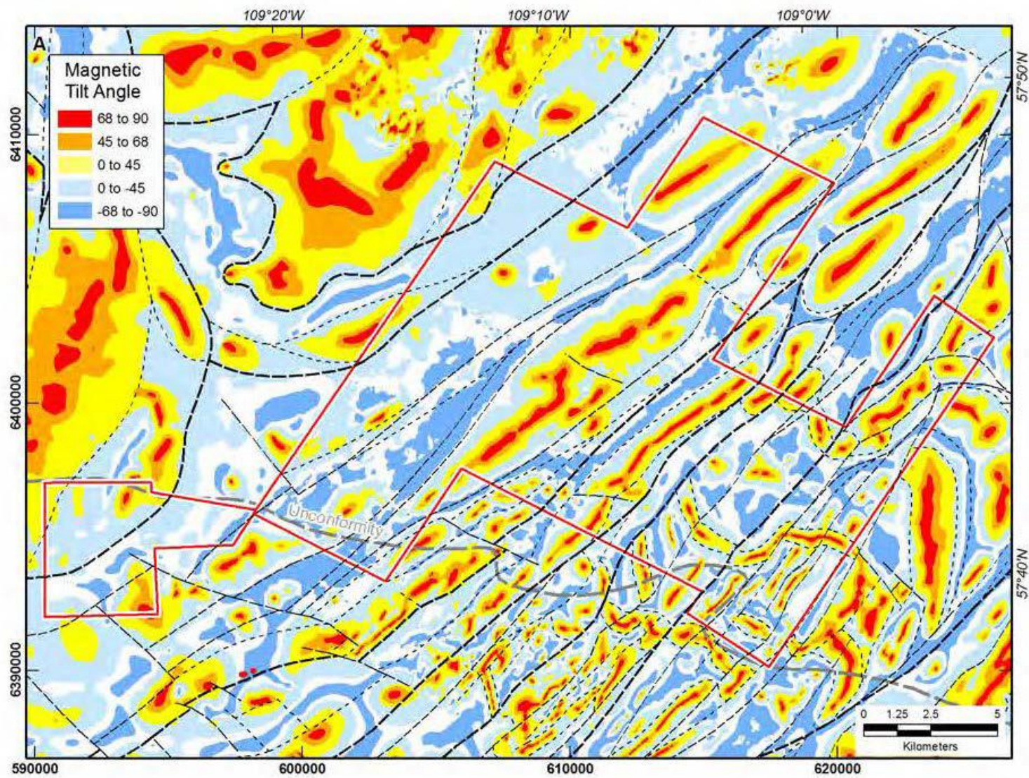
Figure 14: Magnetic Tilt with Structural Interpretation (Condor, 2013)
