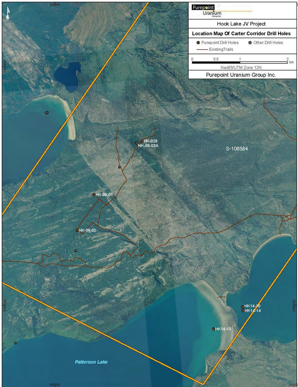
Figure 28: Location Map of Carter Corridor Drill Holes
