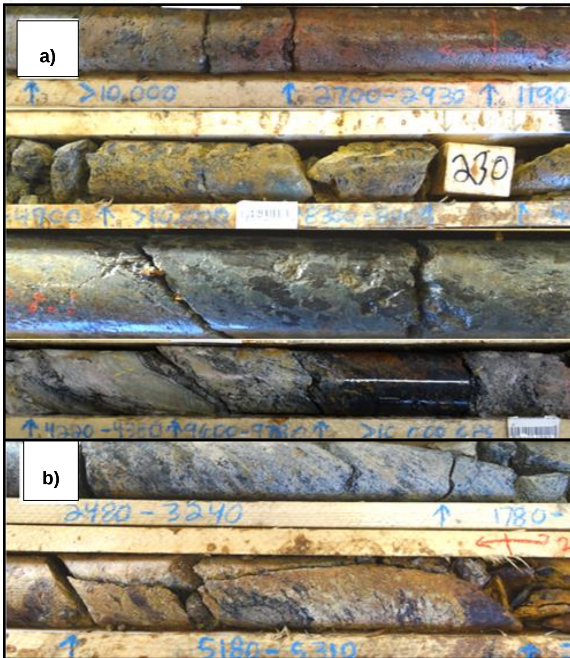
Figure 10: Basement Mineralization Styles of Spitfire Deposit
