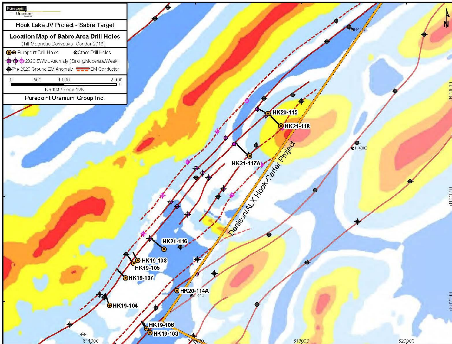
Figure 34: Location Map of Sabre Area Drilling – Magnetic Tilt Background
