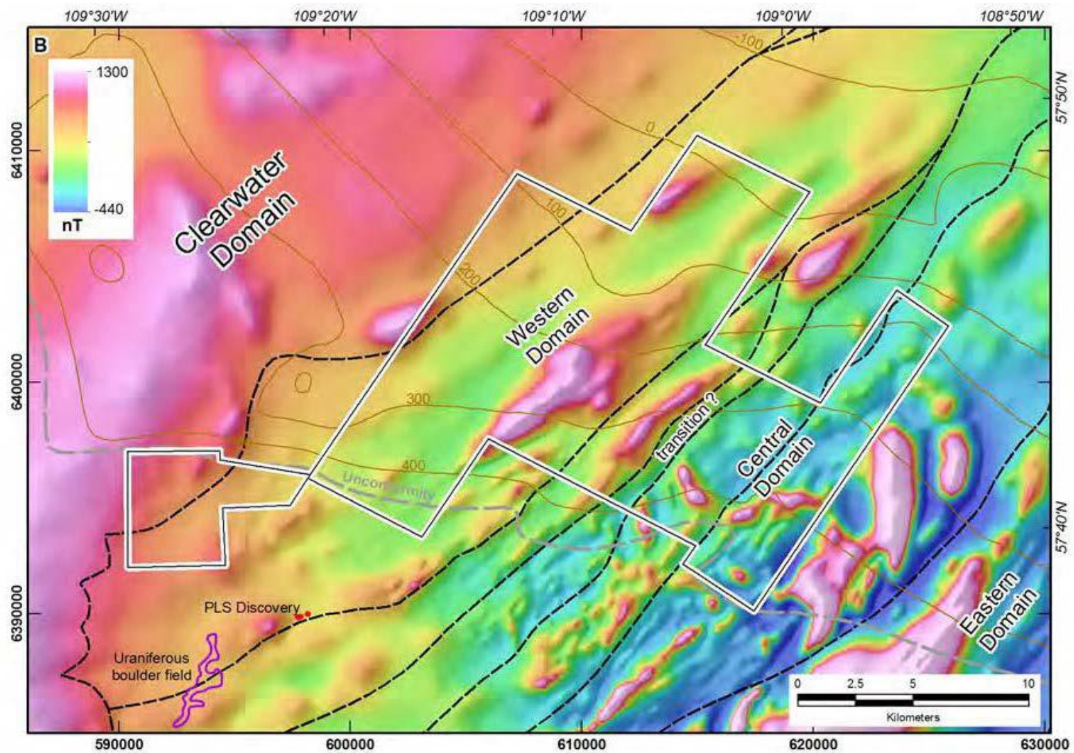
Figure 13: Total Magnetics with Interpreted Structural Domains (Condor, 2013)
