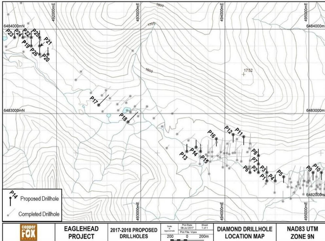
Figure 26-1 Proposed Drillholes
