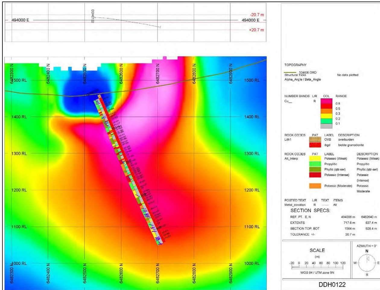
Figure 7-12 Cross-section through Central Bornite Zone showing Drillhole 122 against a Background of Titan 24 Chargeability (after Quist, 2015)
