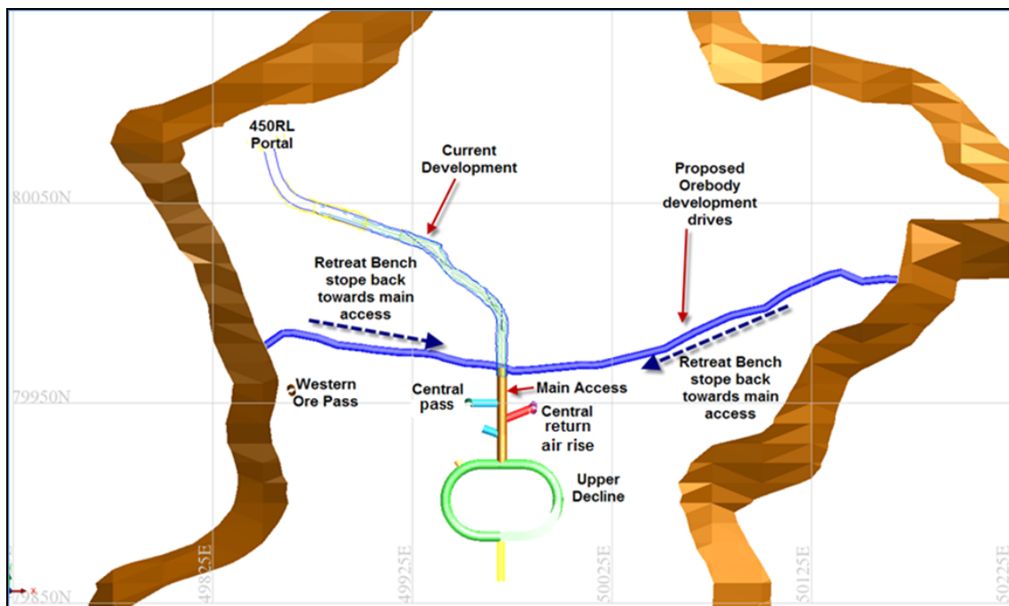
Figure 5 Mine Design Layout, 450 RL
