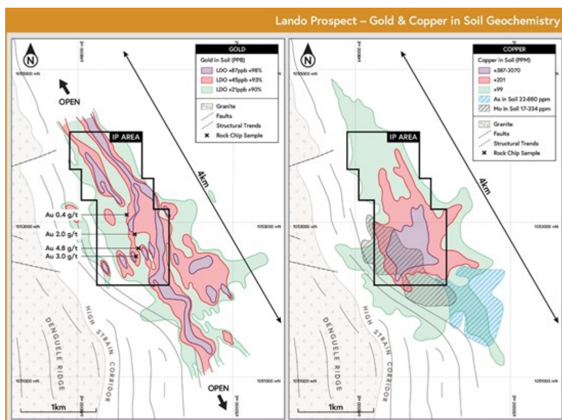
Figure 1: Gold (left) and Copper (right) soil geochemistry for the Lando target.
