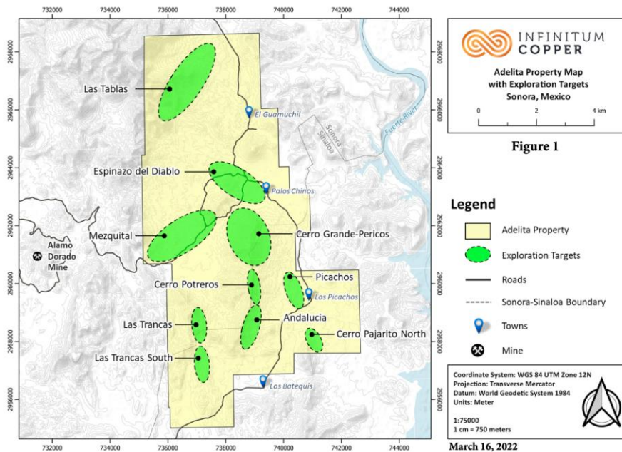
Figure 1. Plan View
