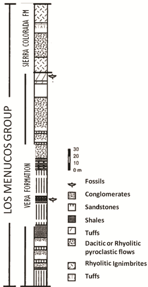
FIGURE 3. STRATIGRAPHIC COLUMN
