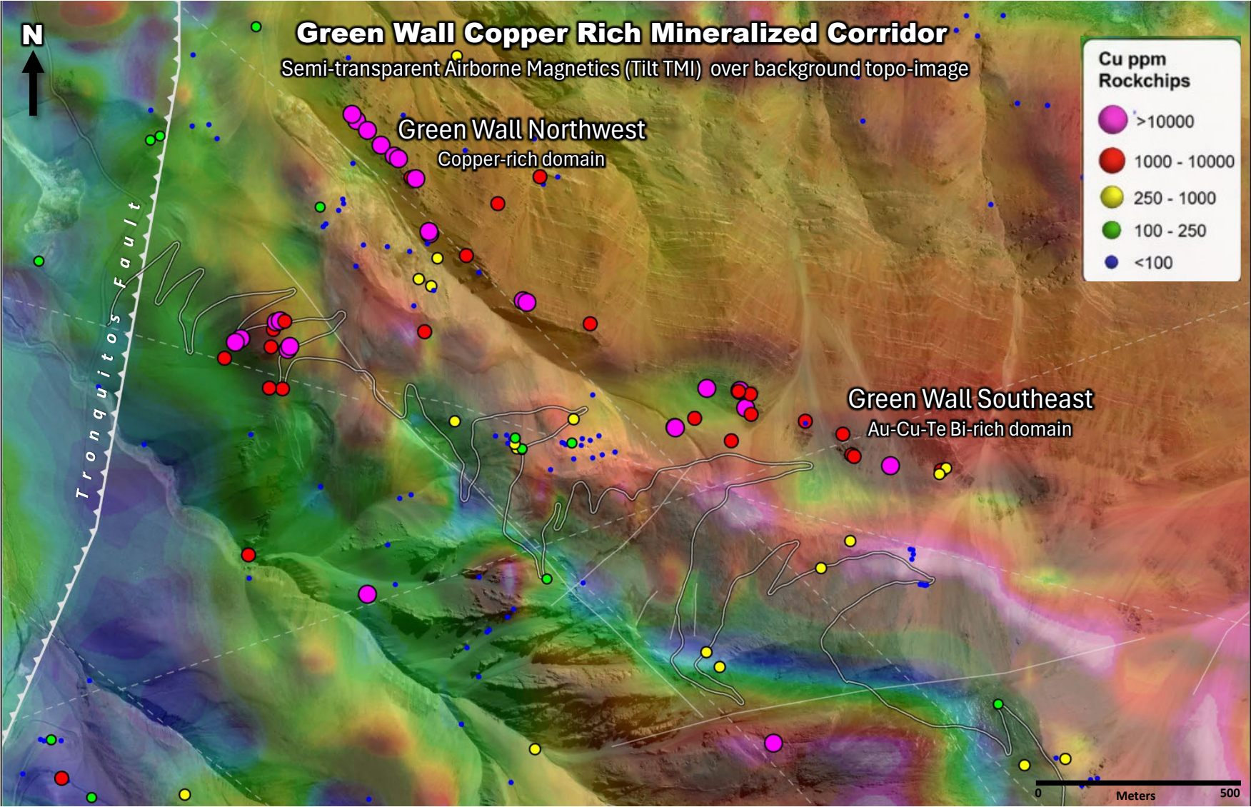
Green Wall copper-rich mineralized corridor, Sobek Central. Airborne magnetic image showing the spatial relationship between copper-rich rock-chip samples, interpreted structural trends and the broader Green Wall mineralized corridor. The map highlights the Green Wall Northwest copper-rich domain and the Green Wall Southeast Au-Cu-Te-Bi domain , developed along a NW-trending corridor.
