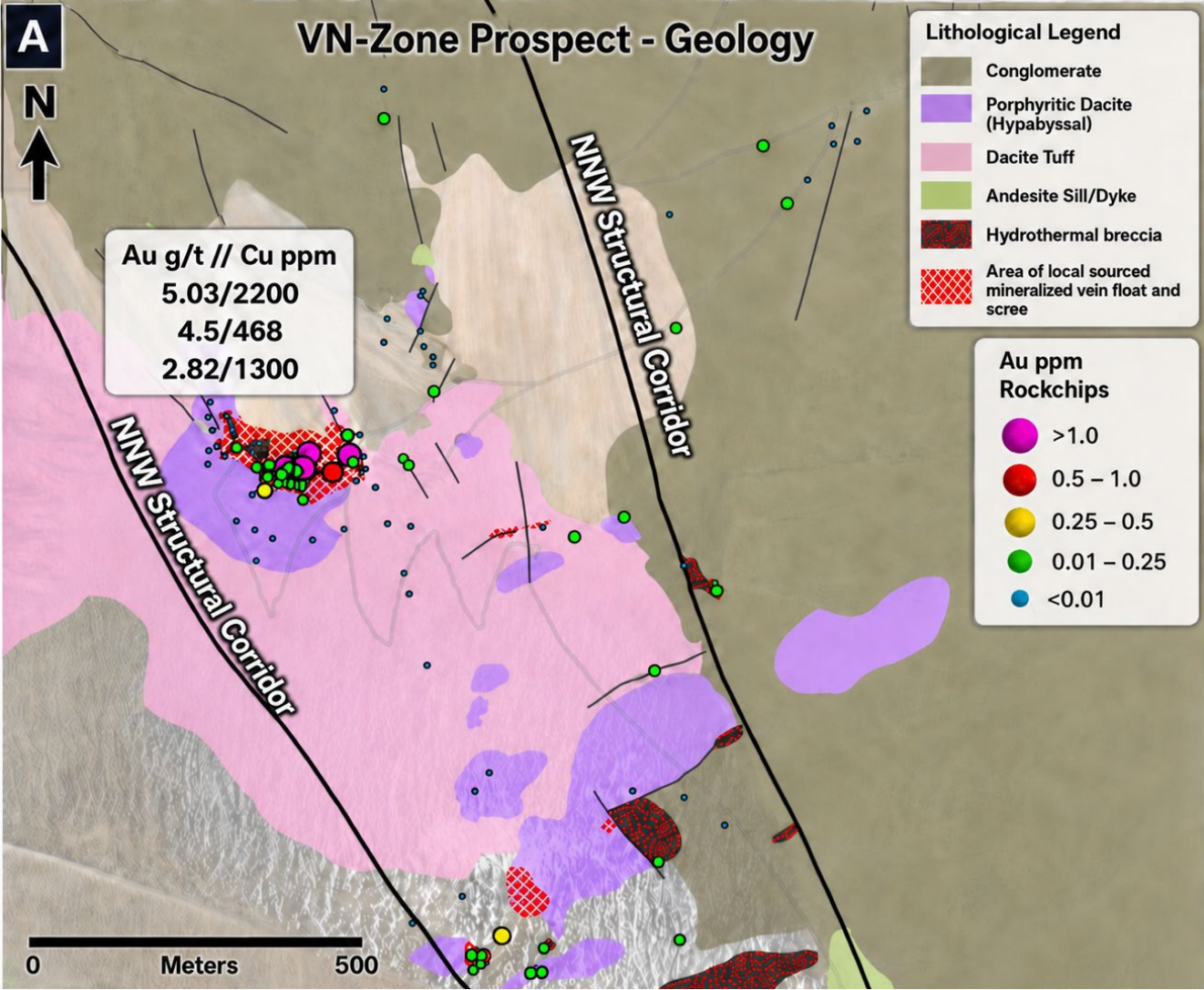
Figure 3: Sobek Central Corridor - VN-Zone Geological Setting, Banded Black Quartz Veins and Magnetite Quartz Veins
