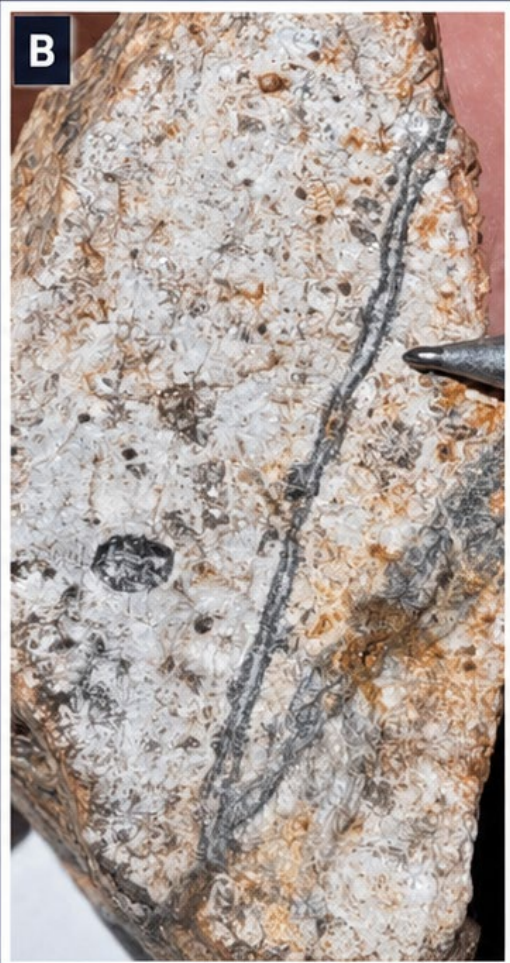
B. Banded black quartz vein
