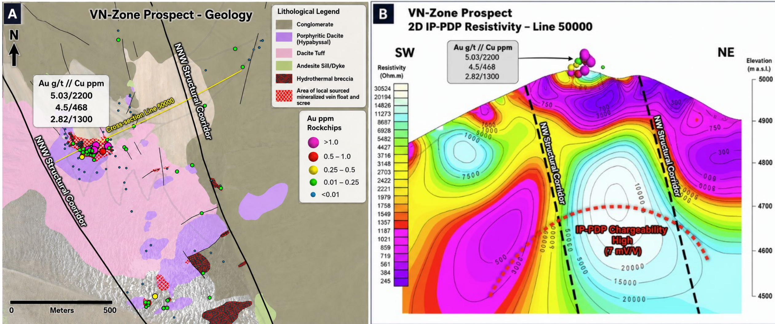
Figure 2: Sobek Central Corridor - VN-Zone IP Resistivity Section
