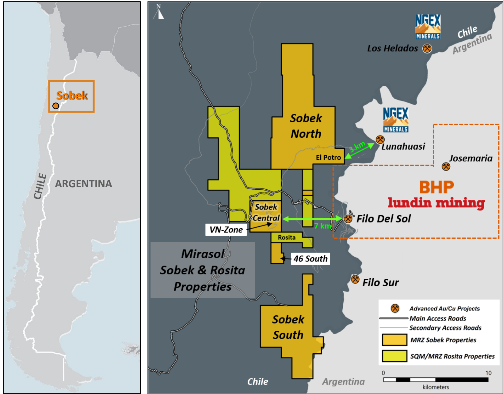
Figure 1: Vicuña District - Sobek Property Package including Sobek Central Corridor of Targets
