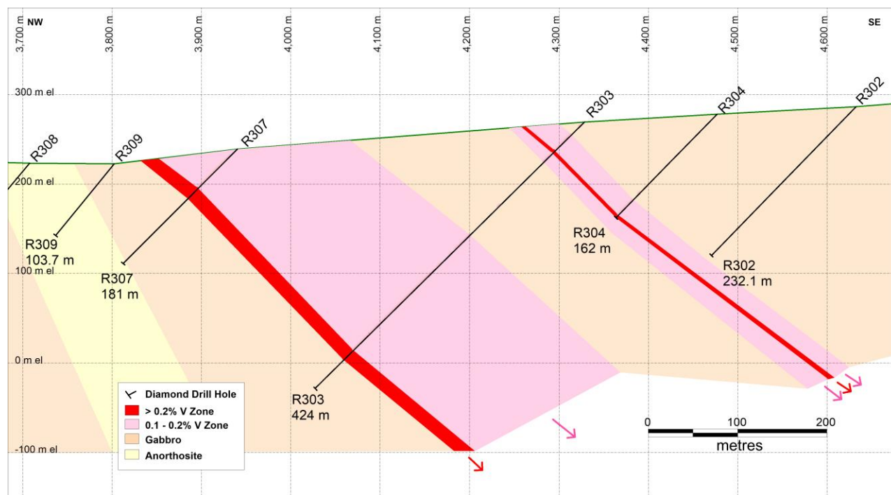
Figure 7-6: Cross Section – Akanvaara MTGB Target
