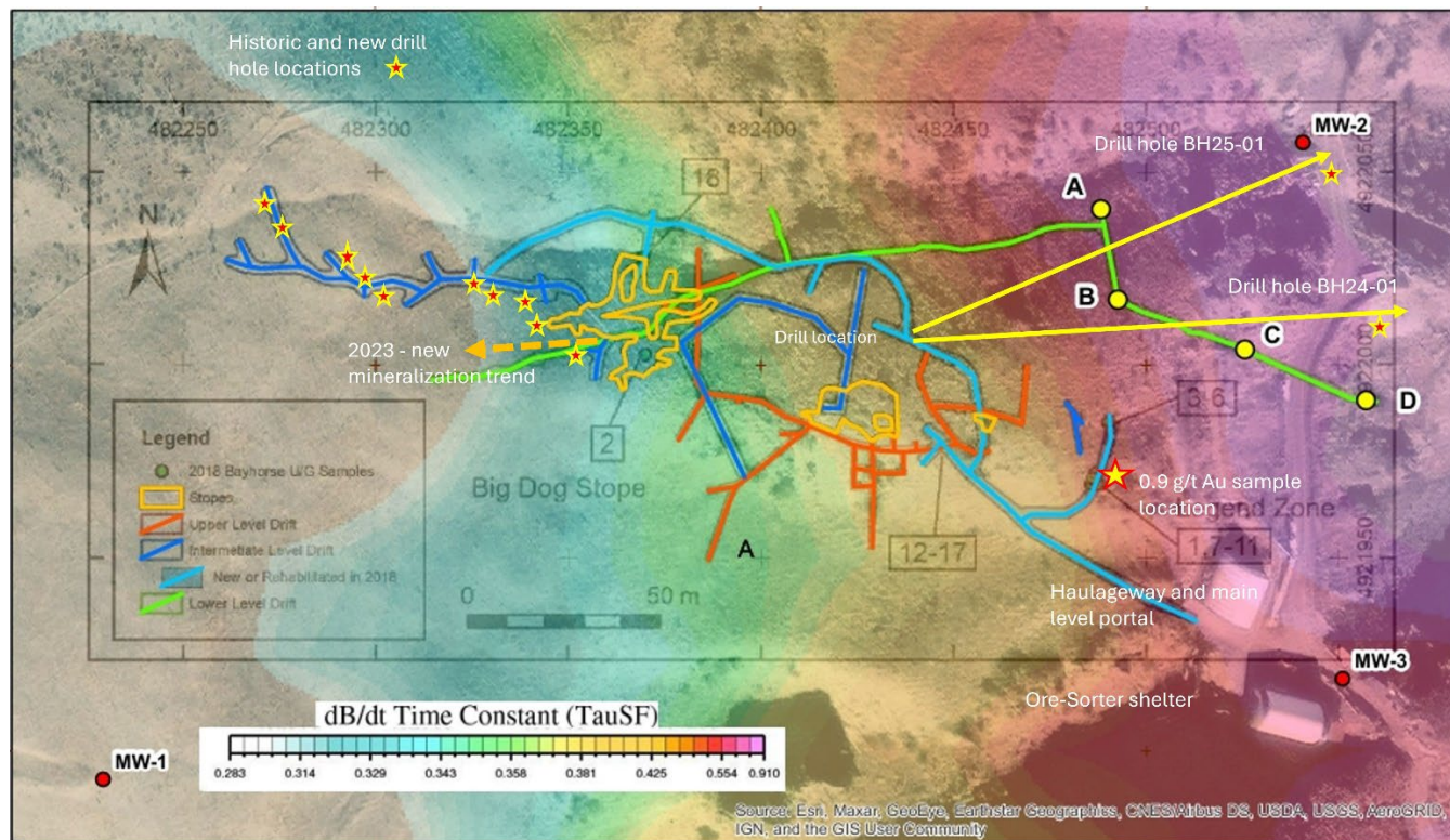
Figure 1. Bayhorse underground plan shown historic drill holes, current drill hole BH24-01 and planned drill hole BH25-01
