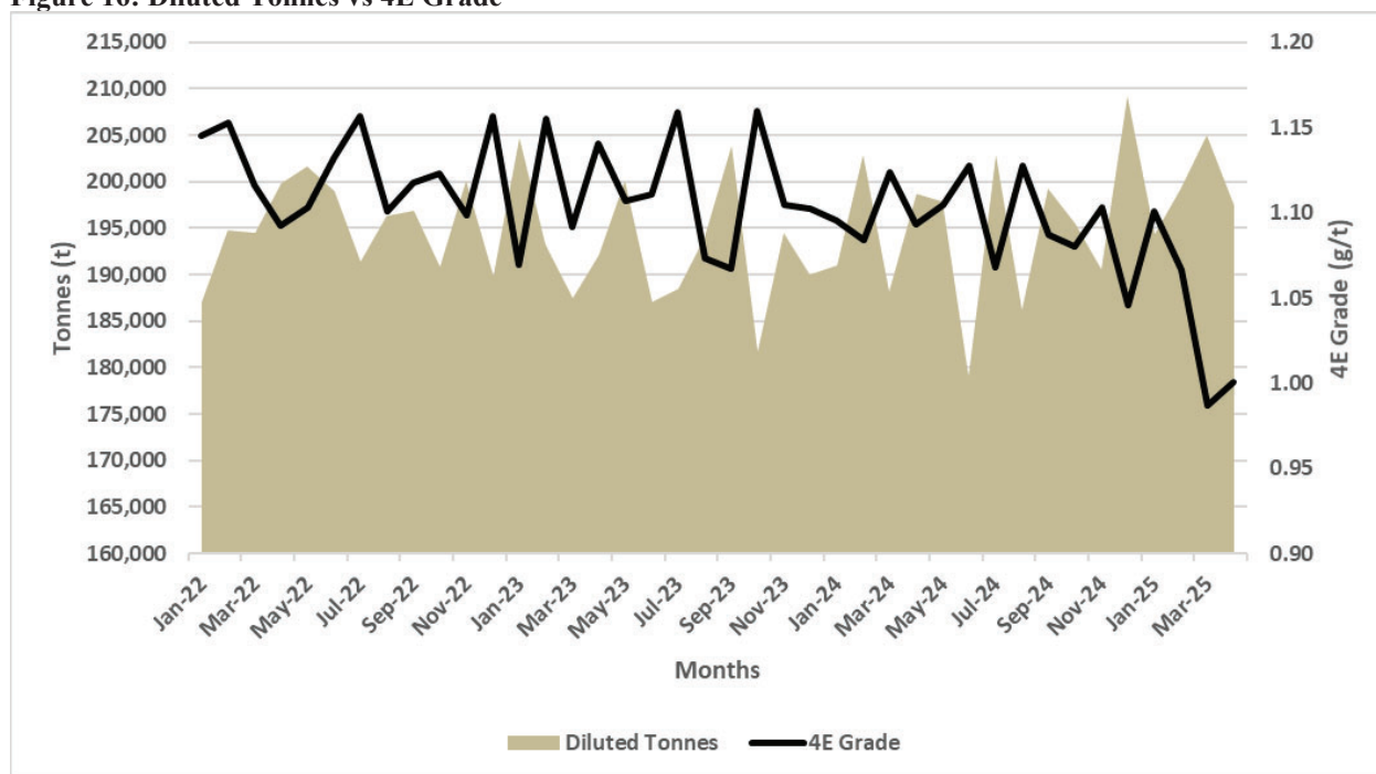
Figure 16: Diluted Tonnes vs 4E Grade
