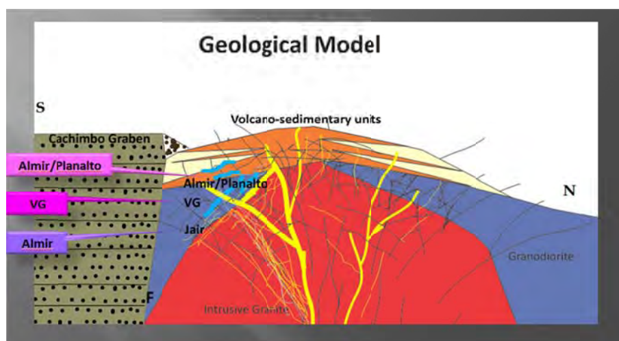
Fig. 7. Geological Model for gold mineralization at Boa Vista (after BGC files-2011)
