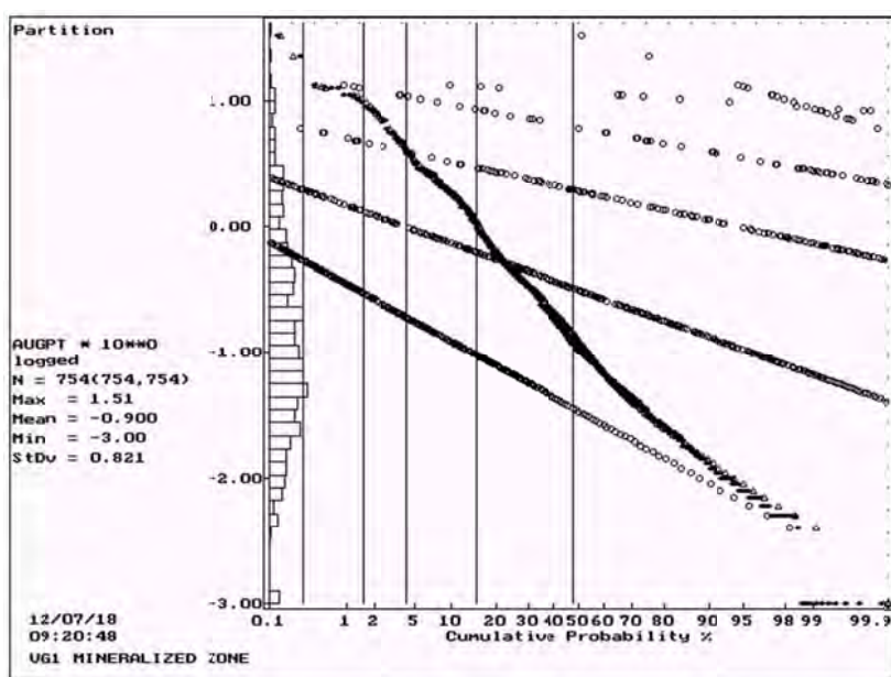
Figure 14: Lognormal Cumulative Frequency Plot for Au in Mineralized Solid
