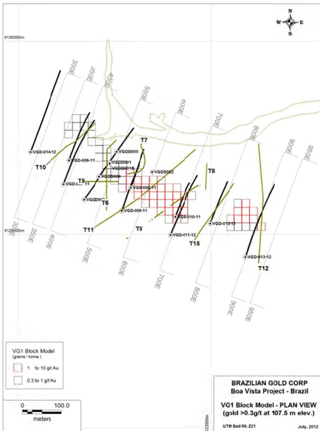
Fig. 17. VG1 Plan View - All blocks . >0.3 g/t gold. 107.5 metre slice
