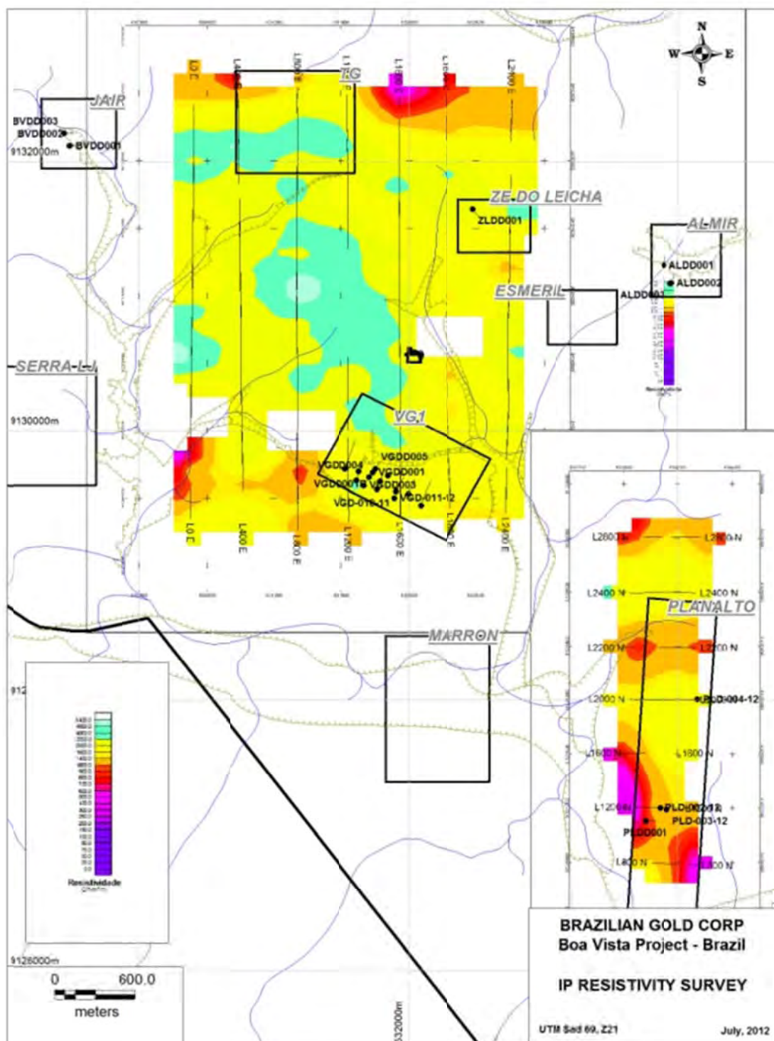
Fig. 10. Fugro-GeoMag IP resistivity survey at VG1 and Planalto prospects
