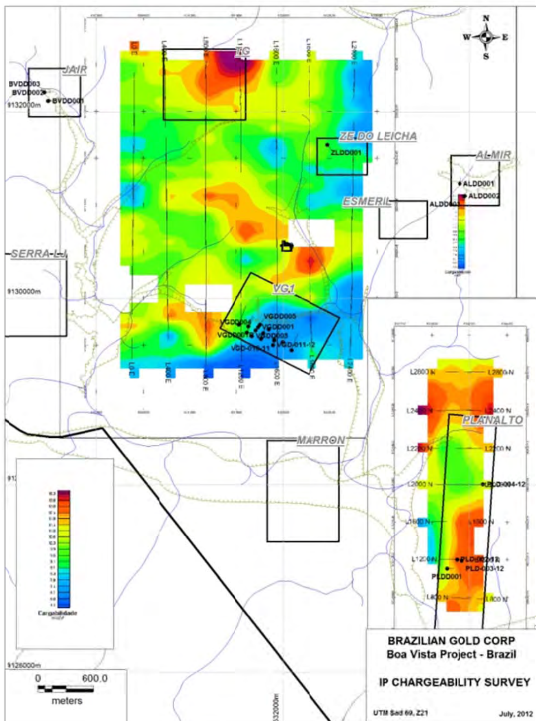
Fig. 9. Fugro-GeoMag IP chargeability survey at VG1 and Planalto prospects
