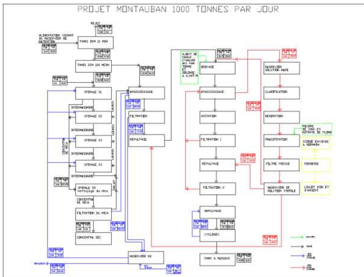
Error! Reference source not found.: Project processing flowsheet
