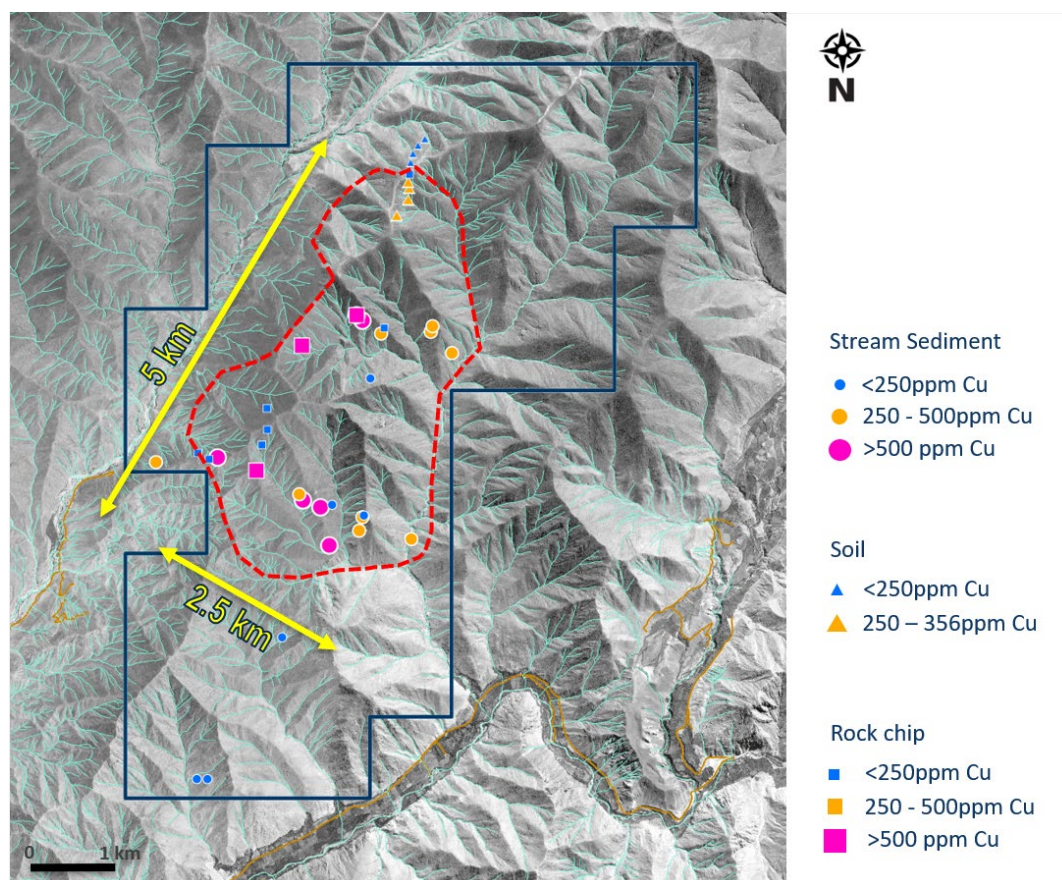
Figure 1: Map of the Lacsha copper project, showing historical copper geochemistry results for stream sediment, soil, and rock chip sampling, which defines a target area approx. 5.0km by 2.5km in area.
