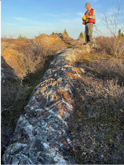
(g) Exposure of Hurwitz Group quartzite, iron formation and quartz veining.
