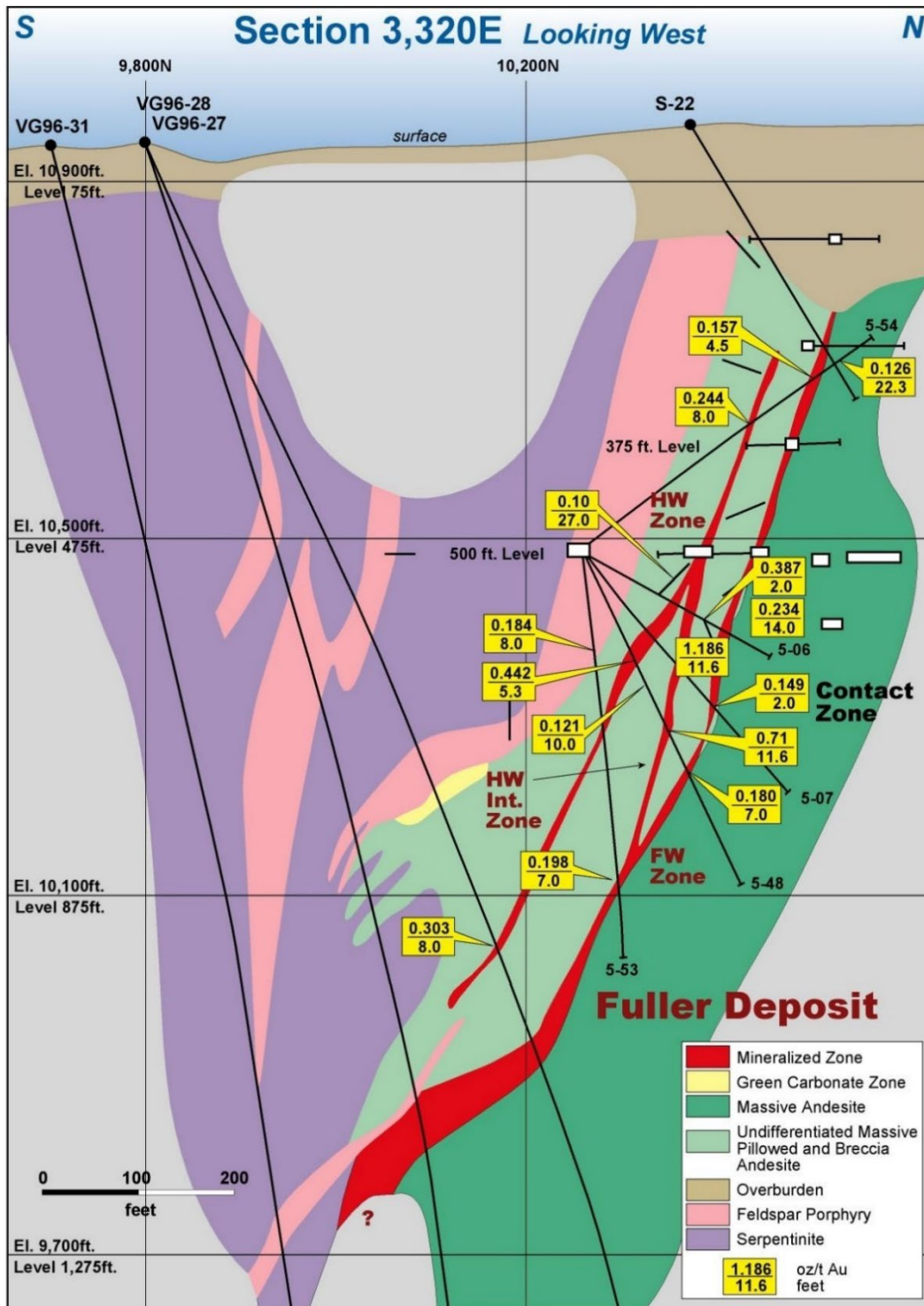
Figure 6-15 Fuller Section 3,320E Looking West (prepared by McEwen, dated 2011)
