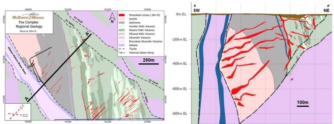
Figure 6-12 Grey Fox Area Schematic Geological Plan Map (left) and Northwest-Looking Cross-Section (right) (prepared by McEwen, dated 2024)
