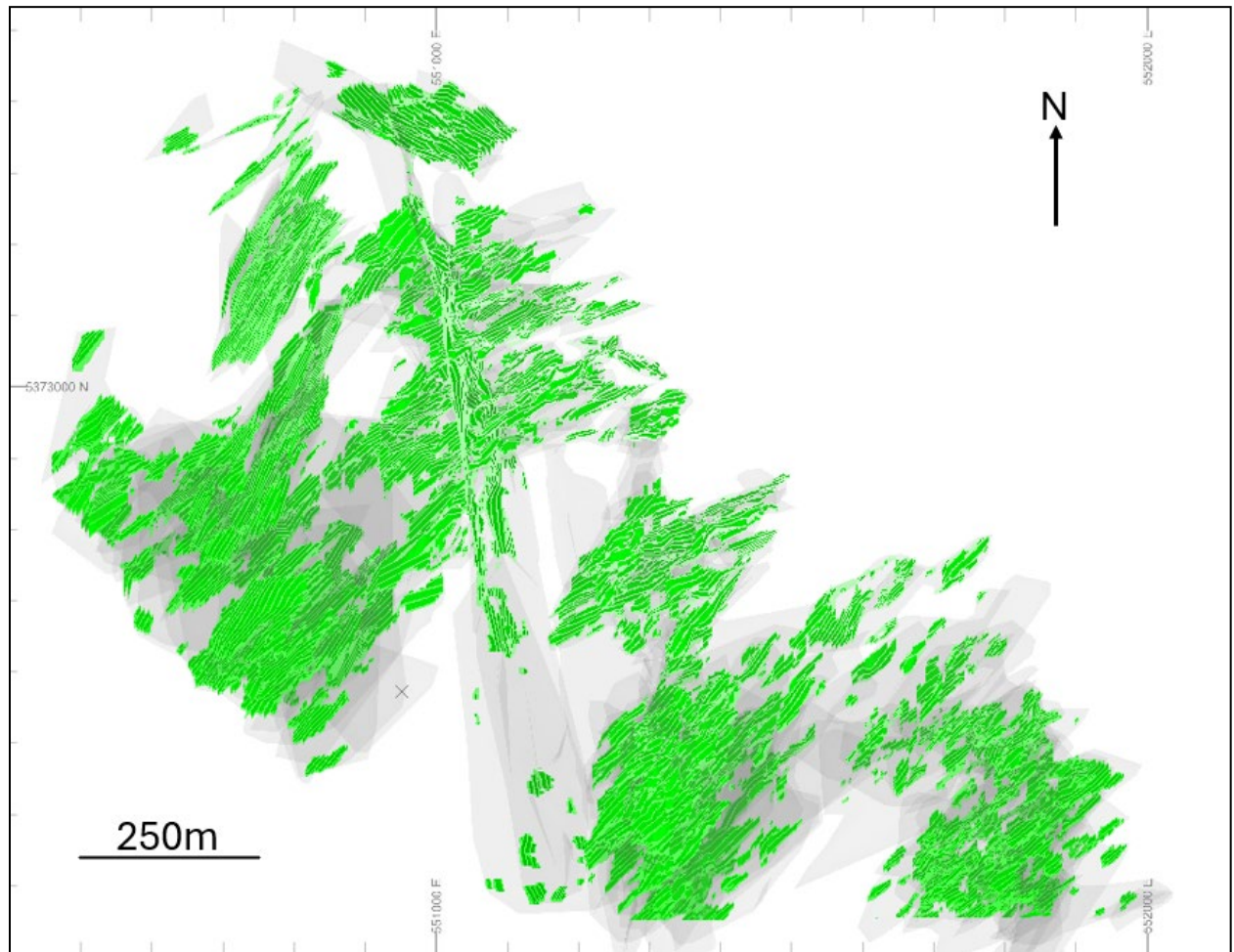
Figure 11-10 Plan View of the Potentially Mineable Stope Shapes at Grey Fox (prepared by McEwen, dated 2024)
