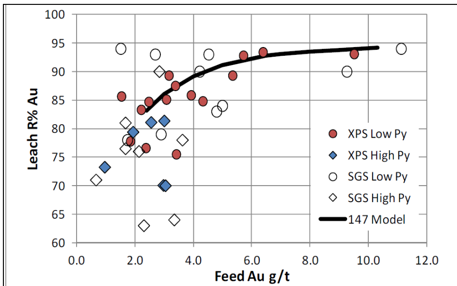
Figure 10-1: Grey Fox Combined Lab Gold Recoveries (XPS, 2014)
