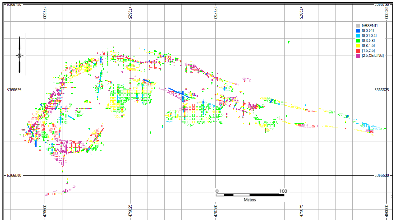
Figure 11-20 Plan View at the 1230 elevation Comparing Block Grades with Drill Hole Data (dots) (prepared by SRK 2021; reissued McEwen 2024)
