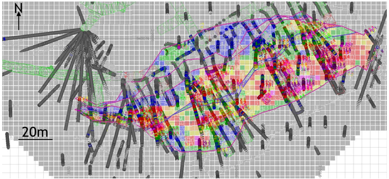
Figure 11-4 Plan View at Elevation 9830 Comparing Block Grades with Drill Hole Data in Froome Domains 300-301 (prepared by McEwen, dated 2024)
