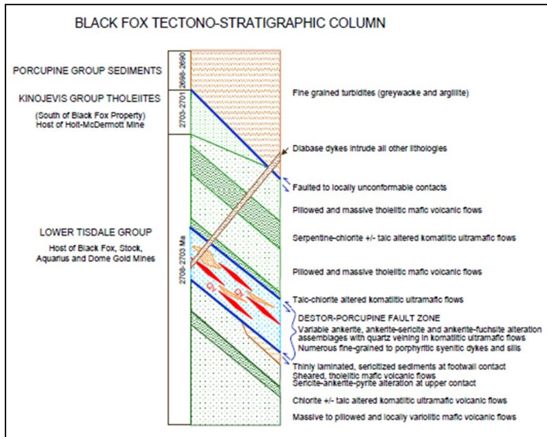
Figure 6-6 Stratigraphic Column for the General Black Fox – Hislop Area (modified after Berentsen et al., 2004)
