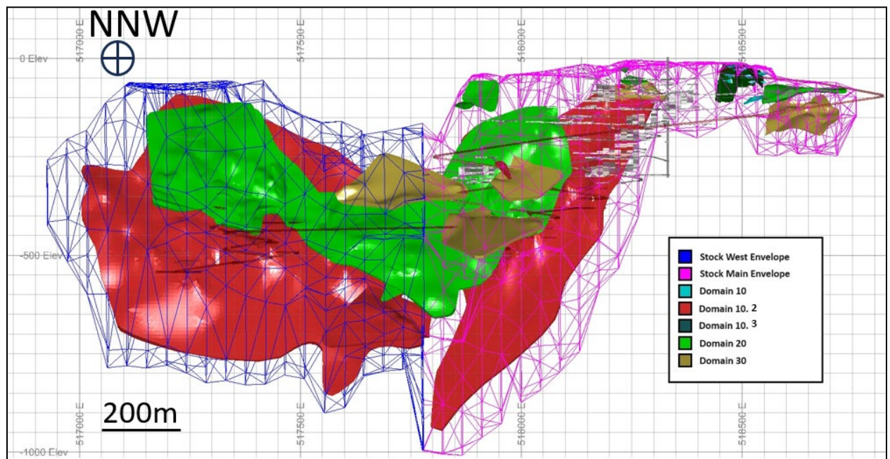
Figure 11-12 Long section of the Stock West & Main Mineralized Zones and Background Envelope (prepared by McEwen, dated 2023)
