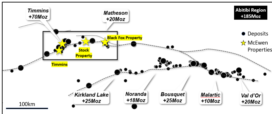
Figure 6-1 Schematic Map of the Abitibi Greenstone Belt showing Relationship of Gold Deposition to Major Structural Conduits (prepared by McEwen, dated 2021)
