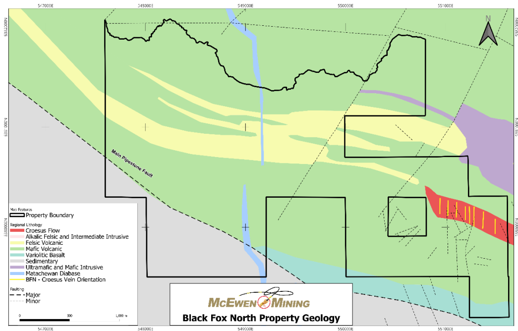
Figure 6-8 Bedrock Geology of the Black Fox North with the possible locations of 'Croesus-like' veins.
