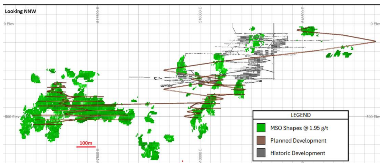
Figure 14-15 Plan View of the Potentially Mineable Stope Shapes at Stock West & Main (prepared by McEwen, dated 2023)
