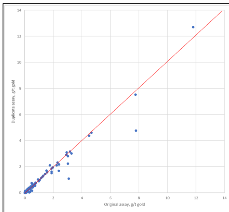
Figure 12-5: Original Assays Against Duplicates for Grey Fox / Gibson for the period 2017 to Current Exploration Period (prepared by McEwen, dated 2021 reissued 2024)
