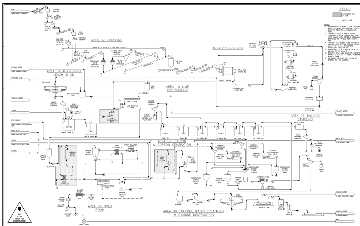
Figure 17-1 Stock Mill Basic Process Flowsheet
