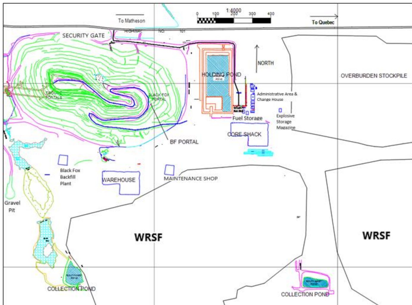
Figure 18-1 Black Fox Site Layout
