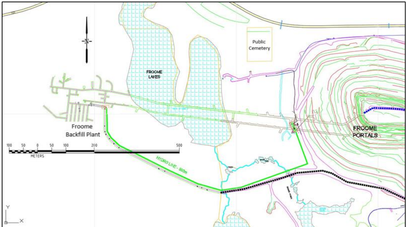
Figure 18-2 Froome Site Layout
