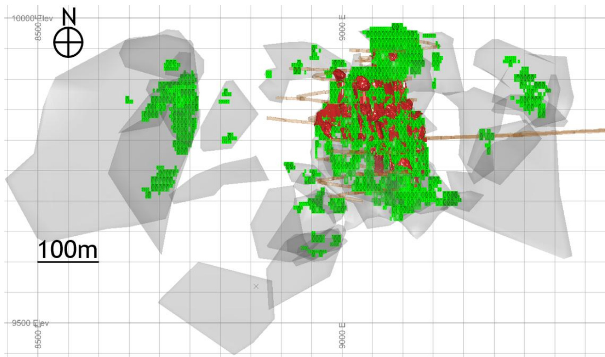
Figure 14-5 Long Section Looking North of the Potentially Mineable Stope Shapes at Froome (prepared by McEwen, dated 2024)
