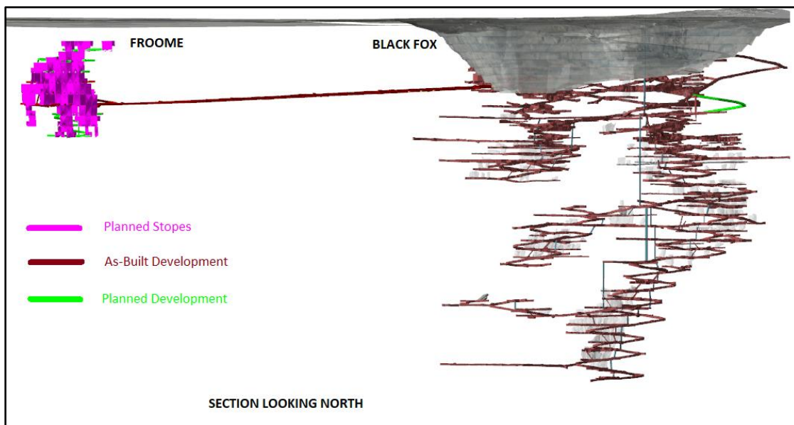
Figure 16-1 Black Fox and Froome Long Section Looking North
