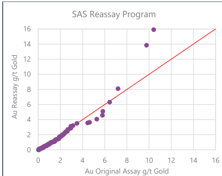
Figure 12-10 Original Assay Data Against Re-assay Data for the St Andrew(SAS) Core Used (prepared by McEwen, dated 2021-reissued 2024)
