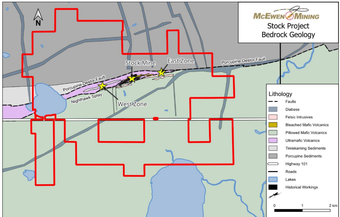
Figure 7-7 Interpreted Geology of the Stock Property and Locations of the Significant Gold Mineralized Zones (yellow stars) (prepared by McEwen, dated 2024)
