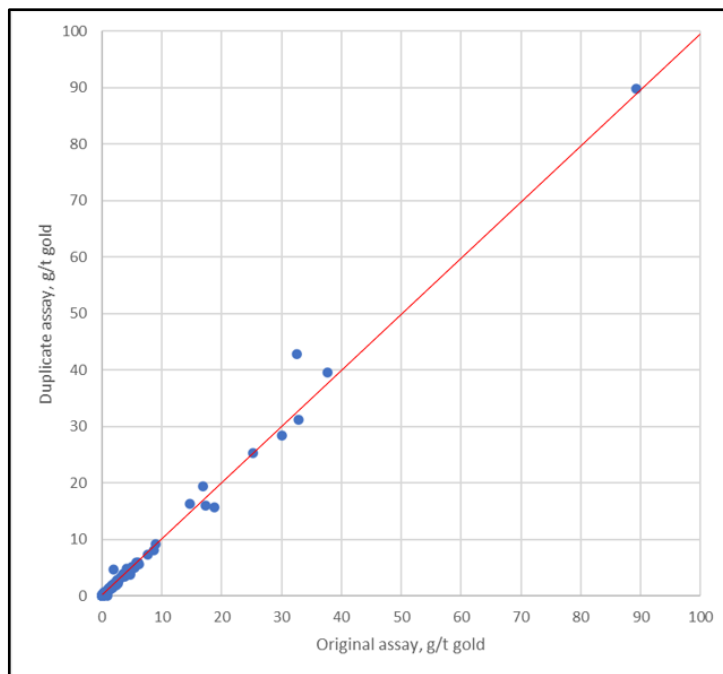
Figure 12-1 Original Assays Against Duplicates at Black Fox for the period 2017 to Current Exploration Period (prepared by McEwen, dated 2021 reissued 2024)
