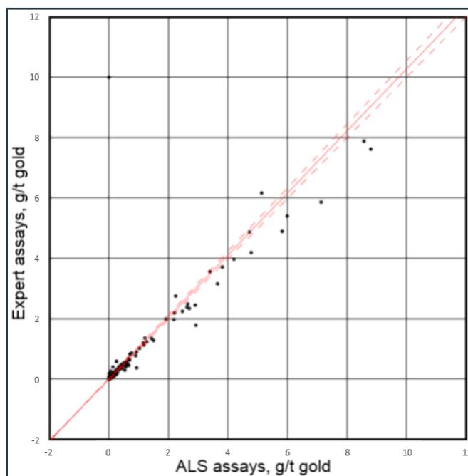
Figure 1212-12 ALS Data Against Expert check Data for the 2009 to 2012 Exploration Period (prepared by SRK 2018; resissued by McEwen 2024)-
