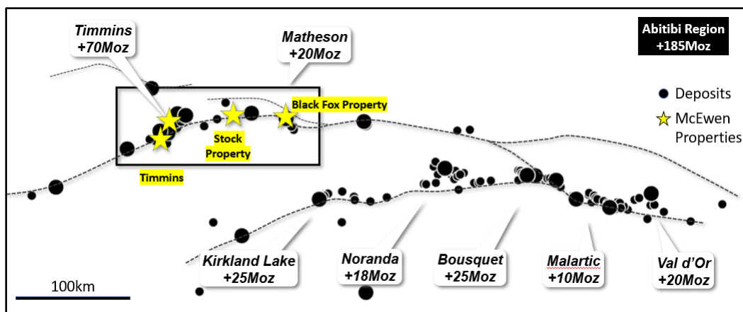
Figure 8-1 Schematic Map of the Abitibi Greenstone Belt showing Relationship of Gold Deposition to Major Structural Conduits (prepared by McEwen, dated 2021)
