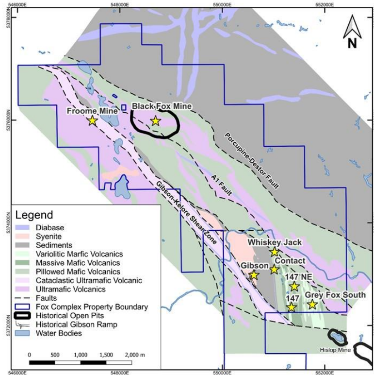
Figure 7-5 Bedrock Geology of the Eastern Properties and Locations of the Significant Gold Mineralized Zones (prepared by McEwen, dated 2024)
