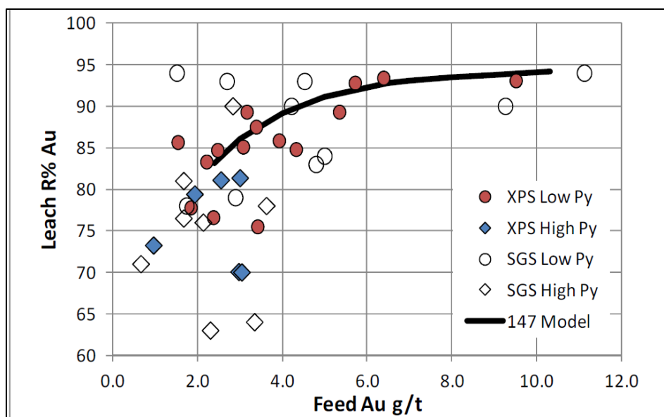
Figure 13-1: Grey Fox Combined Lab Gold Recoveries (XPS, 2014)
