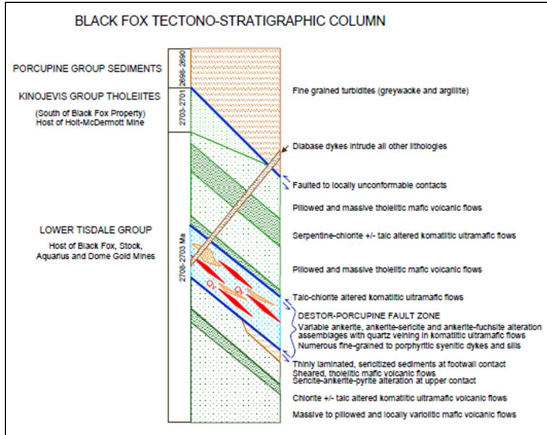
Figure 7-4 Stratigraphic Column for the General Black Fox – Hislop Area (modified after Berentsen et al., 2004)
