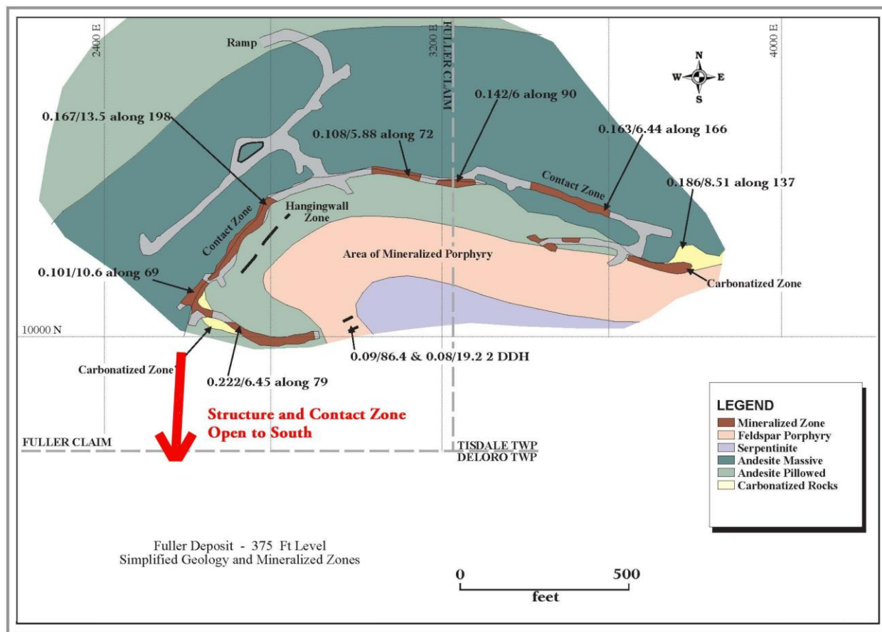
Figure 7-12 Fuller Deposit 375 Level Simplified Geology and Mineralized Zones ( dated 1999; re-issued by McEwen in 2024). NOTE: All values are in oz/t and feet.
