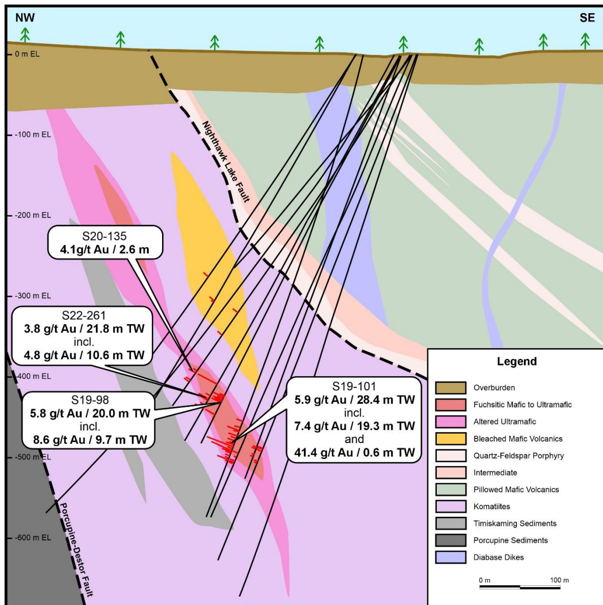
Figure 7-11 Exploration Drilling at Stock West – Schematic Cross-Section Looking to Northeast (prepared by McEwen, dated 2024)
