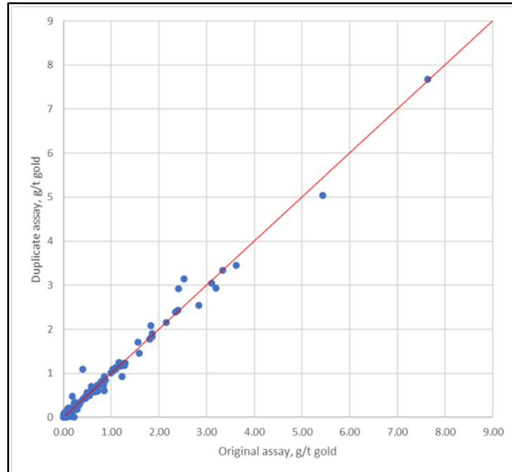
Figure 12-3: Original Assays Against Duplicates at Froome for the period 2017 to Current Exploration Period (prepared by McEwen, dated 2021 reissued 2024)
