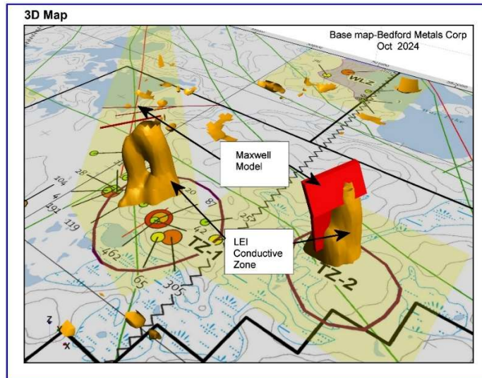
Figure 1: 3D view of VTEM LEI and Maxwell modeling for TZ-1 and TZ-2. (base map from Bedford Metals Corp. Oct 2024)
