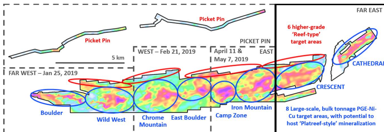
Figure 1 – Fourteen Target Areas Across the 25-Kilometer Length of the Stillwater West Project
