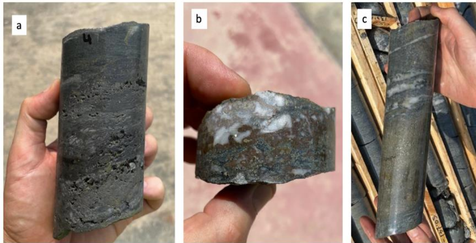
(a) potential high-grade chalcocite at 57m down-hole depth, (b) coarse cassiterite at 134m, and (c) massive sulphide at 139m
