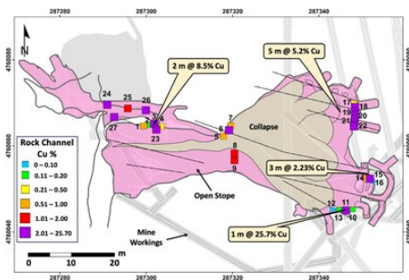
Figure 2 – Plan view of Profunda mine workings and La Cueva open stop and new channel sample locations, within a depth slice from 1425m to 1485m elevation. (CNW Group/Pan Global Resources Inc.)
