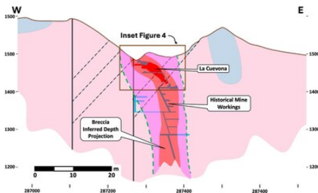
Figure 3 – East-West section projection of the Profunda Breccia and Historical Mine workings (extend from surface to ~260m vertical depth), and Figure 4 location. (CNW Group/Pan Global Resources Inc.)
