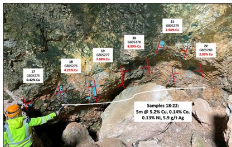
Figure 5 – Profunda rock chip channel sample results (samples 17 to 22) (CNW Group/Pan Global Resources Inc.)
