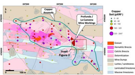
Figure 1 – Profunda Target - geology and alteration map showing the location of the La Cuevona mine workings (Figure 2) and portable XRF (pXRF) soil copper anomaly. (CNW Group/Pan Global Resources Inc.)
