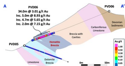
Figure 2 –Geology cross-section for drillholes PVD05 and PVD06 (CNW Group/Pan Global Resources Inc.)
