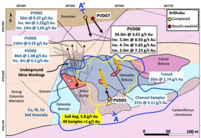
Figure 1 – Summary Geology map and drillhole locations; A – A' cross section location (CNW Group/Pan Global Resources Inc.)
