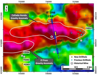
Figure 2 – Cañada Honda and El Pozo gravity anomalies showing SQUID IP and AMT anomalies and drillhole locations (see Figure 3) (CNW Group/Pan Global Resources Inc.)
