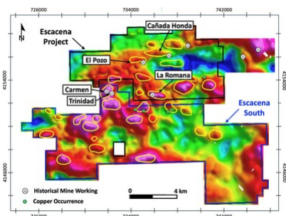
Figure 1 &#8211; Escacena Project gravity anomaly map showing Cañada Honda, La Romana, Escacena South (expanded) and priority exploration targets (CNW Group/Pan Global Resources Inc.)
