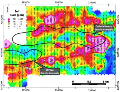
Figure 4 – Soil gold geochemistry and priority target areas across the Cañada Honda and El Pozo corridor (CNW Group/Pan Global Resources Inc.)
