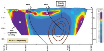
Figure 3 – SQUID IP cross-section (Line CH4) highlighting high chargeability drill targets adjacent to the gravity anomaly (CNW Group/Pan Global Resources Inc.)
