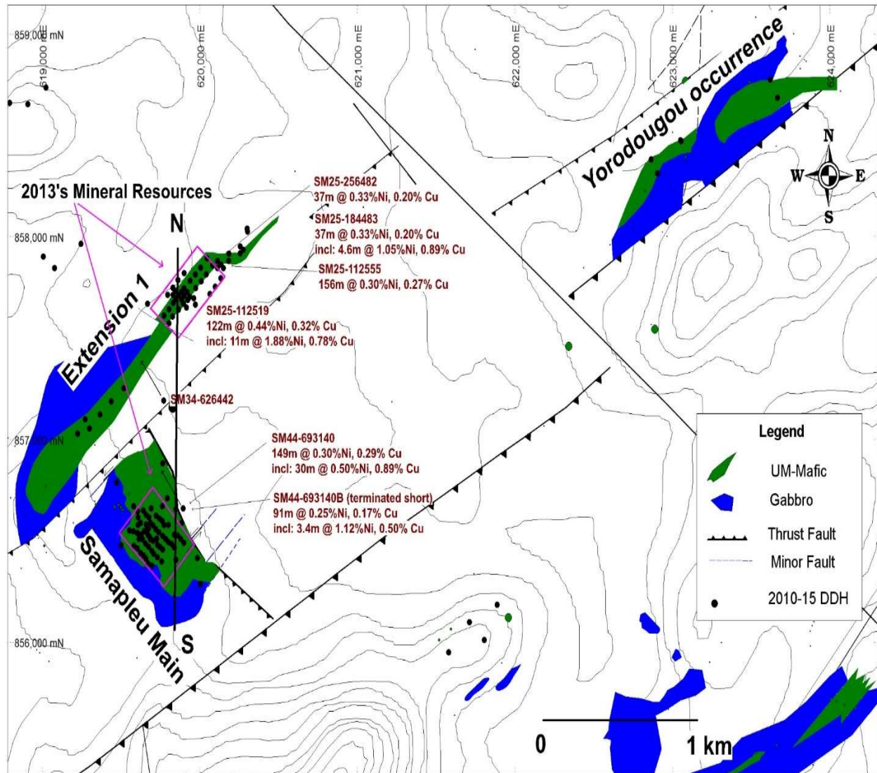
Figure 3: Samapleu Main and Extension 1 deposits together with Yorodougou occurrence.
