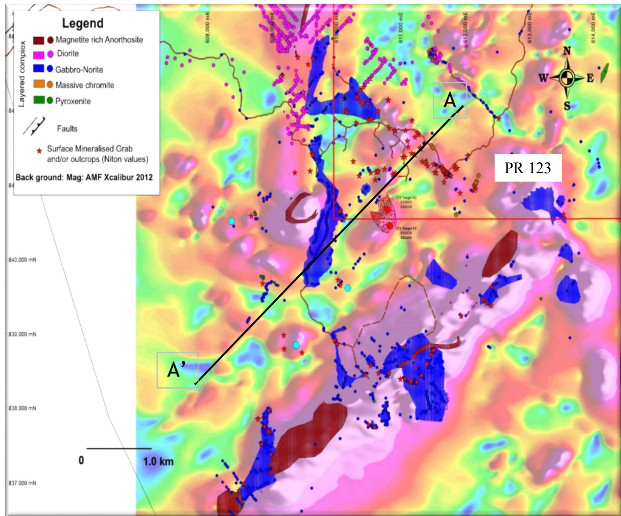
Figure 4: Surface geology and deep target at Yepleu/Zérégouiné (PR 123 - PR 300), cross-section A-A' shown at figure 5.
