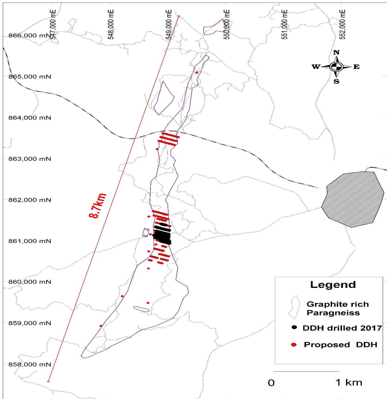
Figure 2: Lola Graphite deposit showing the 2017 drilling program with completed DDH at May 14, 2017.
