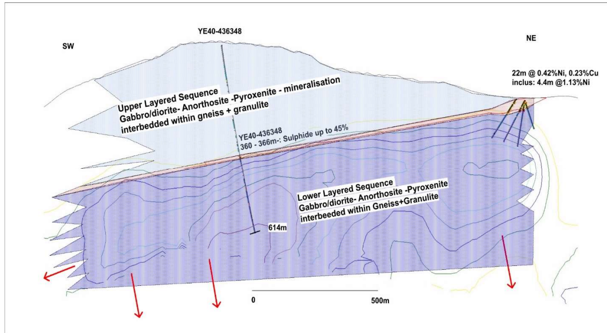
Figure 5: Cross-section at Yepleu showing hole YE40-436348 terminated short of the target for a technical reason. A mineralised horizon of 6.65 m grading 0.30% nickel and 0.26% copper, including 0.55 m at 0.90% nickel and 0.80% copper was intercepted at the interface between two layer assemblages.
