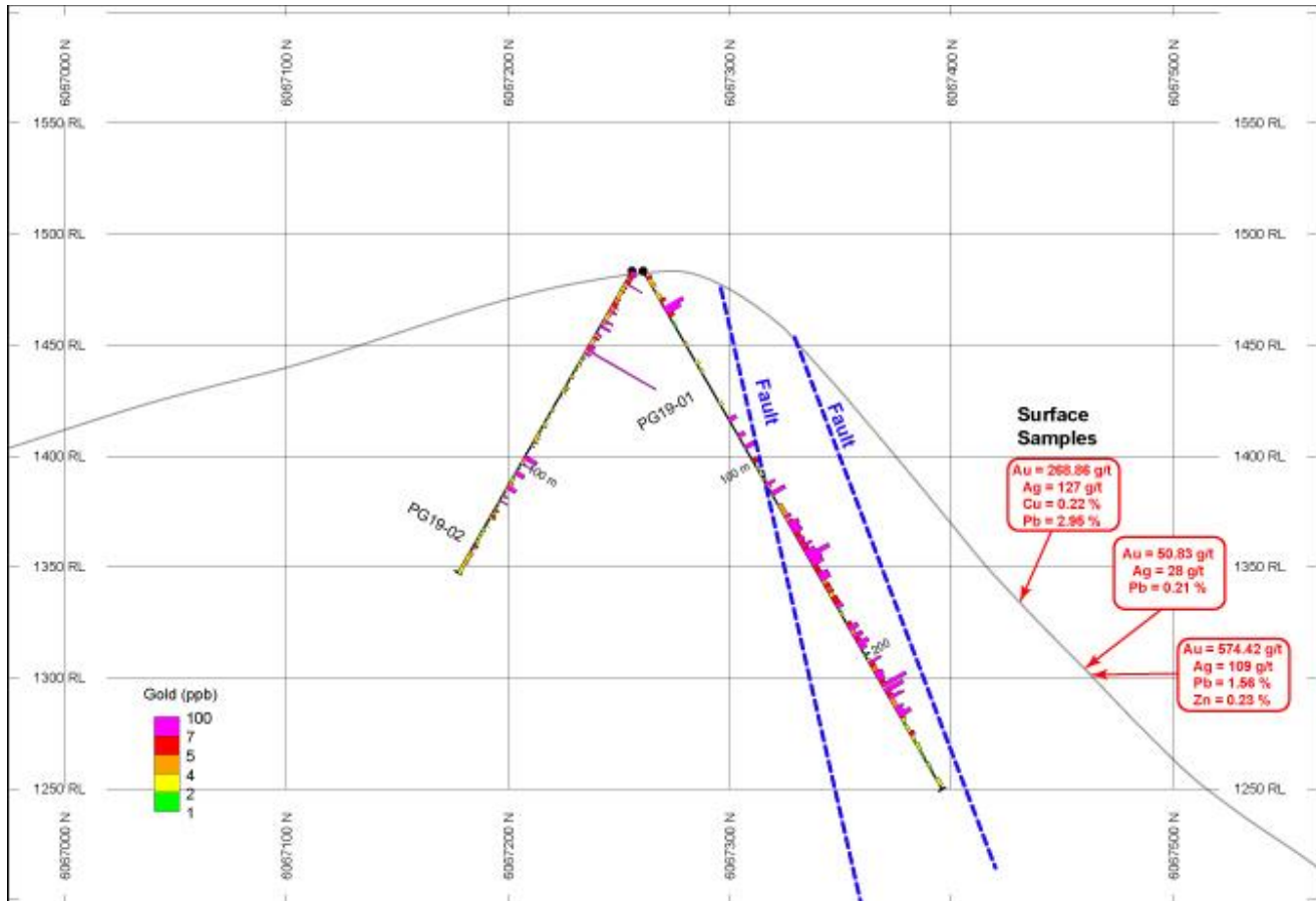
Figure 2: Vertical Section with Drill Holes and Fault (Projected)
