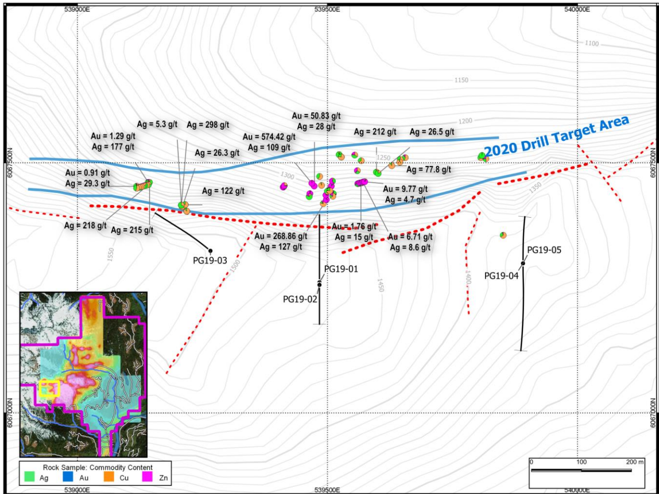
Figure 1 : Paddy Mac Drill Plan
